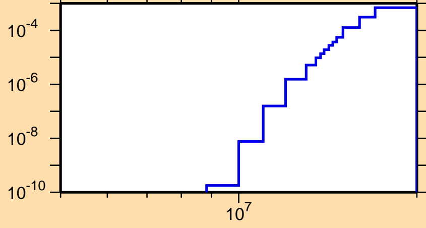
\sigma vs. E for ^{252}\text{Fm}(n,t)
