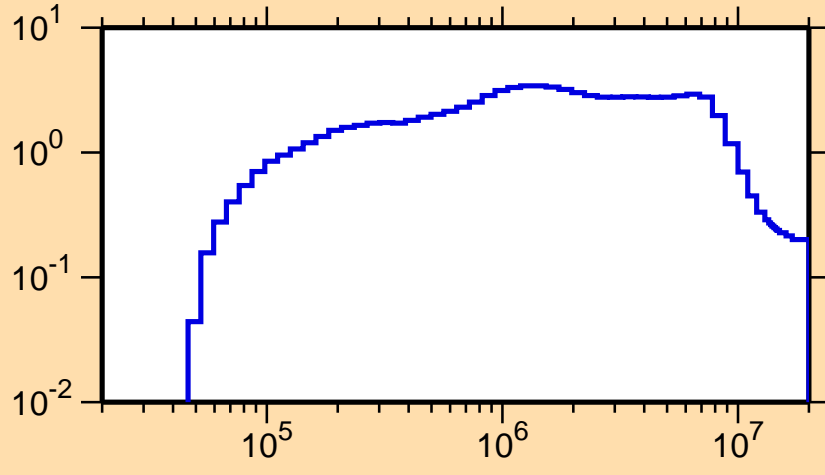
\sigma vs. E for ^{252}\text{Fm}(n,\text{inel.})
