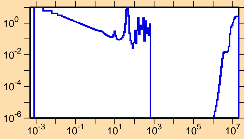
\sigma vs. E for ^{252}\text{Fm}(n,f)
