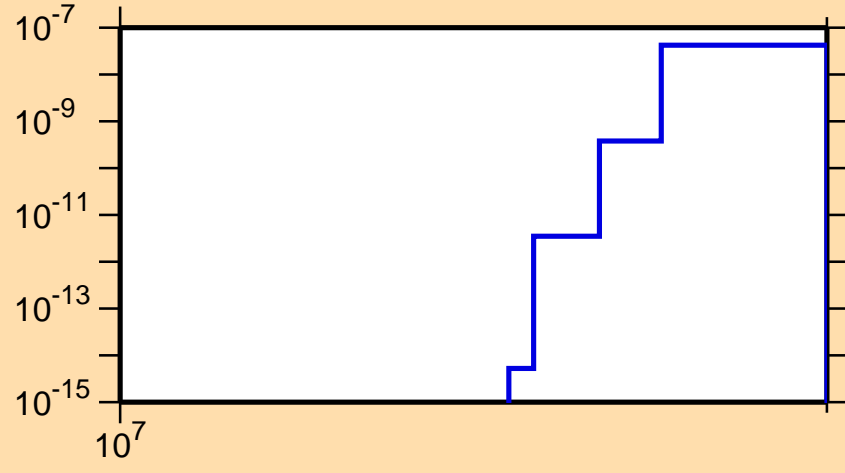
\sigma vs. E for ^{252}\text{Fm}(n,2np)
