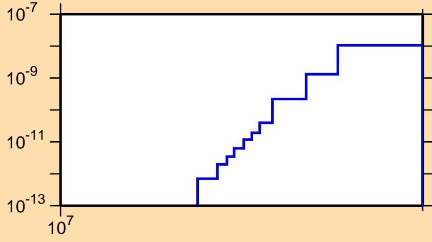
\sigma vs. E for ^{252}\text{Fm}(n,\text{He3})
