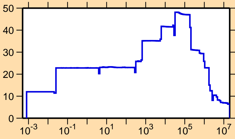
\Delta\sigma/\sigma vs. E for ^{252}\text{Fm}(n,\text{nonel.})
