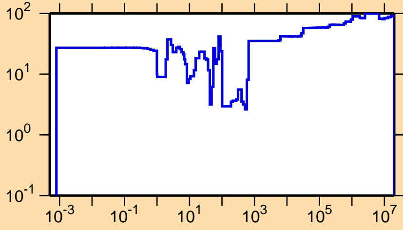
\Delta\sigma/\sigma vs. E for ^{252}\text{Fm}(n,\gamma)
