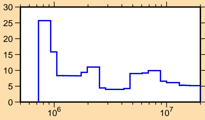
\Delta\sigma/\sigma vs. E for ^{252}\text{Fm}(n,tot.)
