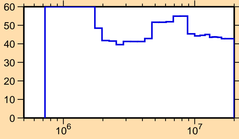
\Delta\sigma/\sigma vs. E for ^{252}\text{Fm}(n,n\text{cont.})
