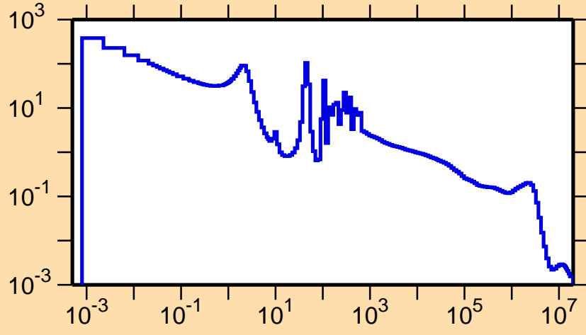
\sigma vs. E for ^{252}\text{Fm}(n,\gamma)
