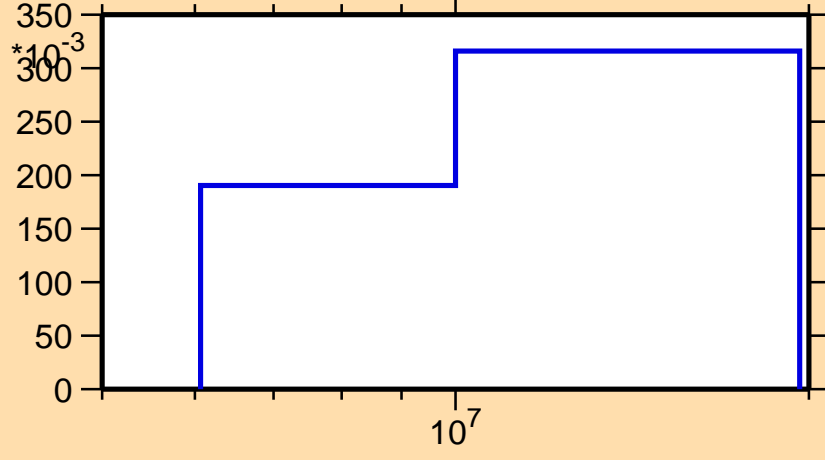
\sigma vs. E for ^{252}\text{Fm}(n,2n)
