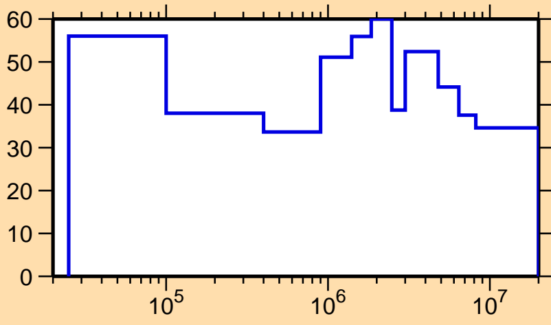
\Delta\sigma/\sigma vs. E for ^{252}\text{Fm}(n,n_1)
