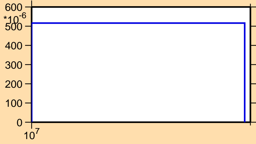
\sigma vs. E for ^{253}\text{Fm}(n,3n)
