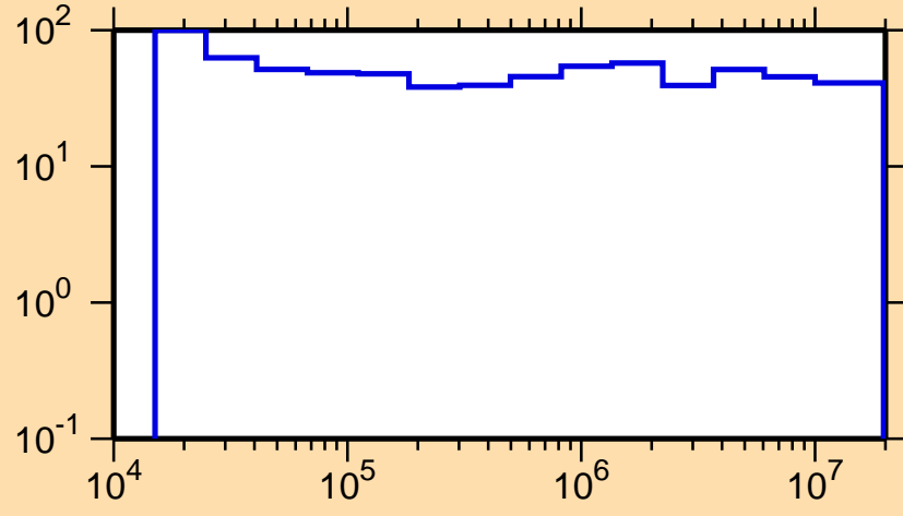
\Delta\sigma/\sigma vs. E for ^{253}\text{Fm}(n,n_1)
