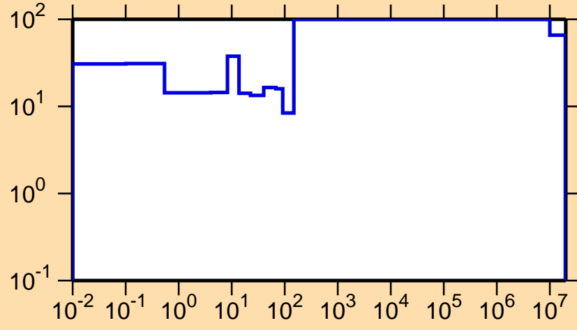
\Delta\sigma/\sigma vs. E for ^{253}\text{Fm}(n,f)
