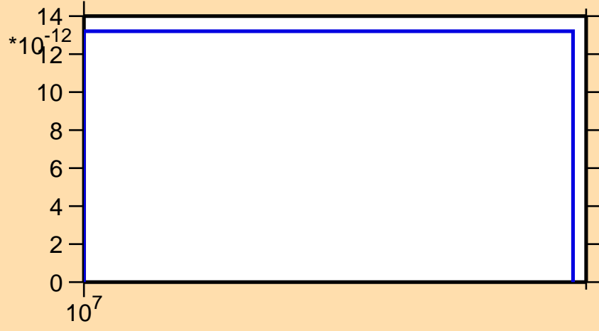
\sigma vs. E for ^{253}\text{Fm}(n,p\alpha)
