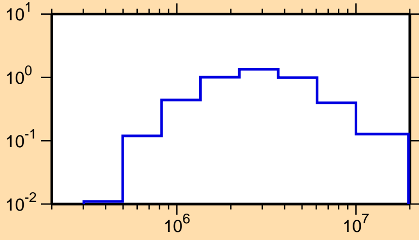
\sigma vs. E for ^{253}\text{Fm}(n,n\text{cont.})
