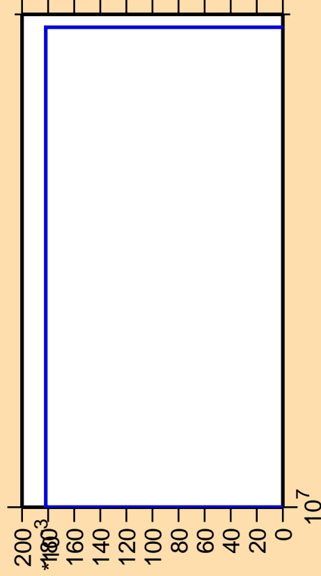
\Delta\sigma/\sigma vs. E for ^{253}\text{Fm} (mt 34)
