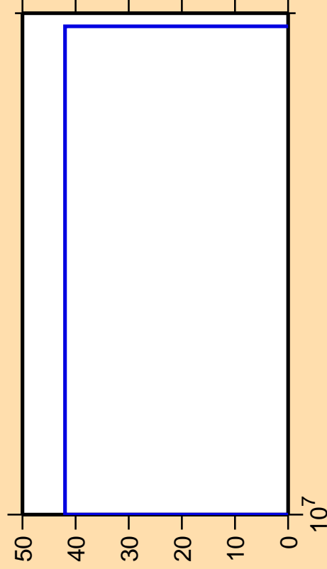
\Delta\sigma/\sigma vs. E for ^{253}\text{Fm}(n,p\alpha)
