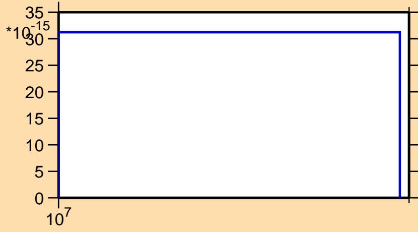
\sigma vs. E for ^{253}\text{Fm} (mt 34)
