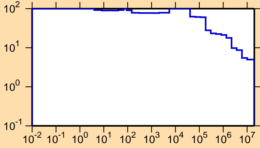
\Delta\sigma/\sigma vs. E for ^{253}\text{Fm}(n,\text{nonel.})
