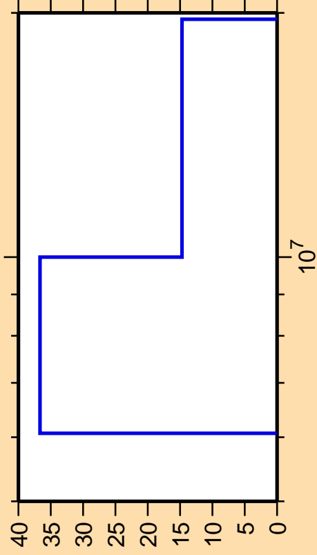
\Delta\sigma/\sigma vs. E for ^{253}\text{Fm}(n,t)
