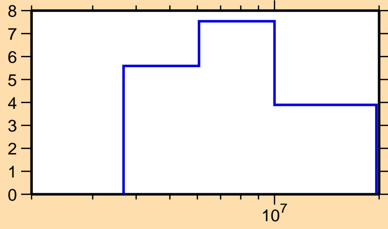
\Delta\sigma/\sigma vs. E for ^{253}\text{Fm}(n,\text{tot.})
