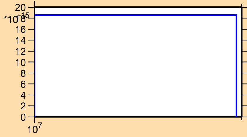
\sigma vs. E for ^{253}\text{Fm}(n,3n\alpha)
