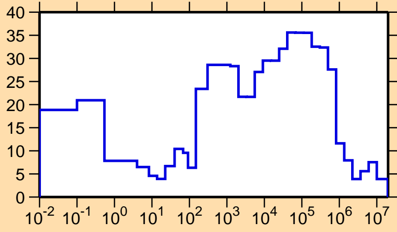
\Delta\sigma/\sigma vs. E for ^{253}\text{Fm}(n,\text{tot.})
