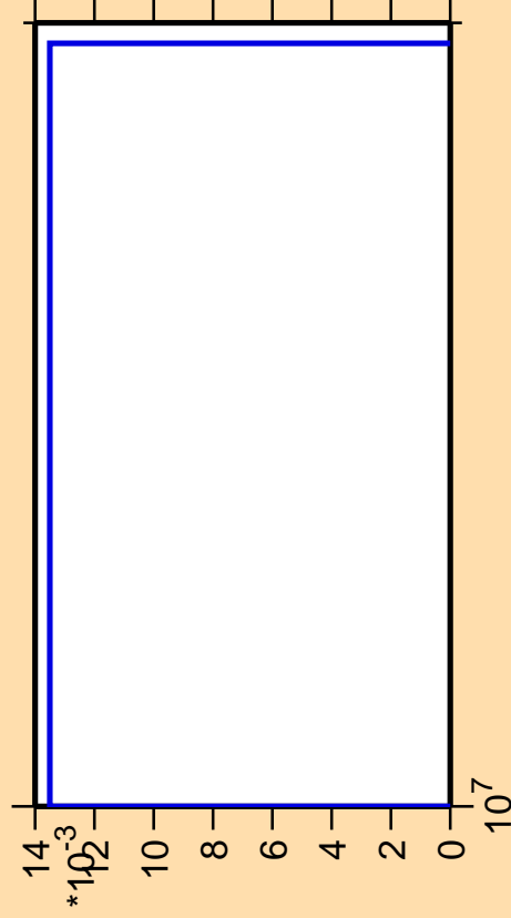
\Delta\sigma/\sigma vs. E for ^{253}\text{Fm}(n,3n\alpha)
