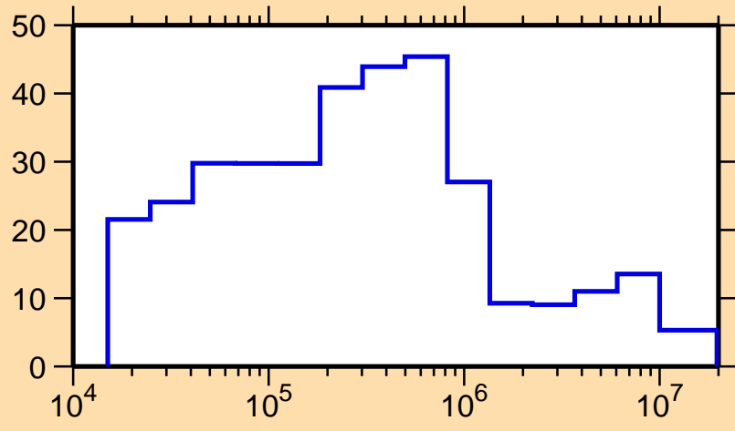
\Delta\sigma/\sigma vs. E for ^{253}\text{Fm}(n,\text{el.})
