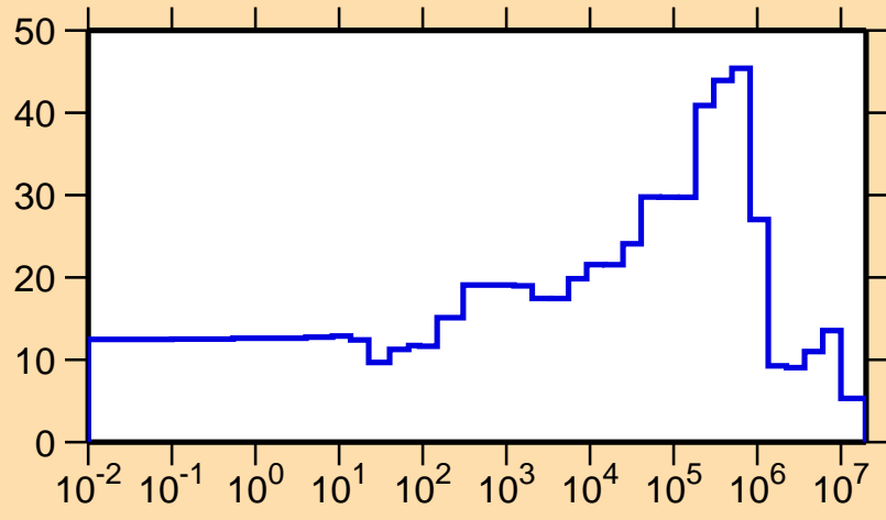
\Delta\sigma/\sigma vs. E for ^{253}\text{Fm}(n,el.)
