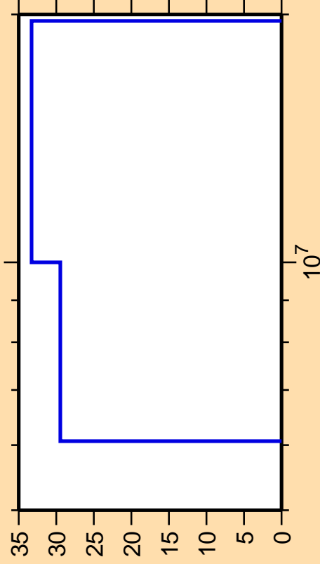
\Delta\sigma/\sigma vs. E for ^{253}\text{Fm}(n,d)
