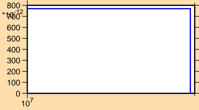
\sigma vs. E for ^{253}\text{Fm}(n,\text{nd})
