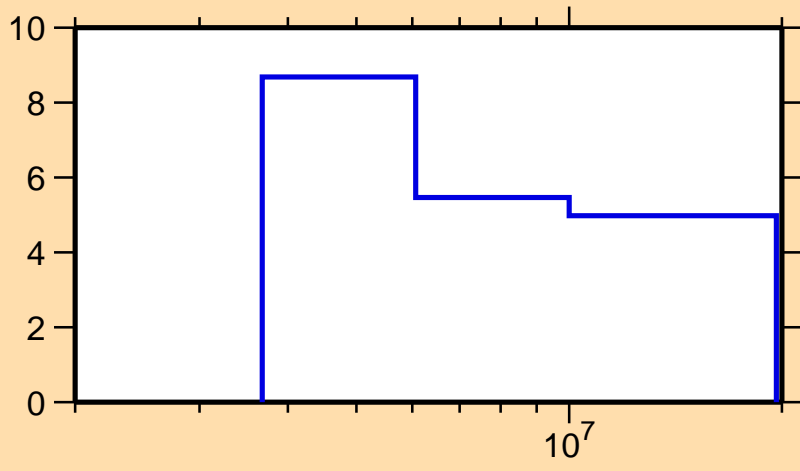
\Delta\sigma/\sigma vs. E for ^{253}\text{Fm}(n,\text{nonel.})
