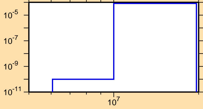
\sigma vs. E for ^{253}\text{Fm}(n,t)
