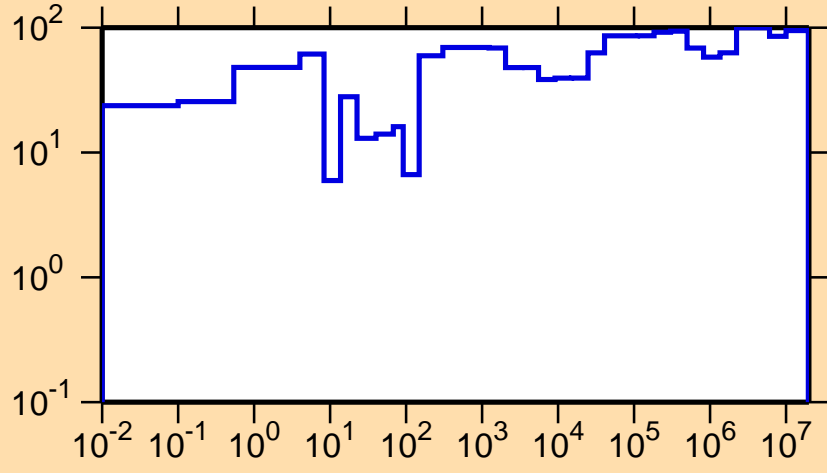
\Delta\sigma/\sigma vs. E for ^{253}\text{Fm}(n,\gamma)
