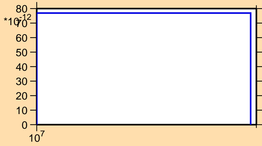
\sigma vs. E for ^{253}\text{Fm}(n,\text{He}3)
