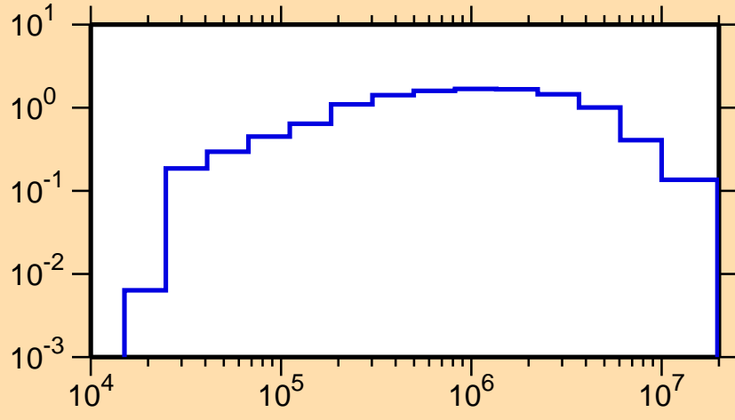
\sigma vs. E for ^{253}\text{Fm}(n,\text{inel.})
