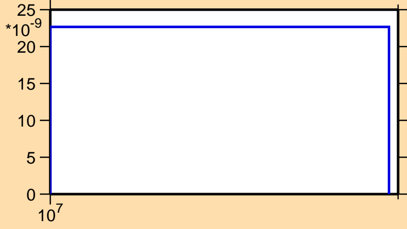
\sigma vs. E for ^{253}\text{Fm}(n,nt)
