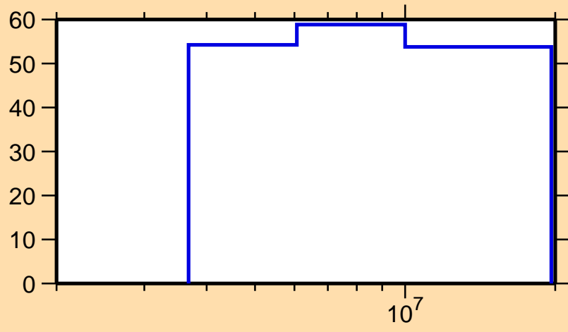
\Delta\sigma/\sigma vs. E for ^{253}\text{Fm}(n,2n)
