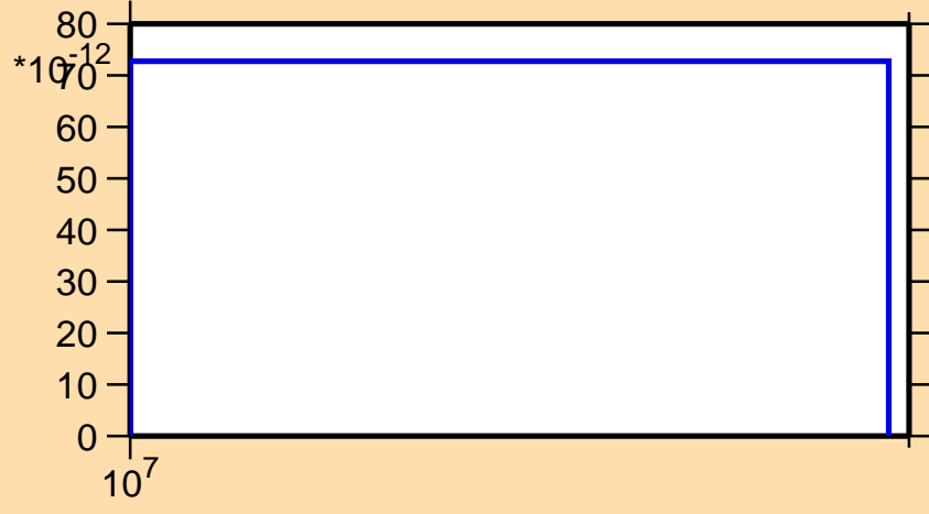
\sigma vs. E for ^{253}\text{Fm}(n,2np)
