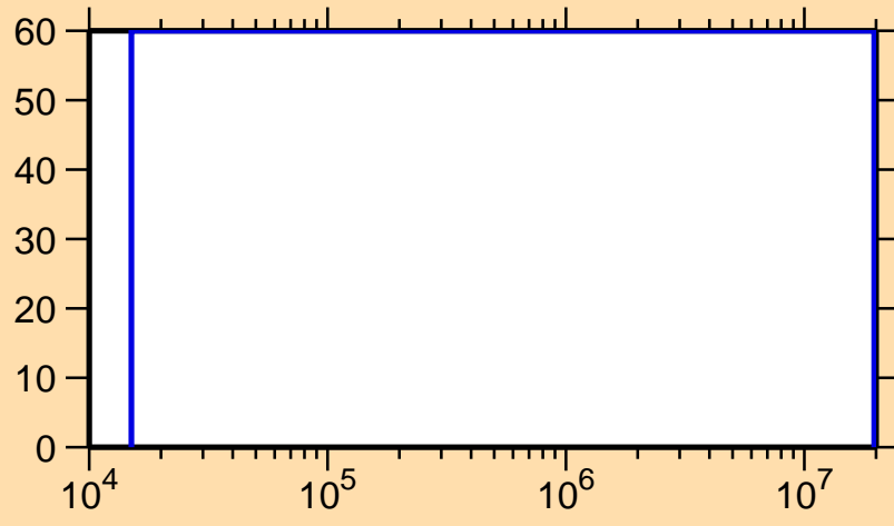
\Delta\sigma/\sigma vs. E for ^{253}\text{Fm}(n,f)
