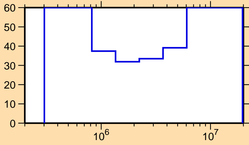
\Delta\sigma/\sigma vs. E for ^{253}\text{Fm}(n,n\text{cont.})
