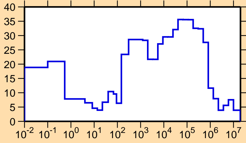
\Delta\sigma/\sigma vs. E for ^{253}\text{Fm}(n,\text{tot.})
