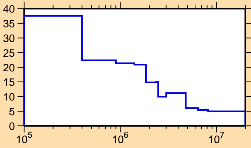
\Delta\sigma/\sigma vs. E for ^{253}\text{Fm}(n,nonel.)
