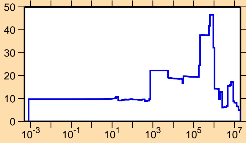
\Delta\sigma/\sigma vs. E for ^{254}\text{Fm}(n,el.)
