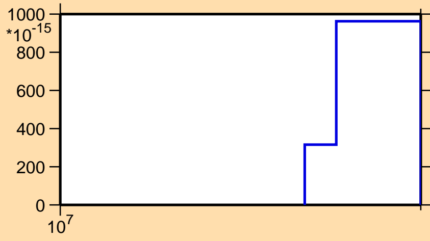
\sigma vs. E for ^{254}\text{Fm}(n,p\alpha)
