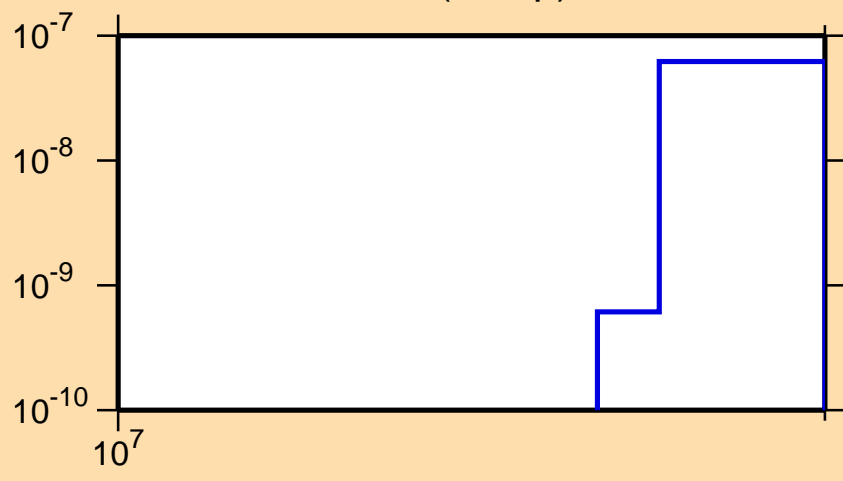
\sigma vs. E for ^{254}\text{Fm}(n,2np)
