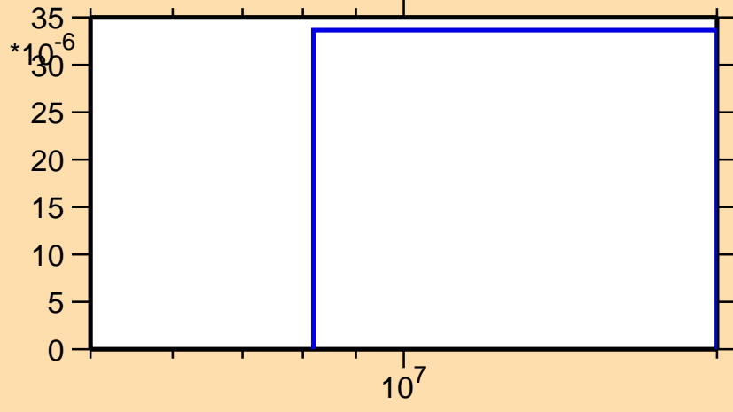
\sigma vs. E for ^{254}\text{Fm}(n,t)
