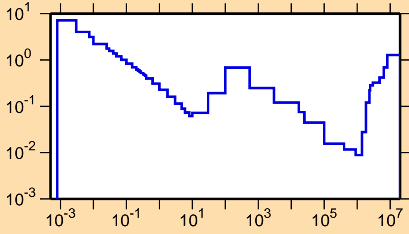
\sigma vs. E for ^{254}\text{Fm}(n,f)
