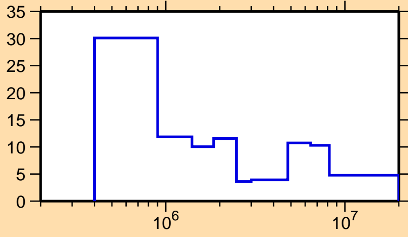
\Delta\sigma/\sigma vs. E for ^{254}\text{Fm}(n, tot.)
