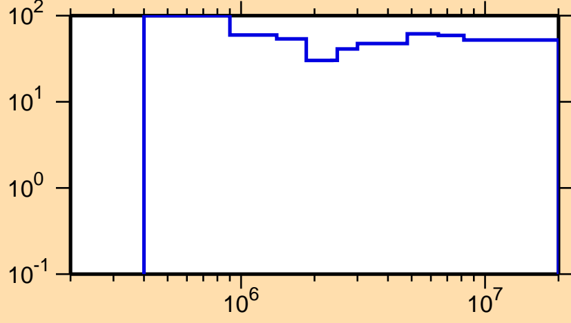
\Delta\sigma/\sigma vs. E for ^{254}\text{Fm}(n,n\text{cont.})
