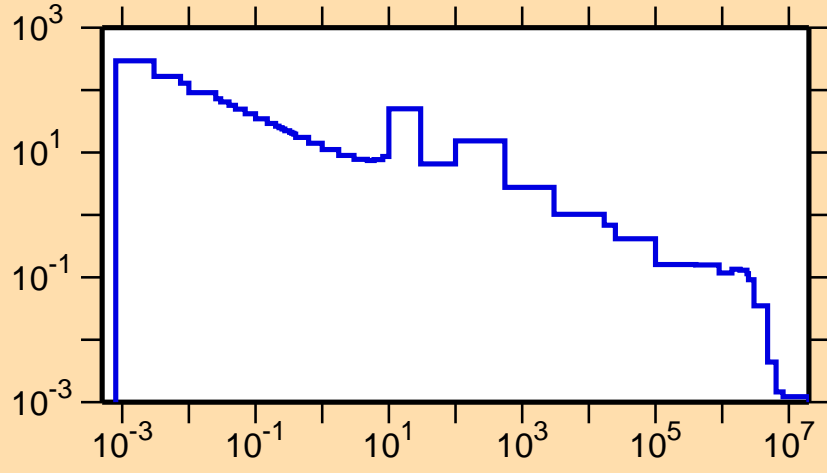
\sigma vs. E for ^{254}\text{Fm}(n,\gamma)
