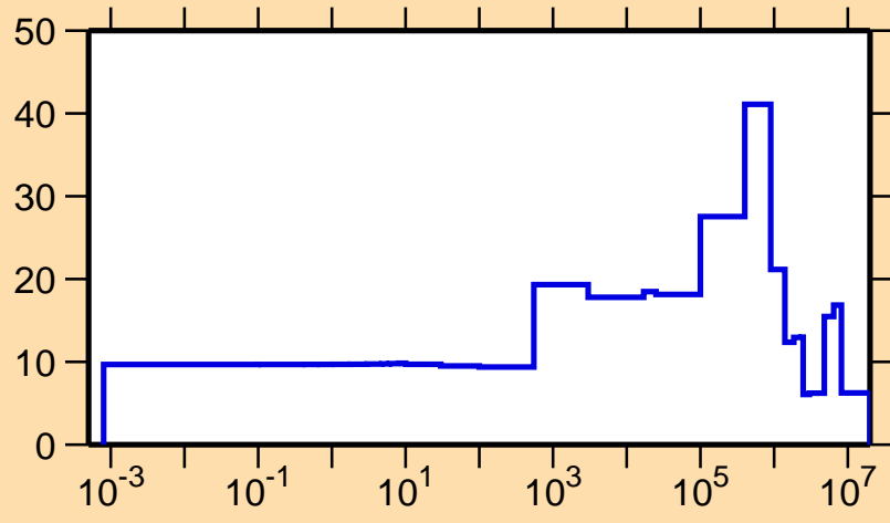
\Delta\sigma/\sigma vs. E for ^{254}\text{Fm}(n,el.)
