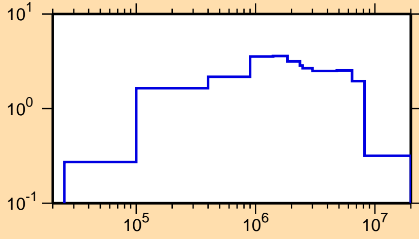
\sigma vs. E for ^{254}\text{Fm}(n,\text{inel.})
