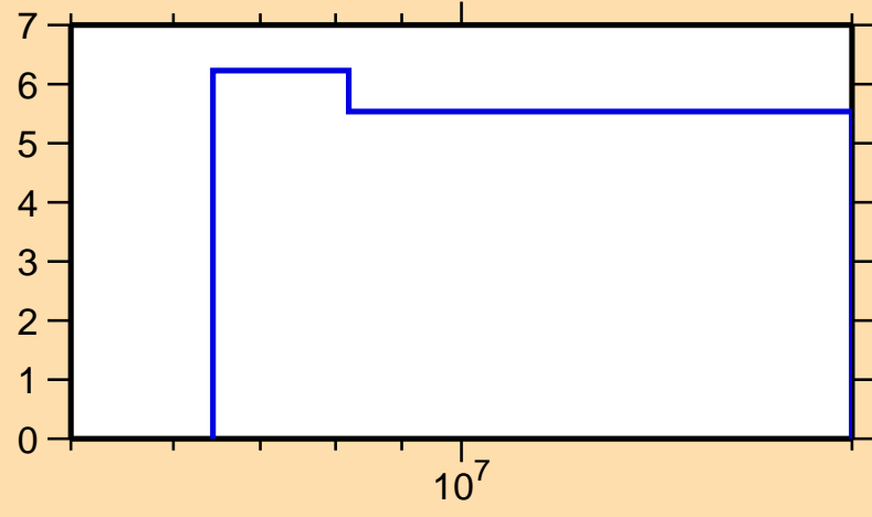
\Delta\sigma/\sigma vs. E for ^{254}\text{Fm}(n,\text{nonel.})
