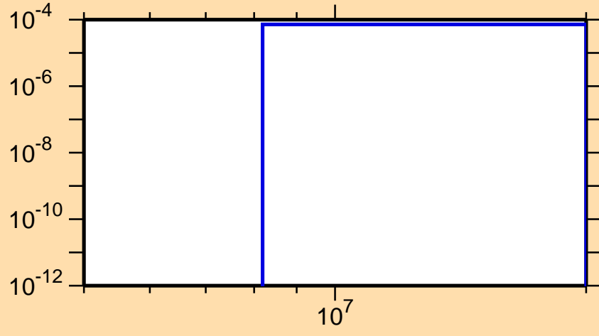
\sigma vs. E for ^{254}\text{Fm}(n,d)
