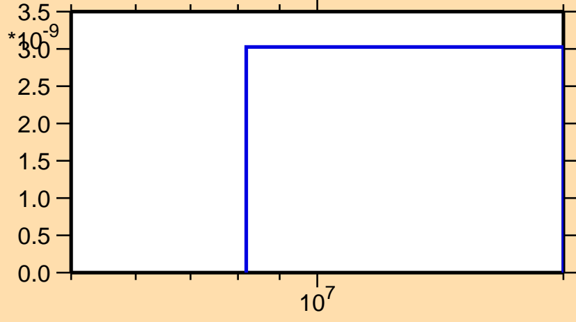
\sigma vs. E for ^{254}\text{Fm}(n,nd)
