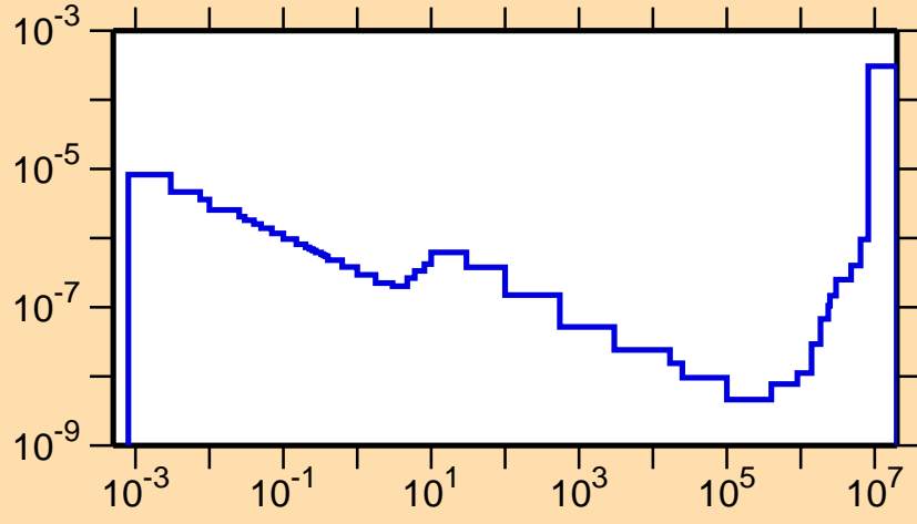
\sigma vs. E for ^{254}\text{Fm}(n,\alpha)
