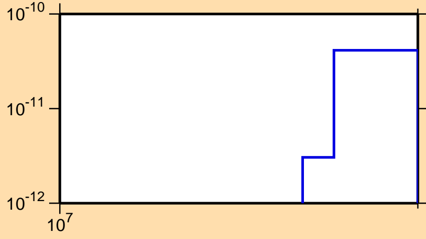
\sigma vs. E for ^{255}\text{Fm}(n,\text{He3})
