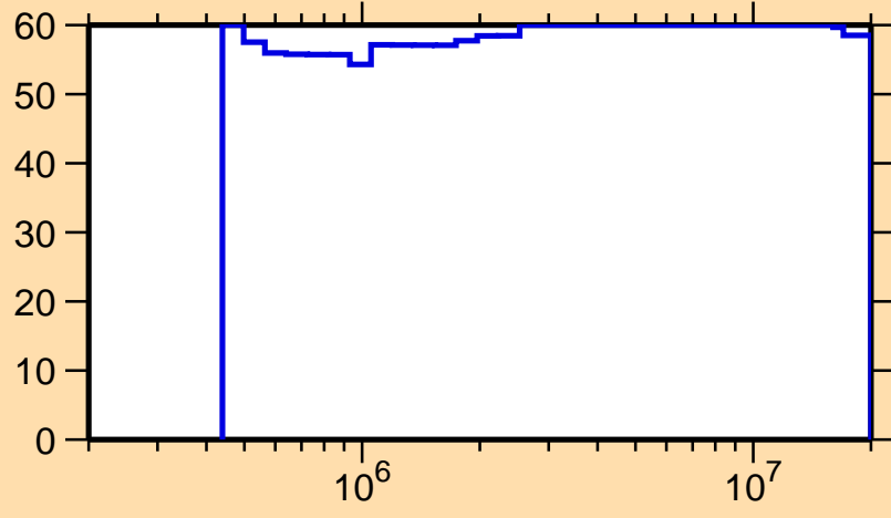
\Delta\sigma/\sigma vs. E for ^{255}\text{Fm}(n,n\text{cont.})
