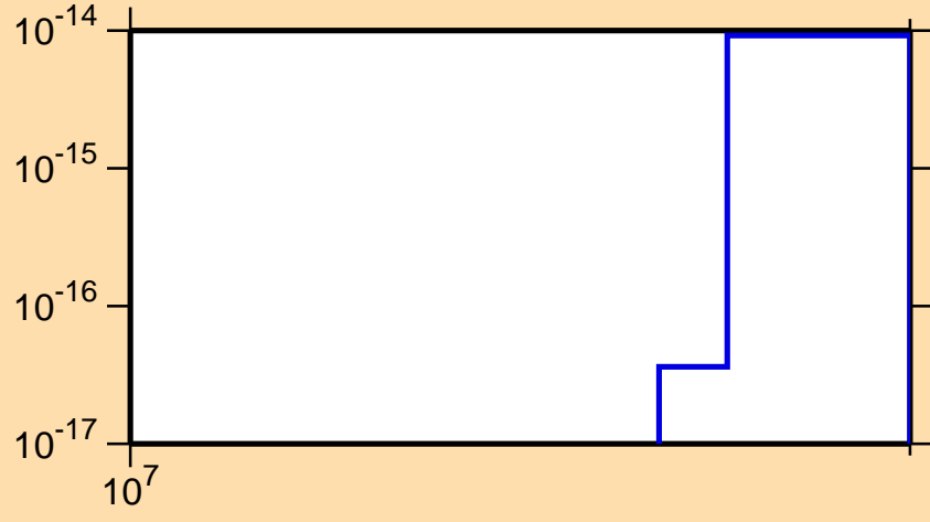
\sigma vs. E for ^{255}\text{Fm} (mt 34)
