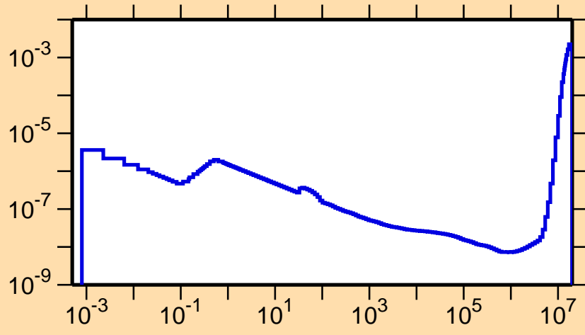
\sigma vs. E for ^{255}\text{Fm}(n,\alpha)
