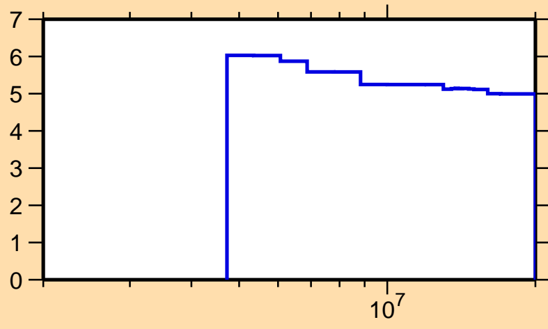
\Delta\sigma/\sigma vs. E for ^{255}\text{Fm}(n,\text{nonel.})
