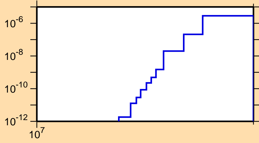
\sigma vs. E for ^{255}\text{Fm}(n,nd)
