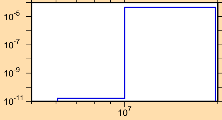
\sigma vs. E for ^{255}\text{Fm}(n,t)
