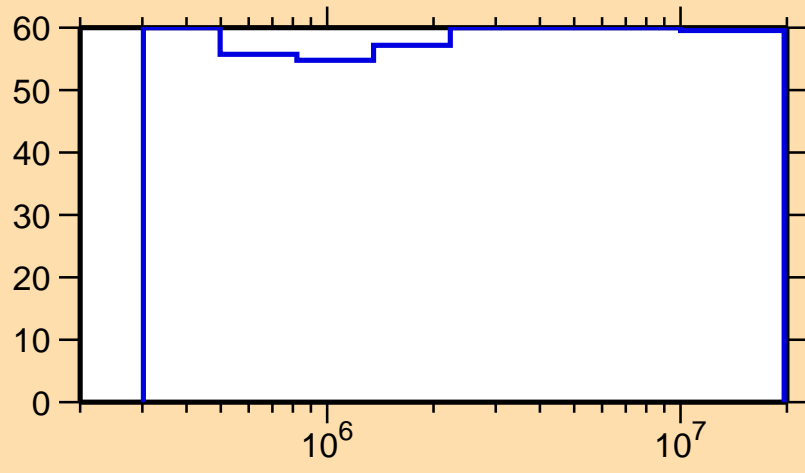
\Delta\sigma/\sigma vs. E for ^{255}\text{Fm}(n,n\text{cont.})
