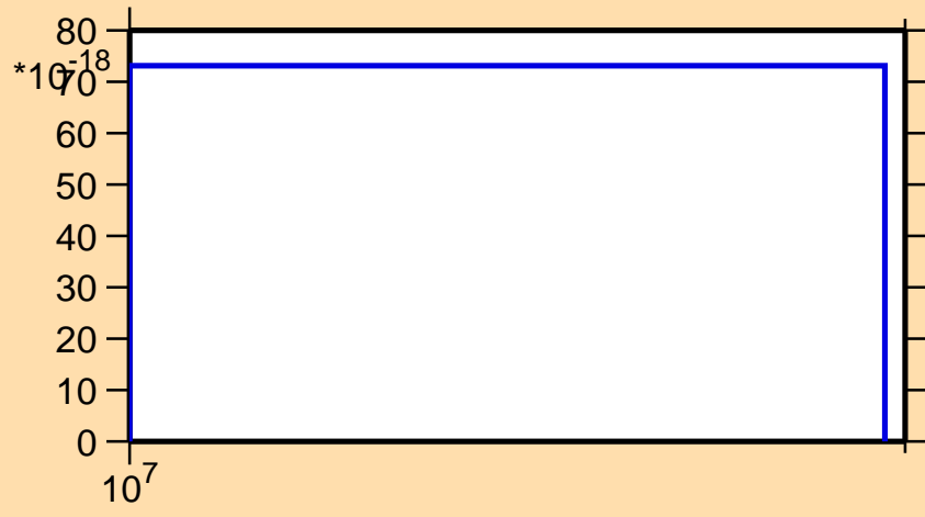
\sigma vs. E for ^{255}\text{Fm} (mt 34)
