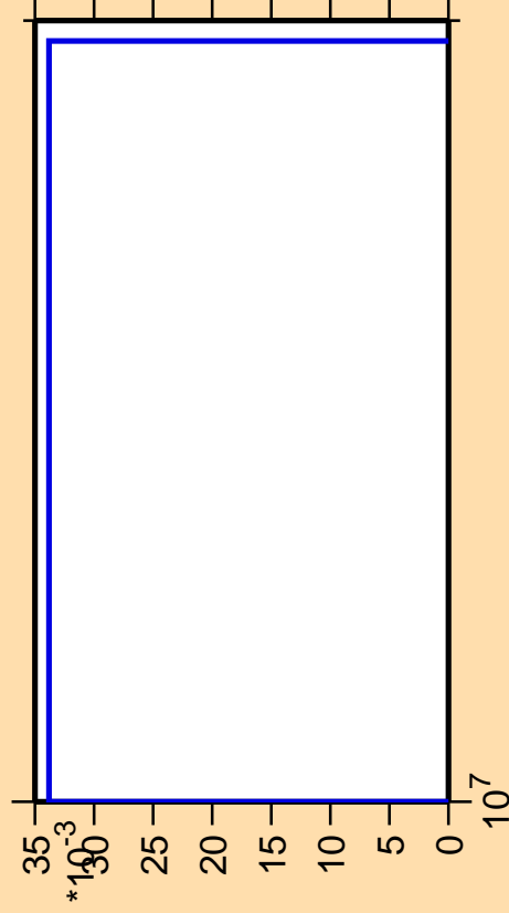
\Delta\sigma/\sigma vs. E for ^{255}\text{Fm}(n,3n\alpha)
