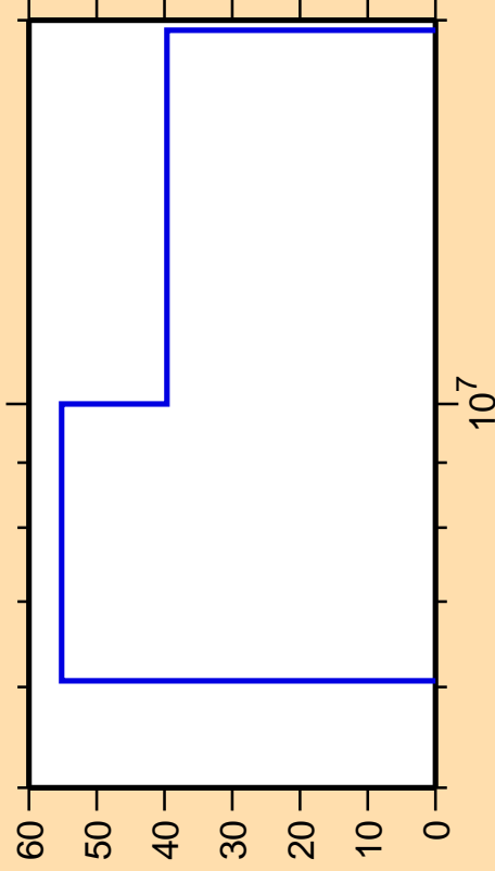
\Delta\sigma/\sigma vs. E for ^{255}\text{Fm}(n,d)
