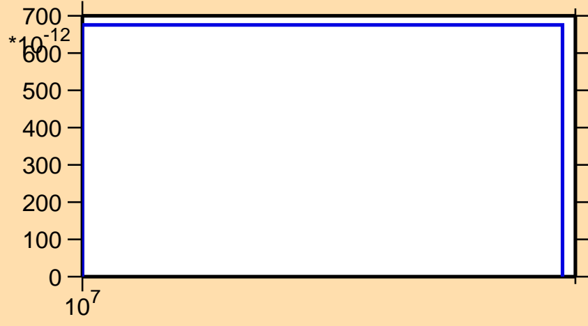
\sigma vs. E for ^{255}\text{Fm}(n,nt)
