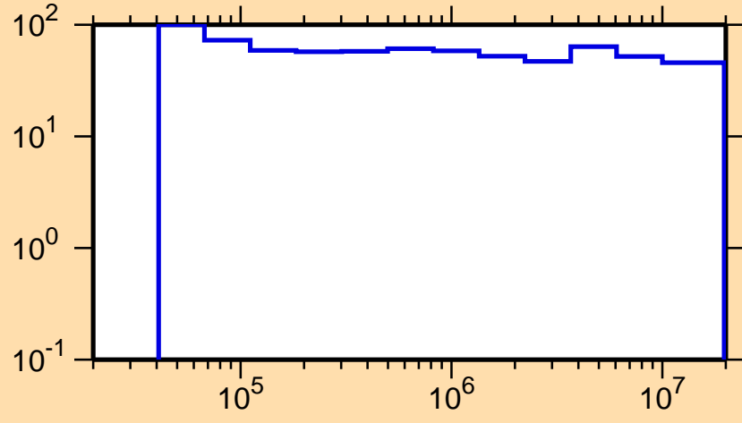
\Delta\sigma/\sigma vs. E for ^{255}\text{Fm}(n,n_1)
