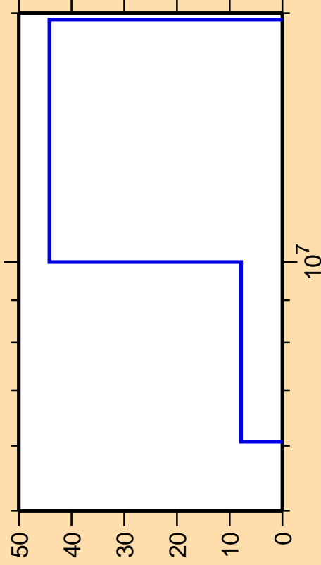
\Delta\sigma/\sigma vs. E for ^{255}\text{Fm}(n,t)
