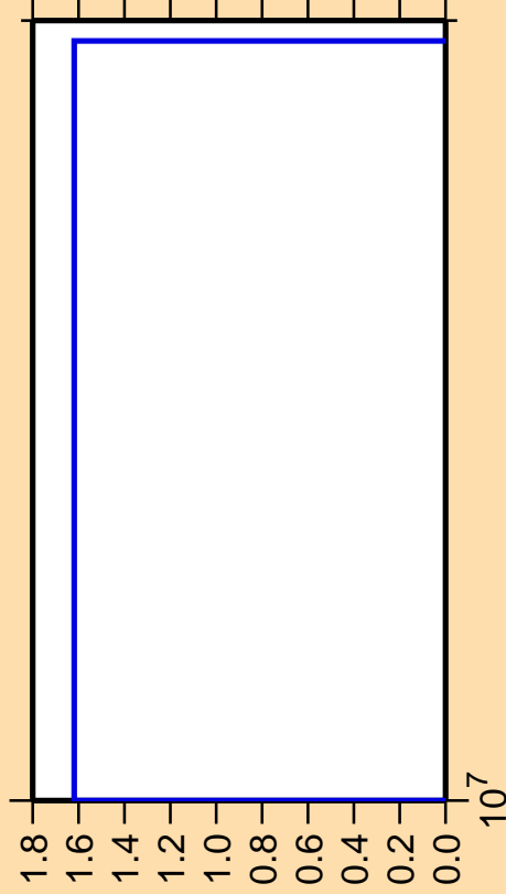
\Delta\sigma/\sigma vs. E for ^{255}\text{Fm}(n,\text{He3})
