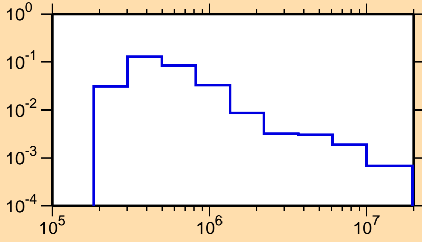
\sigma vs. E for ^{255}\text{Fm}(n,n_2)
