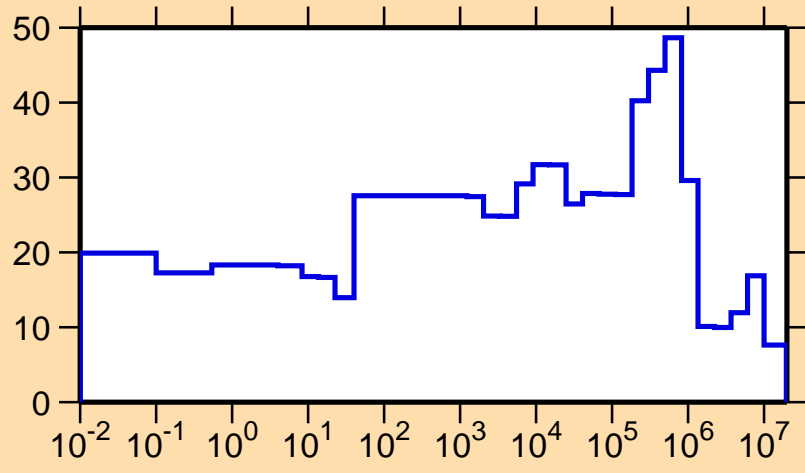
\Delta\sigma/\sigma vs. E for ^{255}\text{Fm}(n,el.)
