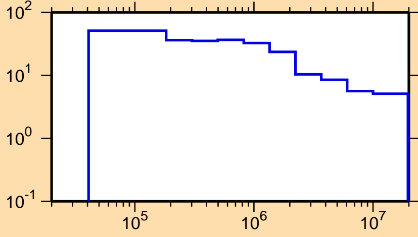
\Delta\sigma/\sigma vs. E for ^{255}\text{Fm}(n,\text{nonel.})
