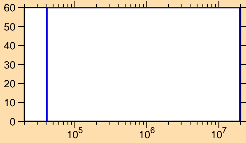
\Delta\sigma/\sigma vs. E for ^{255}\text{Fm}(n,f)
