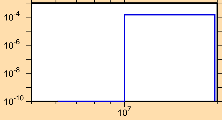
\sigma vs. E for ^{255}\text{Fm}(n,d)
