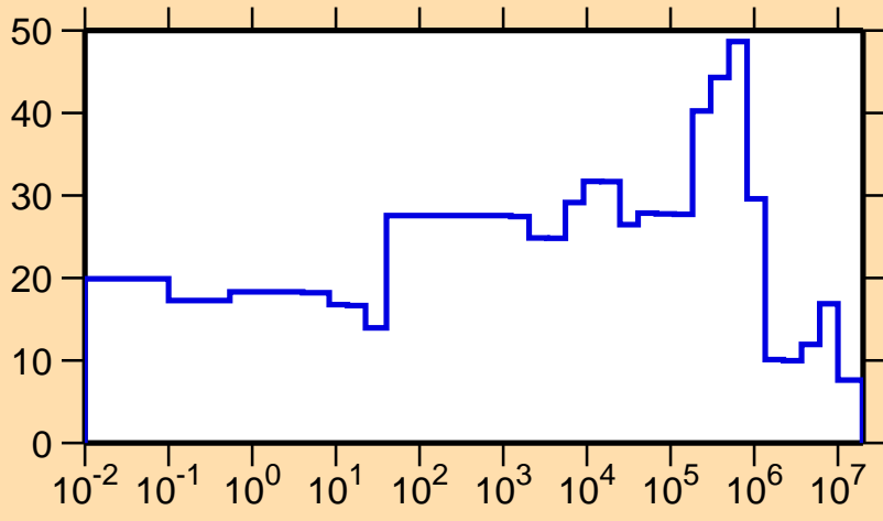
\Delta\sigma/\sigma vs. E for ^{255}\text{Fm}(n,\text{el.})
