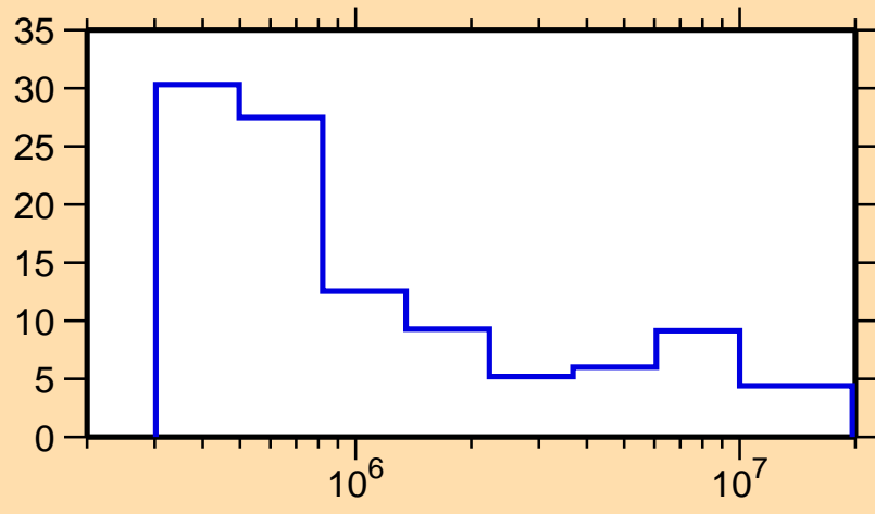
\Delta\sigma/\sigma vs. E for ^{255}\text{Fm}(n, \text{tot.})
