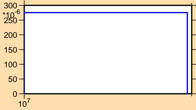
\sigma vs. E for ^{255}\text{Fm}(n,3n)
