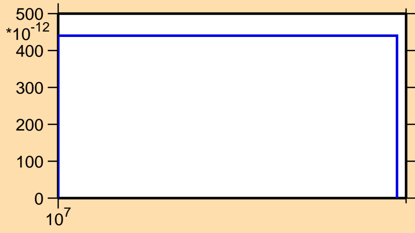
\sigma vs. E for ^{255}\text{Fm}(n,2np)
