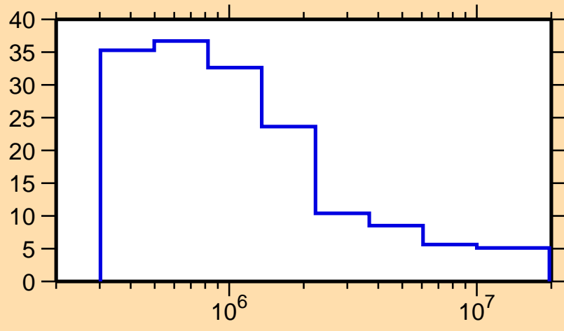
\Delta\sigma/\sigma vs. E for ^{255}\text{Fm}(n,\text{nonel.})
