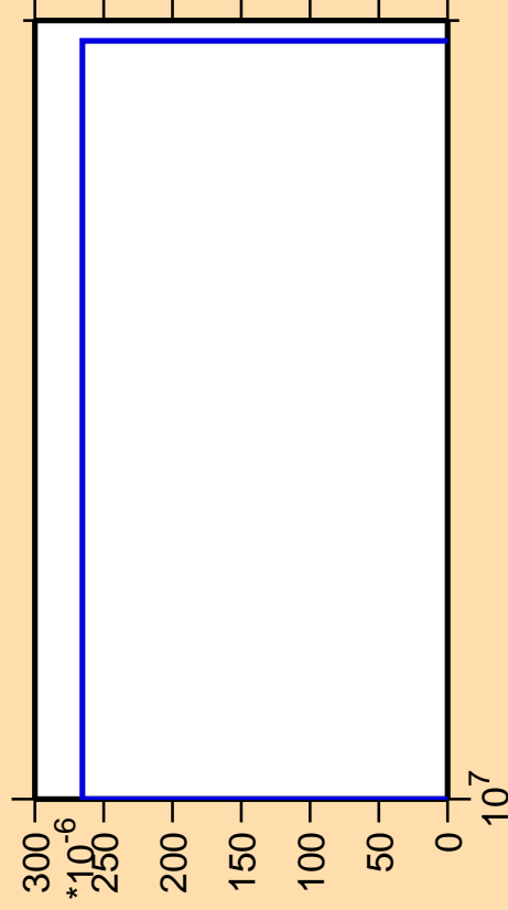
\Delta\sigma/\sigma vs. E for ^{255}\text{Fm} (mt 34)
