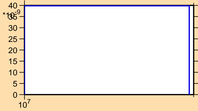
\sigma vs. E for ^{255}\text{Fm}(n,nd)
