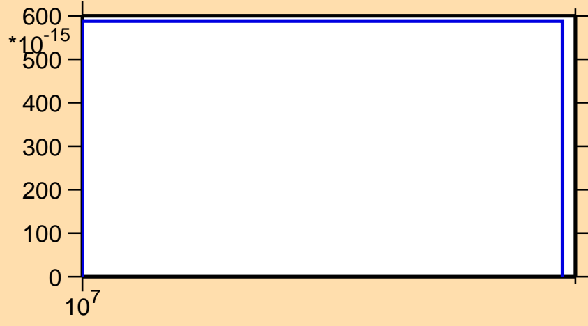
\sigma vs. E for ^{255}\text{Fm}(n,\text{He3})
