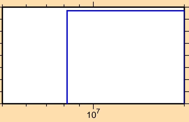
\sigma vs. E for ^{255}\text{Fm} (mt 34)
