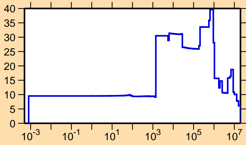
\Delta\sigma/\sigma vs. E for ^{256}\text{Fm}(n,el.)
