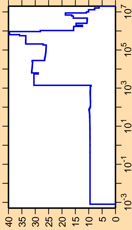
\Delta\sigma/\sigma vs. E for ^{256}\text{Fm}(n,\text{el.})
