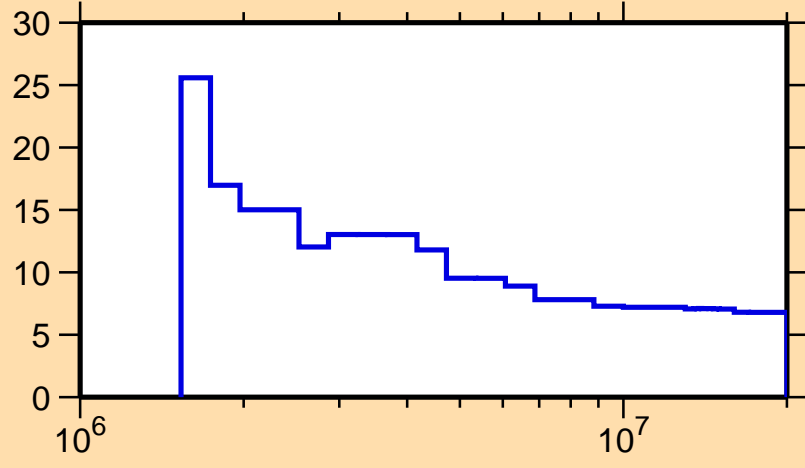
\Delta\sigma/\sigma vs. E for ^{256}\text{Fm}(n, nonel.)
