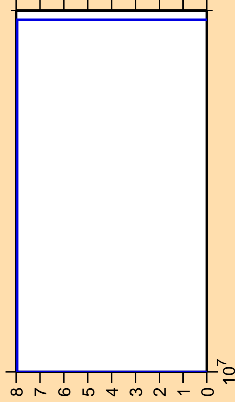
\Delta\sigma/\sigma vs. E for ^{256}\text{Fm}(n,3n\alpha)
