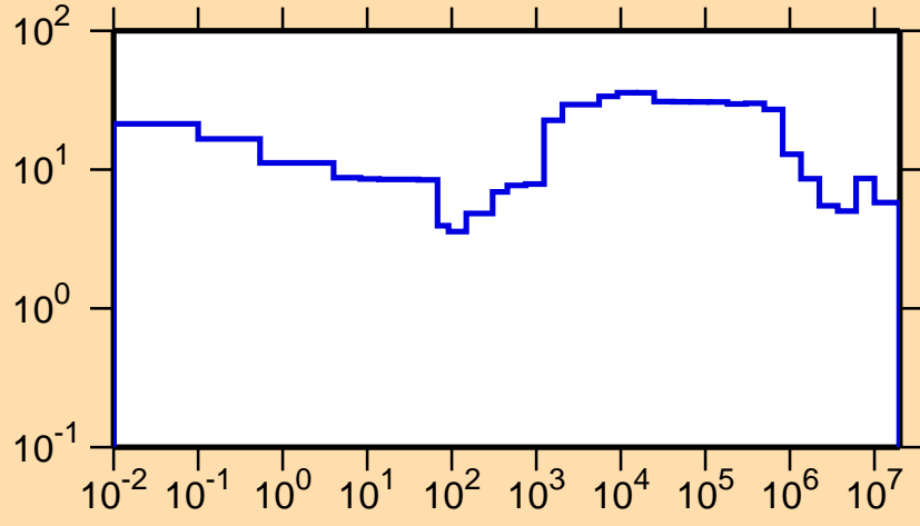
\Delta\sigma/\sigma vs. E for ^{256}\text{Fm}(n,tot.)
