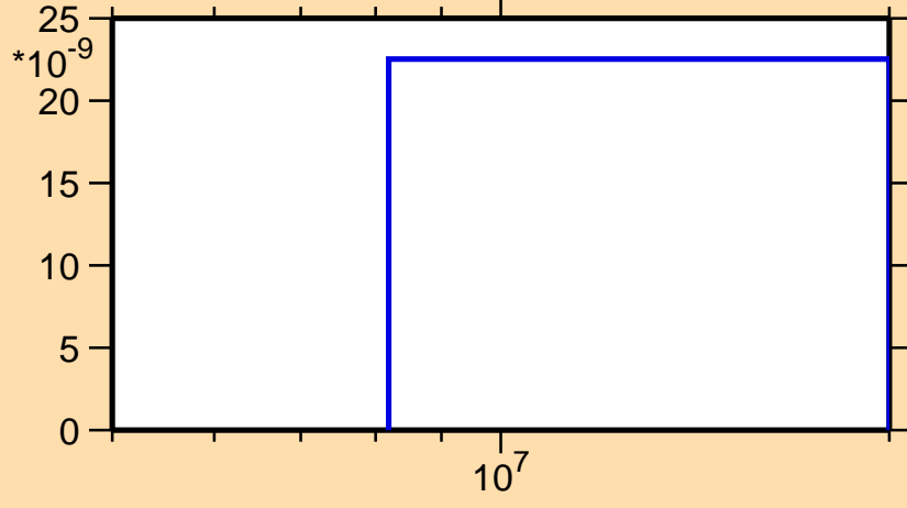
\sigma vs. E for ^{256}\text{Fm}(n,2n\alpha)
