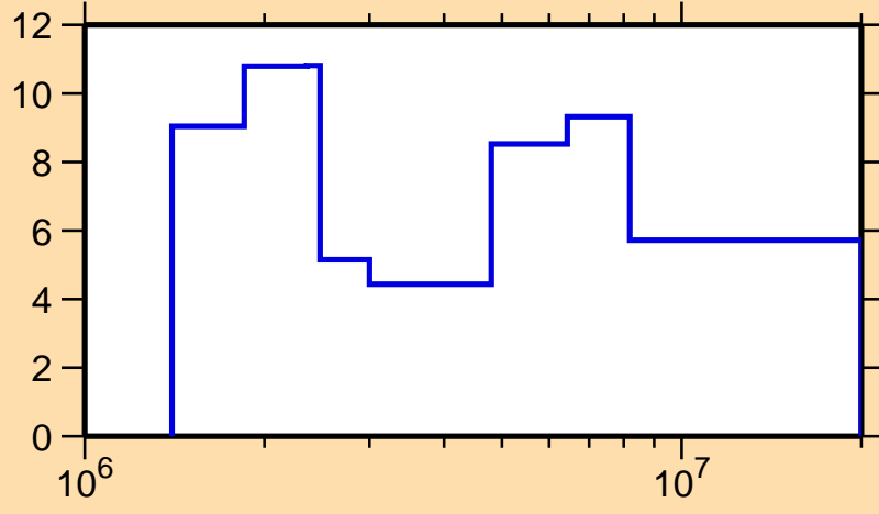
\Delta\sigma/\sigma vs. E for ^{256}\text{Fm}(n,tot.)
