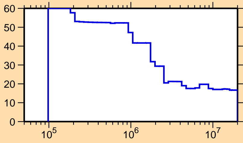
\Delta\sigma/\sigma vs. E for ^{257}\text{Fm}(n,f)
