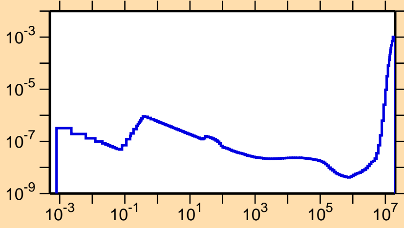
\sigma vs. E for ^{257}\text{Fm}(n,\alpha)
