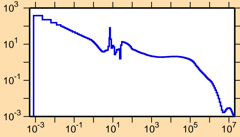
\sigma vs. E for ^{257}\text{Fm}(n,\gamma)
