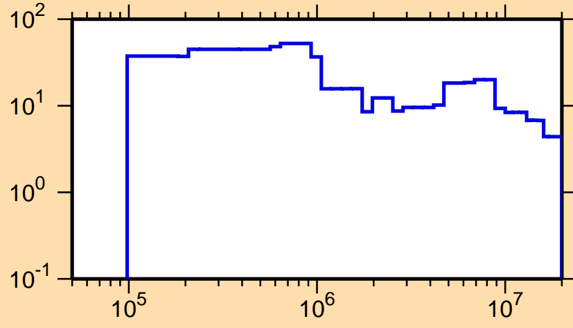
\Delta\sigma/\sigma vs. E for ^{257}\text{Fm}(n,el.)
