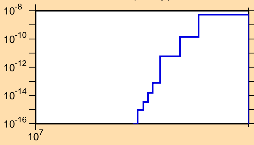
\sigma vs. E for ^{257}\text{Fm}(n,2np)
