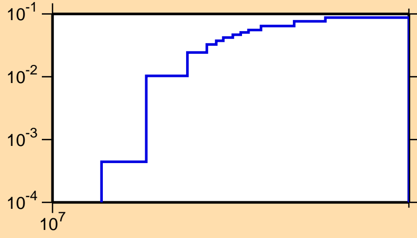
\sigma vs. E for ^{257}\text{Fm}(n,3n)
