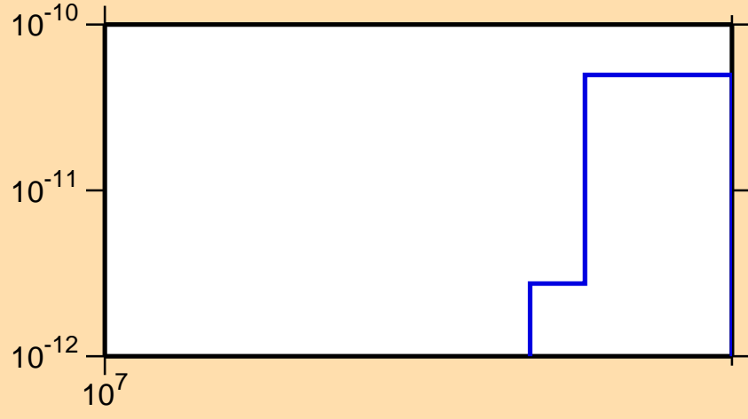
\sigma vs. E for ^{257}\text{Fm}(n,\text{He3})
