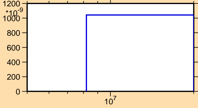
\sigma vs. E for ^{257}\text{Fm}(n,np)
