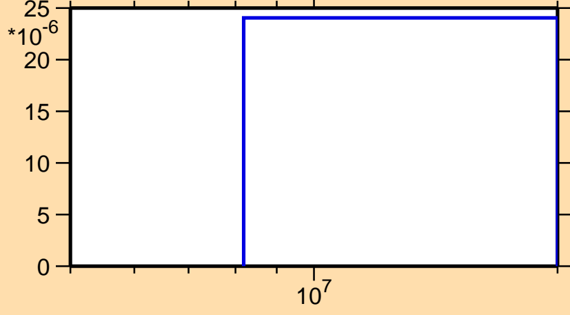
\sigma vs. E for ^{257}\text{Fm}(n,t)
