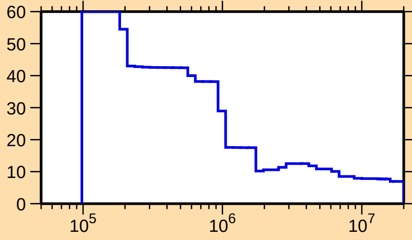
\Delta\sigma/\sigma vs. E for ^{259}\text{Fm}(n,n\text{onel.})
