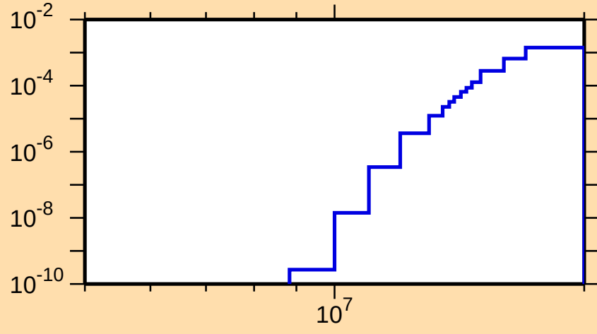
\sigma vs. E for ^{259}\text{Fm}(n,d)
