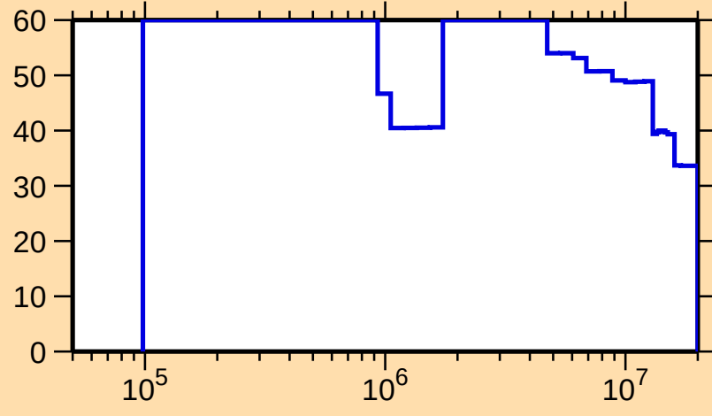
\Delta\sigma/\sigma vs. E for ^{259}\text{Fm}(n,n_1)
