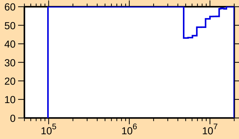
\Delta\sigma/\sigma vs. E for ^{259}\text{Fm}(n,\text{inel.})
