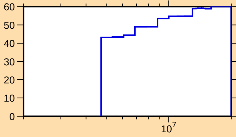
\Delta\sigma/\sigma vs. E for ^{259}\text{Fm}(n,\text{inel.})
