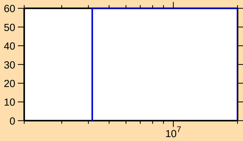
\Delta\sigma/\sigma vs. E for ^{259}\text{Fm}(n,\gamma)
