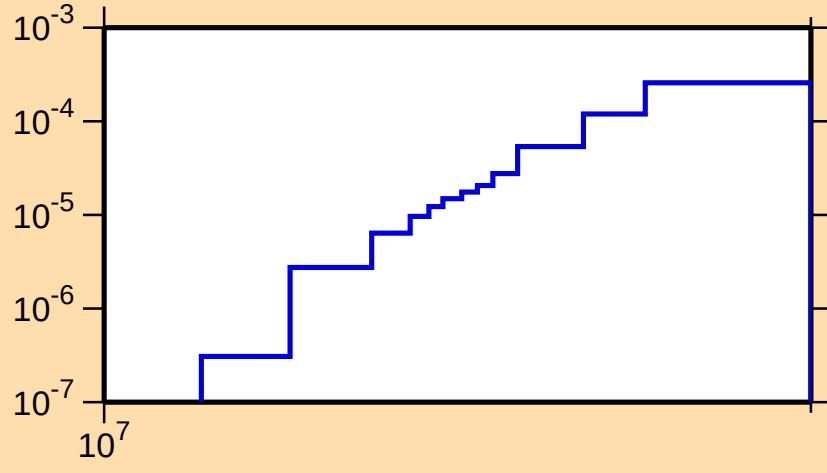
\sigma vs. E for ^{259}\text{Fm}(n,3n)
