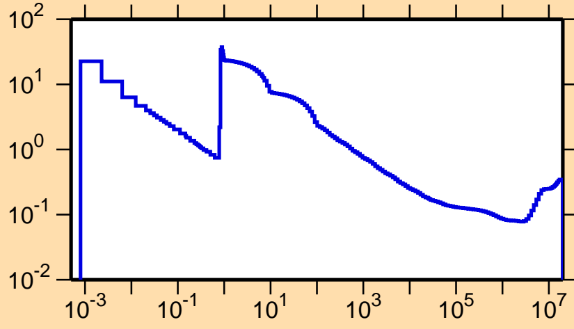
\sigma vs. E for ^{204}\text{Fr}(n,\text{nonel.})
