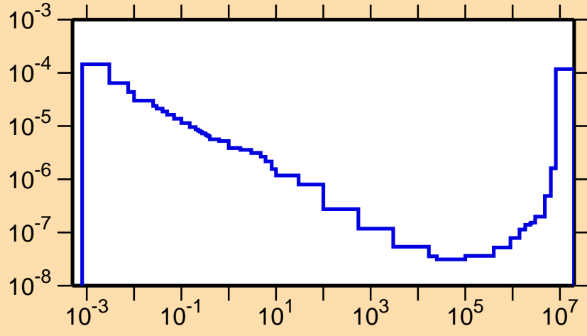
\sigma vs. E for ^{204}\text{Fr}(n,p\alpha)
