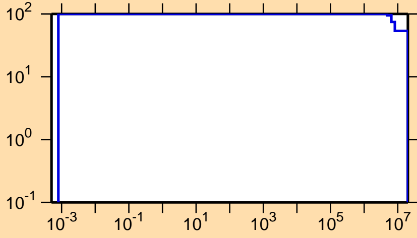
\Delta\sigma/\sigma vs. E for ^{204}\text{Fr}(n,p)
