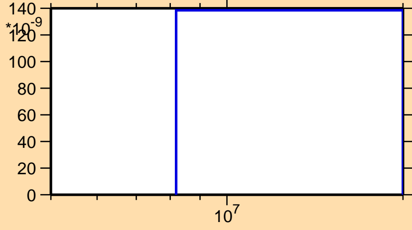
\sigma vs. E for ^{204}\text{Fr}(n,\text{nd})
