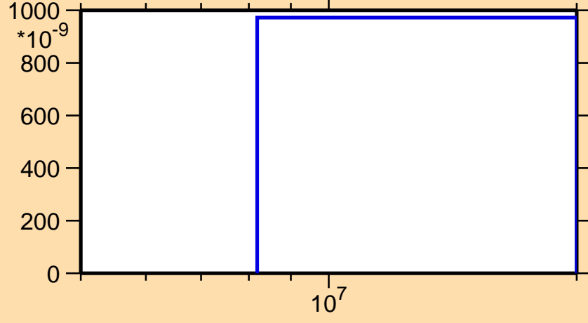
\sigma vs. E for ^{204}\text{Fr}(n,2np)
