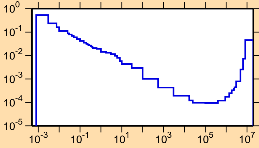
\sigma vs. E for ^{204}\text{Fr}(n,\alpha)
