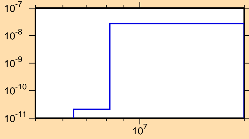
\sigma vs. E for ^{204}\text{Fr}(n,2n\alpha)
