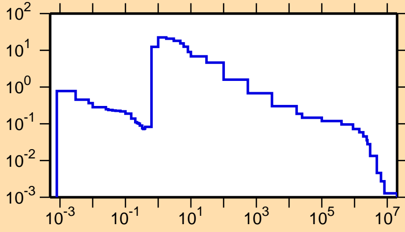
\sigma vs. E for ^{204}\text{Fr}(n,\gamma)
