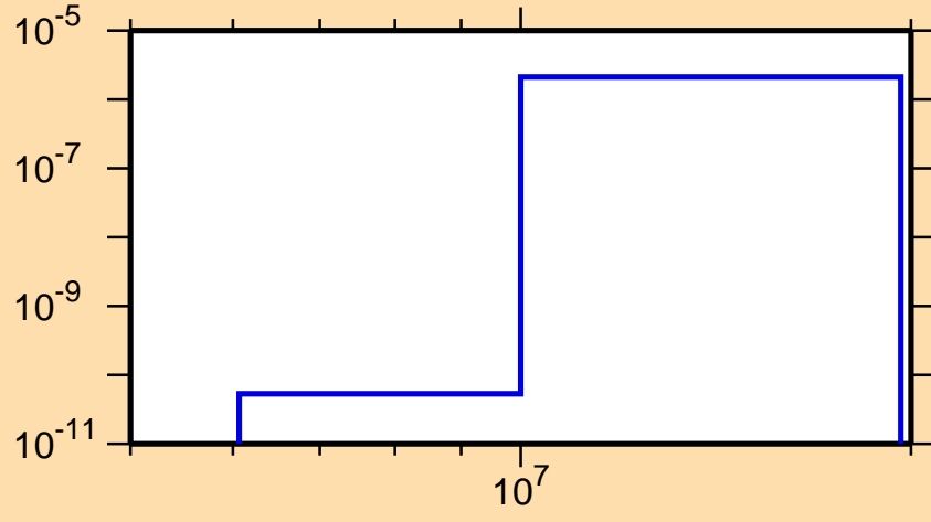
\sigma vs. E for ^{205}\text{Fr}(n,\text{He3})
