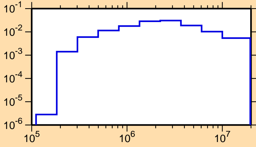
\sigma vs. E for ^{205}\text{Fr}(n,n_1)
