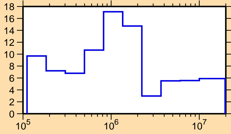
\Delta\sigma/\sigma vs. E for ^{205}\text{Fr}(n, el.)
