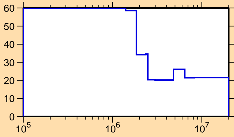
\Delta\sigma/\sigma vs. E for ^{205}\text{Fr}(n,n_1)
