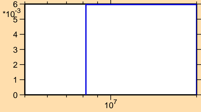
\sigma vs. E for ^{205}\text{Fr}(n,2n)
