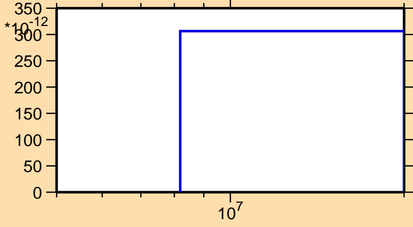
\sigma vs. E for ^{205}\text{Fr}(n,3n)
