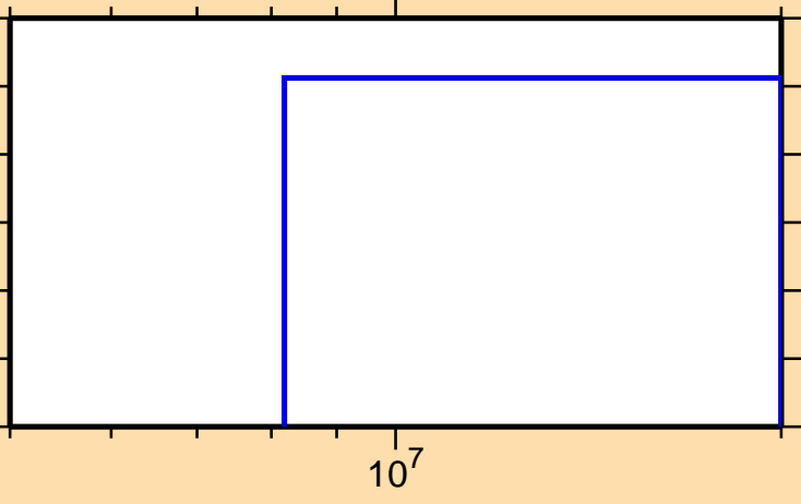
\sigma vs. E for ^{205}\text{Fr}(n,\text{pd})
