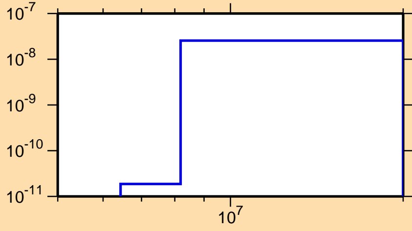
\sigma vs. E for ^{205}\text{Fr}(\text{mt117})
