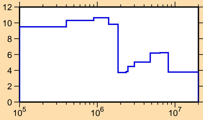
\Delta\sigma/\sigma vs. E for ^{205}\text{Fr}(n,\text{tot.})
