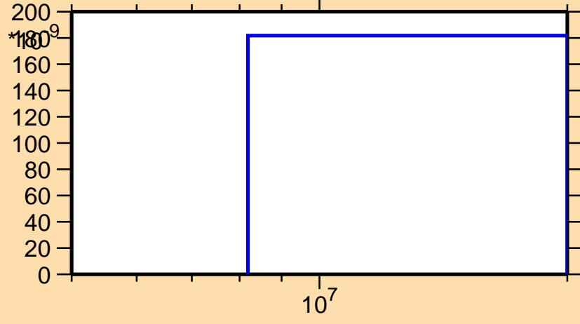
\sigma vs. E for ^{205}\text{Fr}(n,2np)
