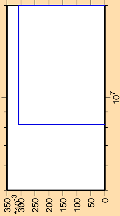
\Delta\sigma/\sigma vs. E for ^{205}\text{Fr}(n,3n\alpha)
