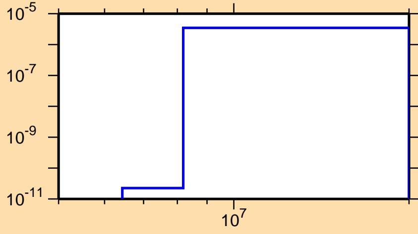
\sigma vs. E for ^{206}\text{Fr}(n,\text{He3})
