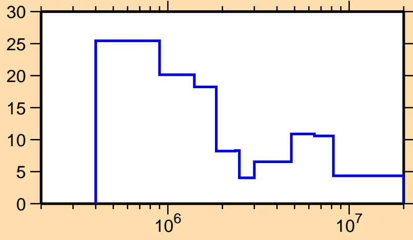
\Delta\sigma/\sigma vs. E for ^{206}\text{Fr}(n, el.)
