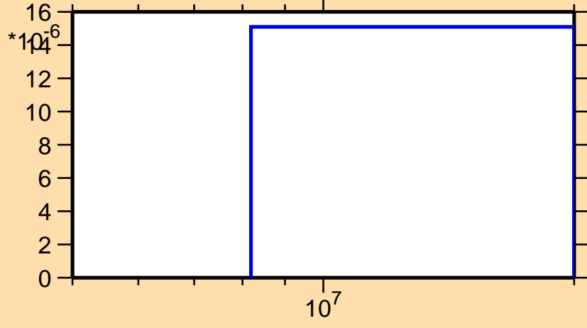
\sigma vs. E for ^{206}\text{Fr}(n,2np)
