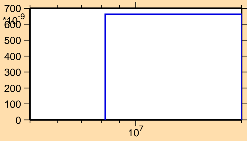
\sigma vs. E for ^{206}\text{Fr}(n,\text{nd})
