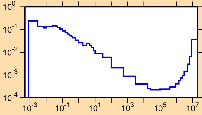
\sigma vs. E for ^{206}\text{Fr}(n,\alpha)
