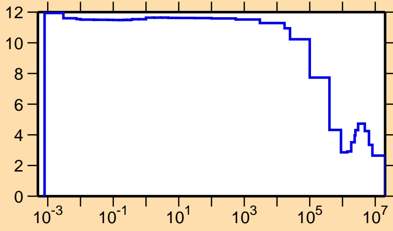
\sigma vs. E for ^{206}\text{Fr}(n,\text{el.})
