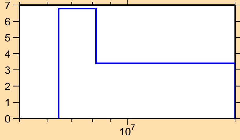
\Delta\sigma/\sigma vs. E for ^{206}\text{Fr}(n,\text{tot.})
