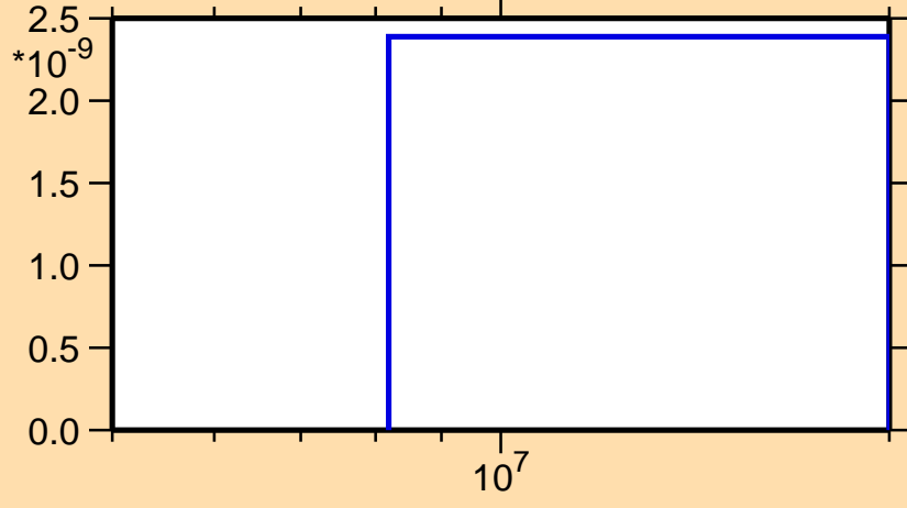
\sigma vs. E for ^{206}\text{Fr}(n,\text{pd})
