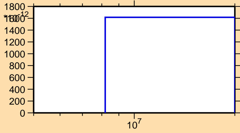
\sigma vs. E for ^{206}\text{Fr}(\text{mt117})
