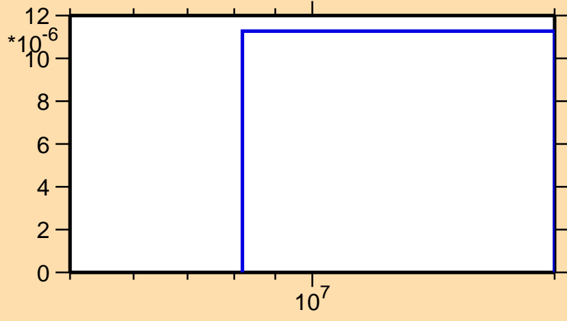
\sigma vs. E for ^{206}\text{Fr}(n,2np)
