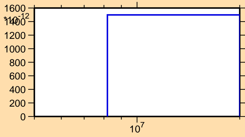
\sigma vs. E for ^{206}\text{Fr}(\text{mt117})
