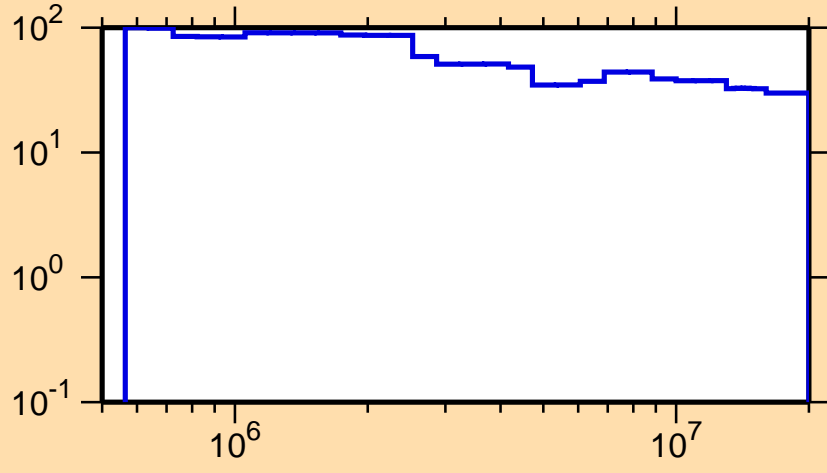
\Delta\sigma/\sigma vs. E for ^{207}\text{Fr}(n,n_1)
