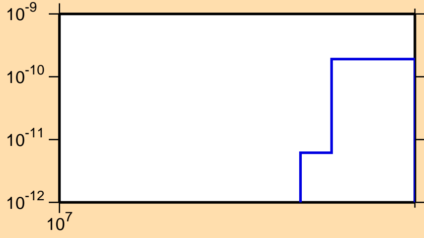
\sigma vs. E for ^{207}\text{Fr}(n,\text{pt})
