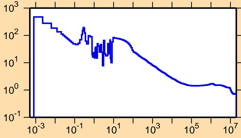
\sigma vs. E for ^{207}\text{Fr}(n,\text{nonel.})
