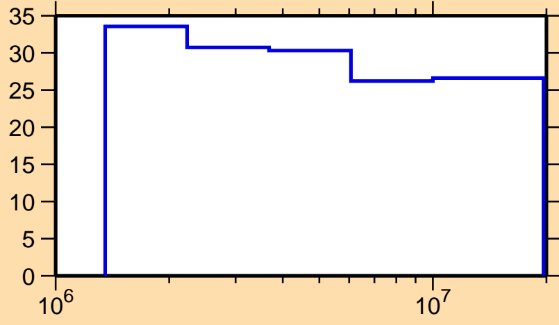
\Delta\sigma/\sigma vs. E for ^{207}\text{Fr}(n,ncont.)
