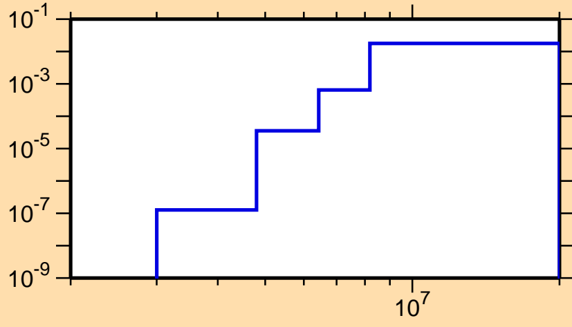
\sigma vs. E for ^{207}\text{Fr}(n,np)
