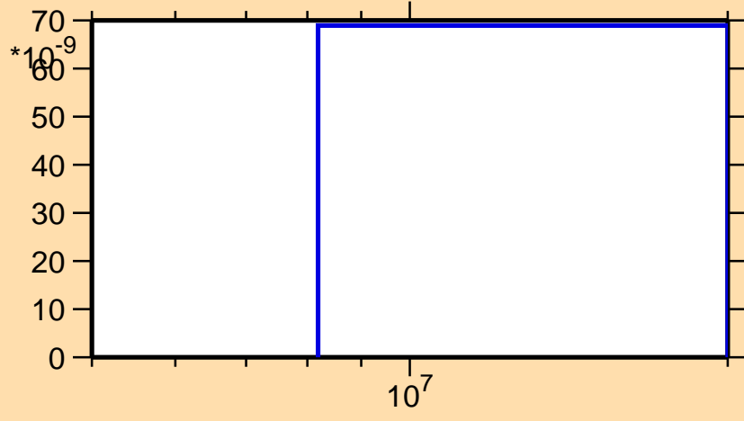
\sigma vs. E for ^{207}\text{Fr}(n,\text{nd})
