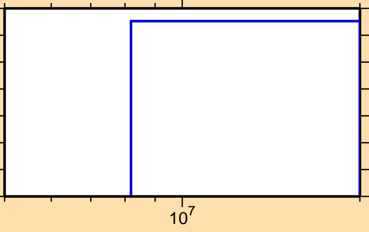
\sigma vs. E for ^{207}\text{Fr}(n,3n)
