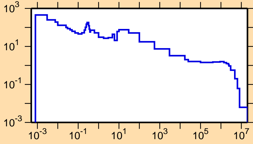
\sigma vs. E for ^{207}\text{Fr}(n,\gamma)
