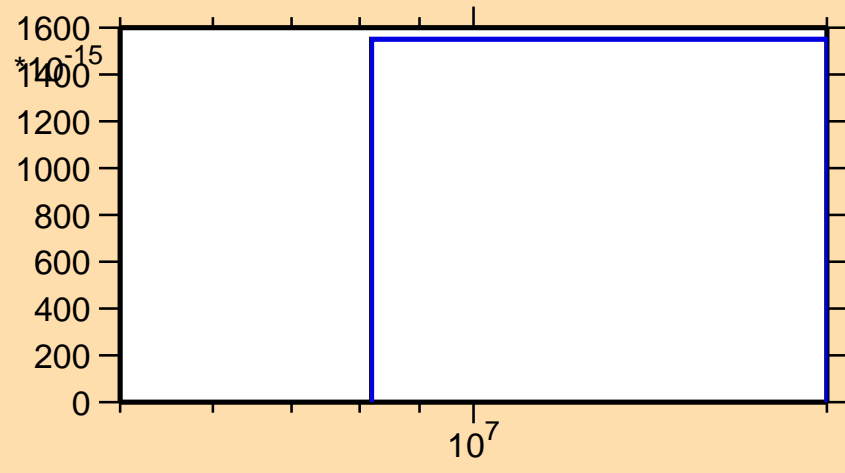
\sigma vs. E for ^{207}\text{Fr}(n,3n\alpha)
