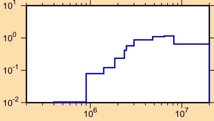
\sigma vs. E for ^{207}\text{Fr}(n,\text{inel.})
