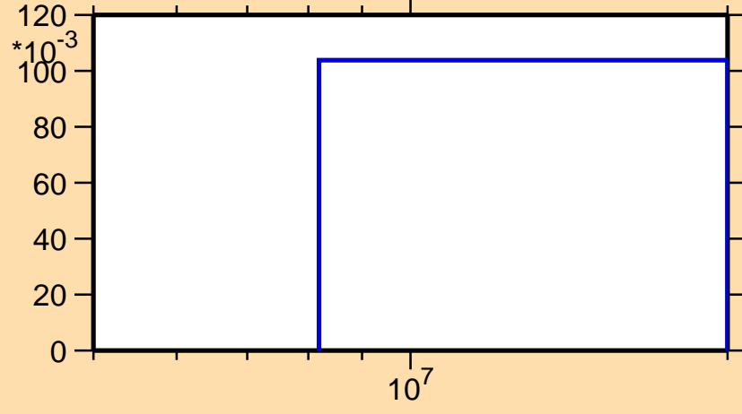
\sigma vs. E for ^{207}\text{Fr}(n,2n)
