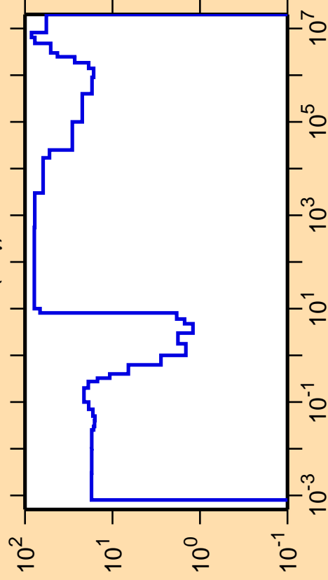
\Delta\sigma/\sigma vs. E for ^{207}\text{Fr}(n,\gamma)
