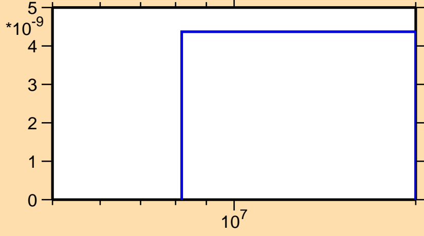
\sigma vs. E for ^{207}\text{Fr}(n,\text{pd})
