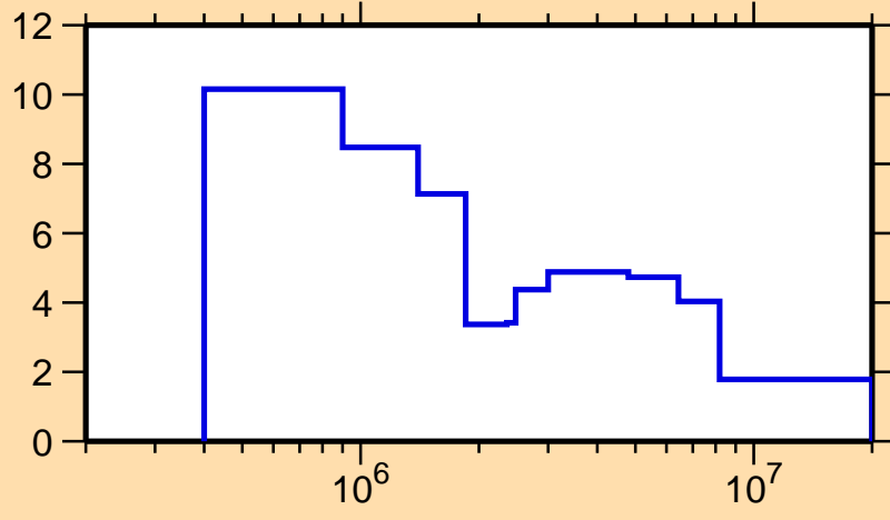
\Delta\sigma/\sigma vs. E for ^{207}\text{Fr}(n,\text{tot.})
