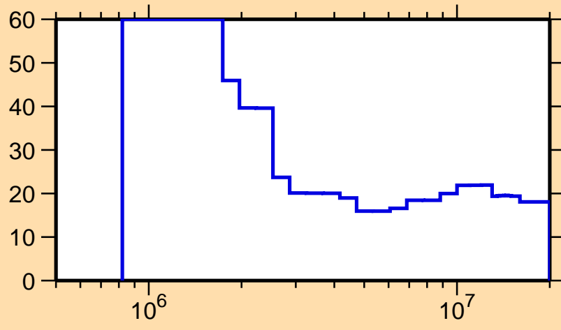
\Delta\sigma/\sigma vs. E for ^{208}\text{Fr}(n,n\text{cont.})
