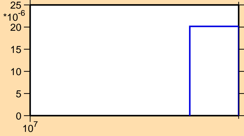
\sigma vs. E for ^{208}\text{Fr}(n,3n)
