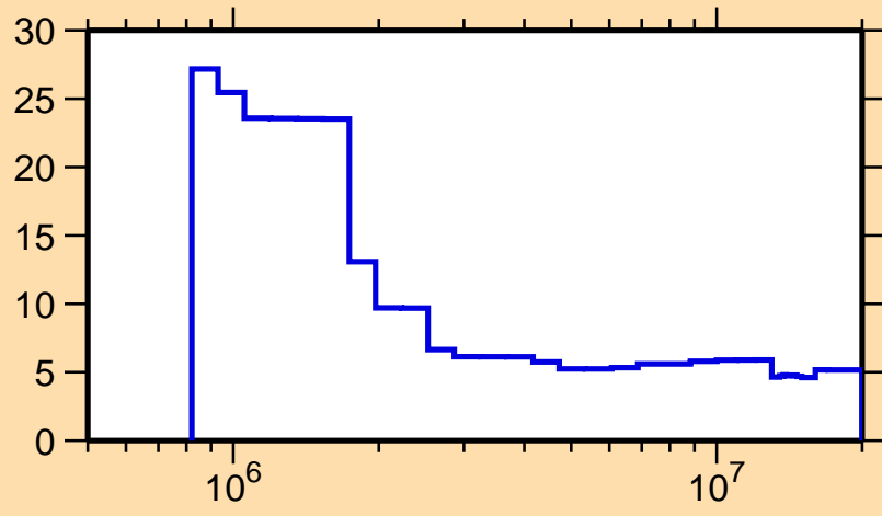
\Delta\sigma/\sigma vs. E for ^{208}\text{Fr}(n,n\text{nonel.})
