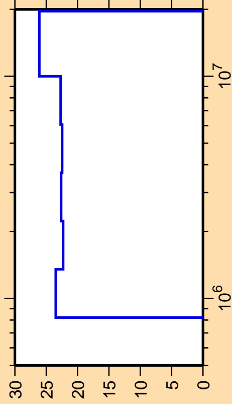
\Delta\sigma/\sigma vs. E for ^{208}\text{Fr}(n,n_2)
