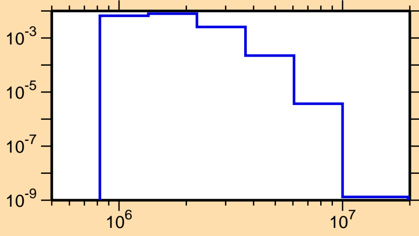
\sigma vs. E for ^{208}\text{Fr}(n,n_4)
