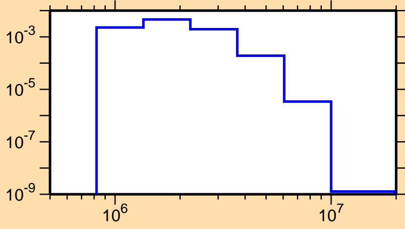
\sigma vs. E for ^{208}\text{Fr}(n,n_2)
