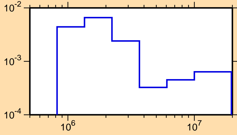
\sigma vs. E for ^{208}\text{Fr}(n,n_3)
