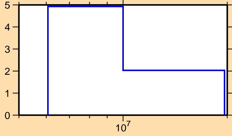
\Delta\sigma/\sigma vs. E for ^{208}\text{Fr}(n,\text{el.})
