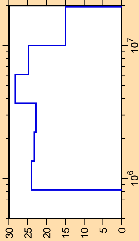
\Delta\sigma/\sigma vs. E for ^{208}\text{Fr}(n,n_3)
