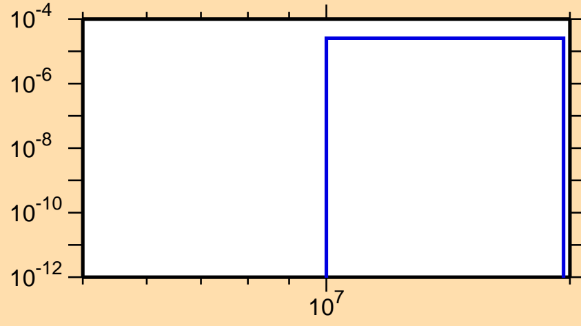
\sigma vs. E for ^{208}\text{Fr}(n,2np)
