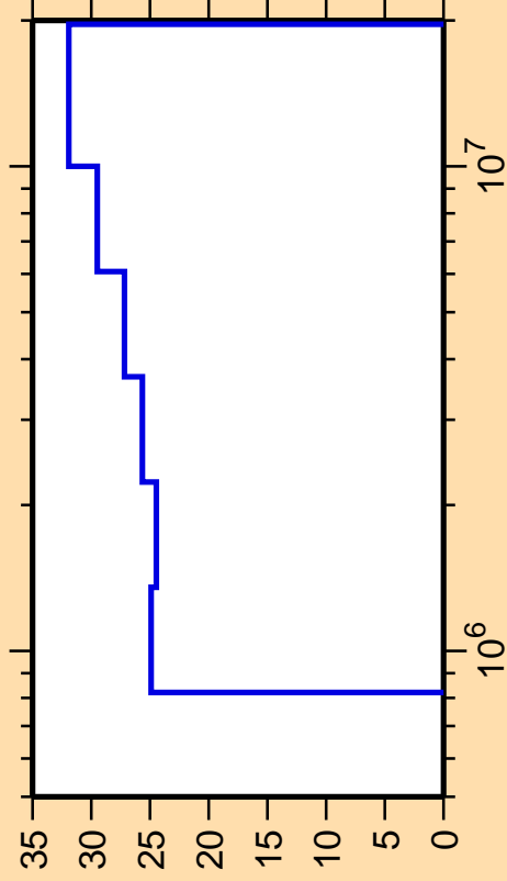
\Delta\sigma/\sigma vs. E for ^{208}\text{Fr}(n,n_4)
