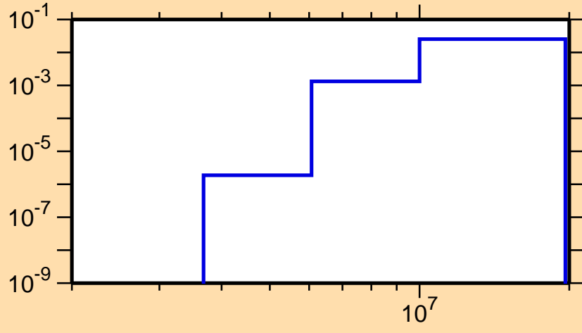
\sigma vs. E for ^{208}\text{Fr}(n,np)
