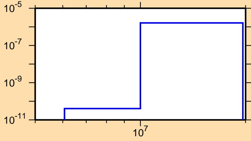
\sigma vs. E for ^{208}\text{Fr}(n,\text{He3})
