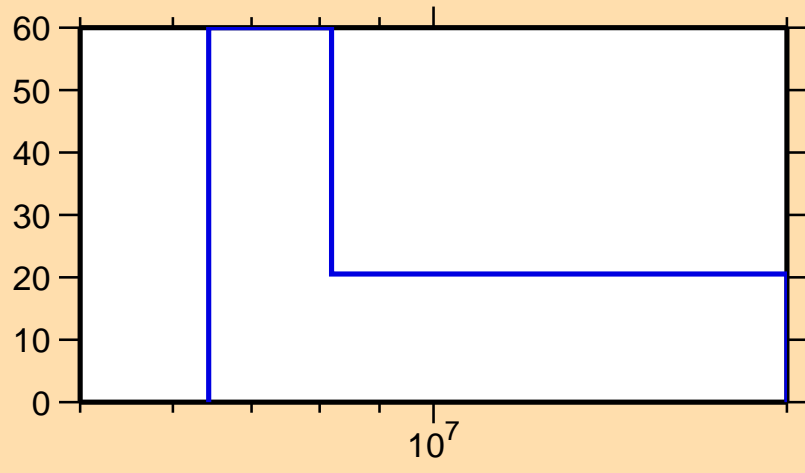
\Delta\sigma/\sigma vs. E for ^{208}\text{Fr}(n,2n)
