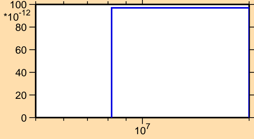
\sigma vs. E for ^{208}\text{Fr}(n,pt)
