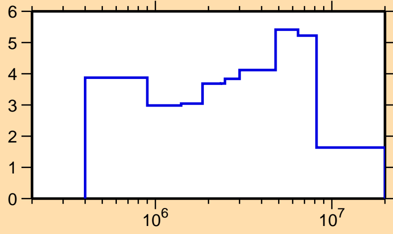
\Delta\sigma/\sigma vs. E for ^{208}\text{Fr}(n, el.)
