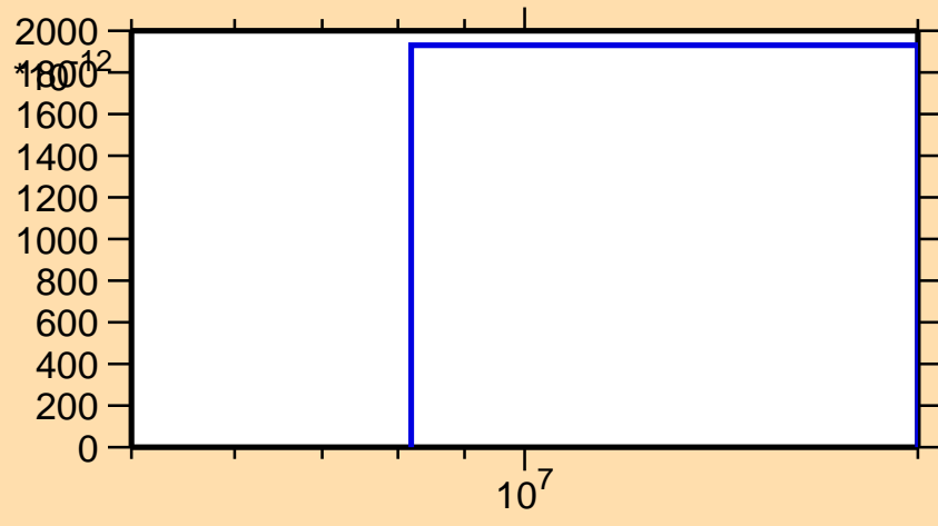
\sigma vs. E for ^{208}\text{Fr}(n,\text{pd})
