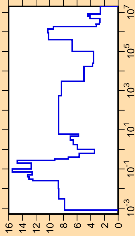
\Delta\sigma/\sigma vs. E for ^{208}\text{Fr}(n,\text{tot.})
