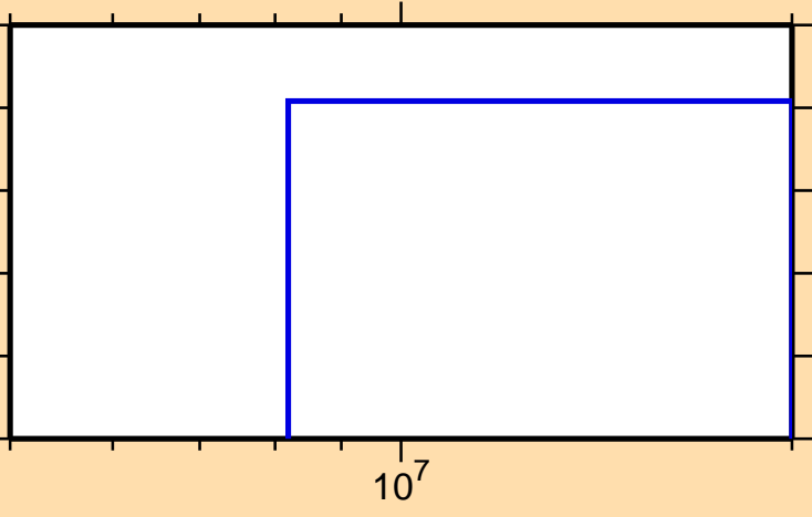
\sigma vs. E for ^{208}\text{Fr}(n,\text{nd})
