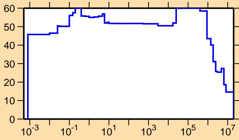
\Delta\sigma/\sigma vs. E for ^{208}\text{Fr}(n,p)
