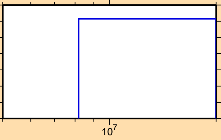
\sigma vs. E for ^{208}\text{Fr}(\text{mt117})
