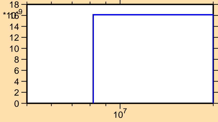
\sigma vs. E for ^{208}\text{Fr}(\text{mt } 45)
