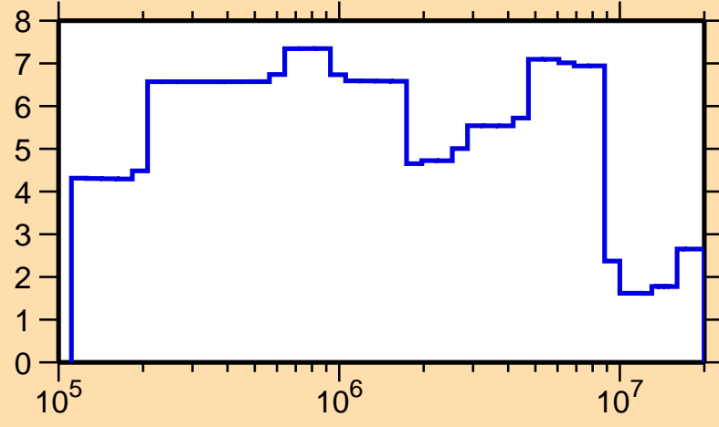
\Delta\sigma/\sigma vs. E for ^{209}\text{Fr}(n, el.)
