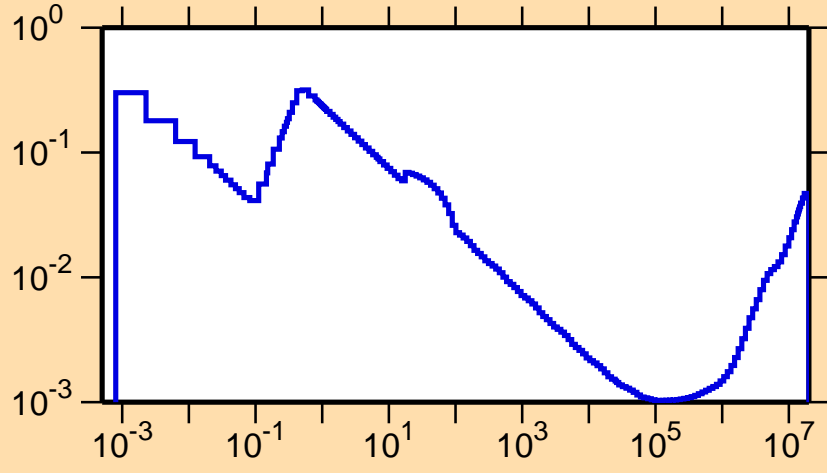
\sigma vs. E for ^{209}\text{Fr}(n,p)
