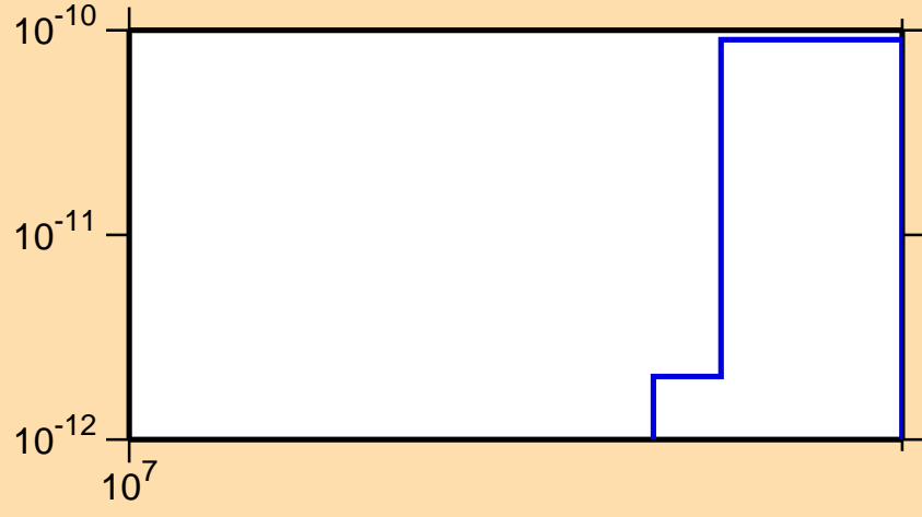
\sigma vs. E for ^{209}\text{Fr}(\text{mt } 34)
