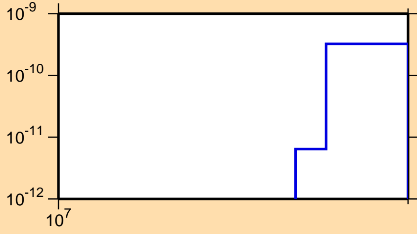
\sigma vs. E for ^{209}\text{Fr}(n,\text{pt})
