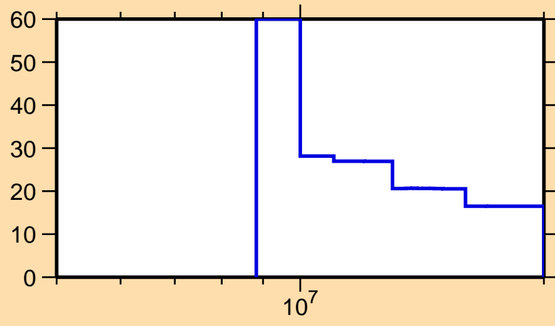
\Delta\sigma/\sigma vs. E for ^{209}\text{Fr}(n,2n)
