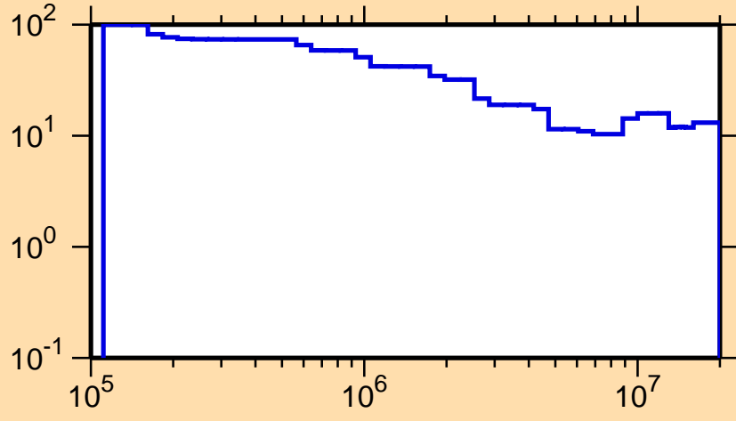
\Delta\sigma/\sigma vs. E for ^{209}\text{Fr}(n,ncont.)
