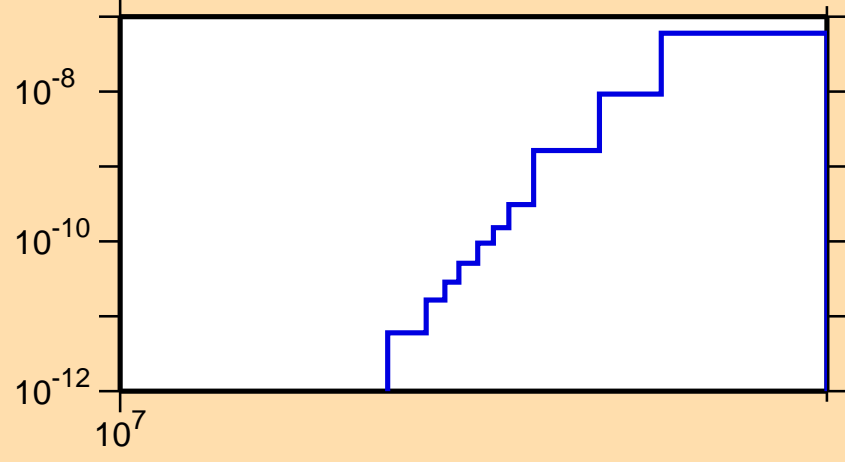
\sigma vs. E for ^{209}\text{Fr}(n,\text{pd})
