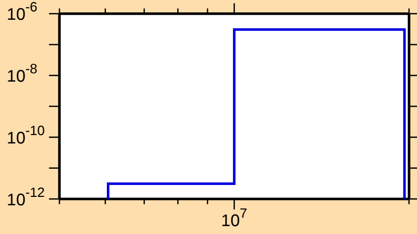
\sigma vs. E for ^{209}\text{Fr}(n,\text{He3})
