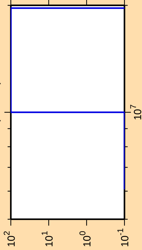
\Delta\sigma/\sigma vs. E for ^{209}\text{Fr}(\text{mt117})
