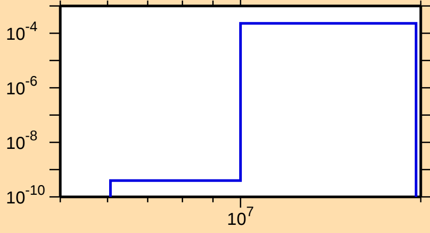
\sigma vs. E for ^{209}\text{Fr}(n,t)
