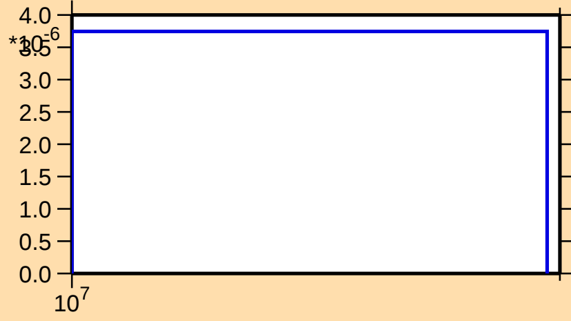
\sigma vs. E for ^{209}\text{Fr}(n,3n)
