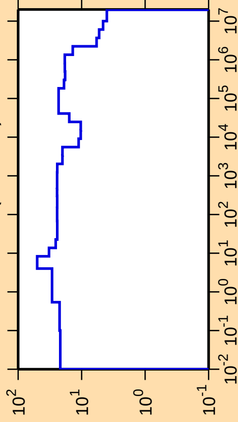
\Delta\sigma/\sigma vs. E for ^{209}\text{Fr}(n,\text{nonel.})
