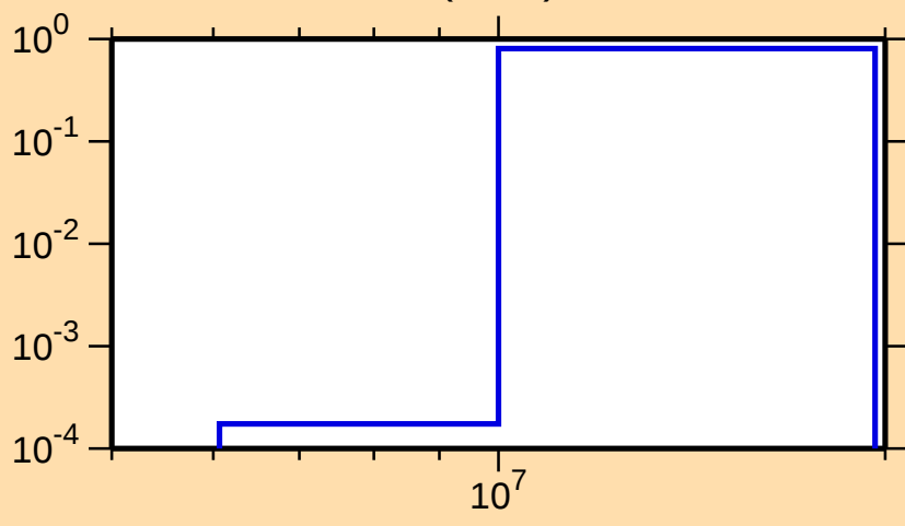
\sigma vs. E for ^{209}\text{Fr}(n,2n)
