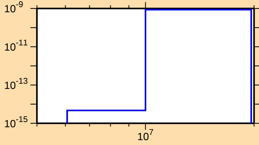
\sigma vs. E for ^{209}\text{Fr}(\text{mt117})
