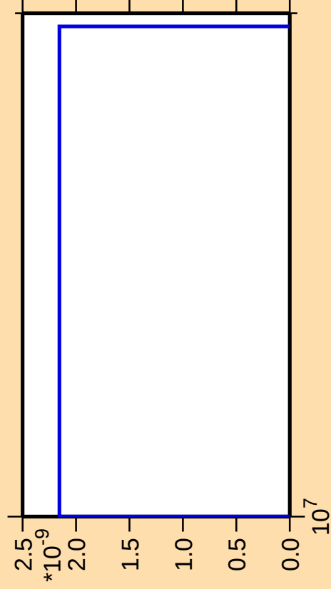
\Delta\sigma/\sigma vs. E for ^{209}\text{Fr}(\text{mt } 42)
