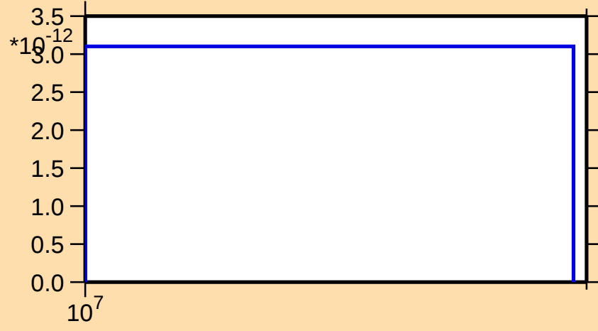
\sigma vs. E for ^{209}\text{Fr}(n,\text{pt})
