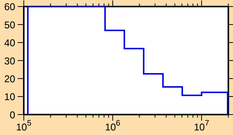
\Delta\sigma/\sigma vs. E for ^{209}\text{Fr}(n,n\text{cont.})
