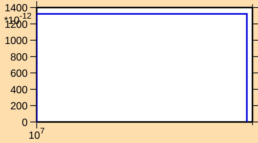
\sigma vs. E for ^{209}\text{Fr}(n,\text{nt})
