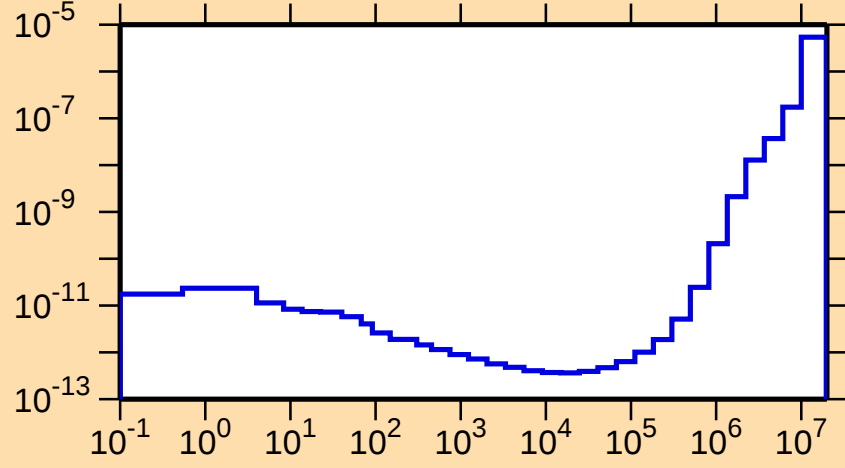
\sigma vs. E for ^{209}\text{Fr}(n,p\alpha)
