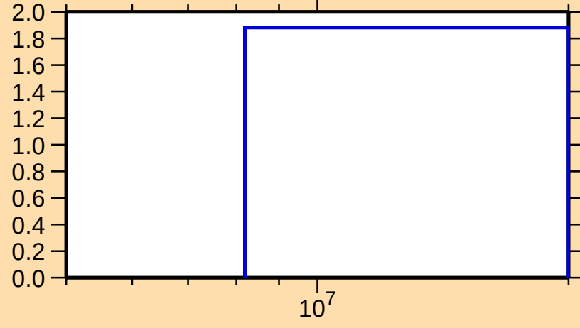
\Delta\sigma/\sigma vs. E for ^{209}\text{Fr}(n,\text{tot.})
