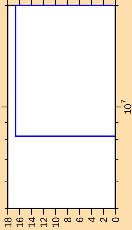
\Delta\sigma/\sigma vs. E for ^{209}\text{Fr}(n,p)
