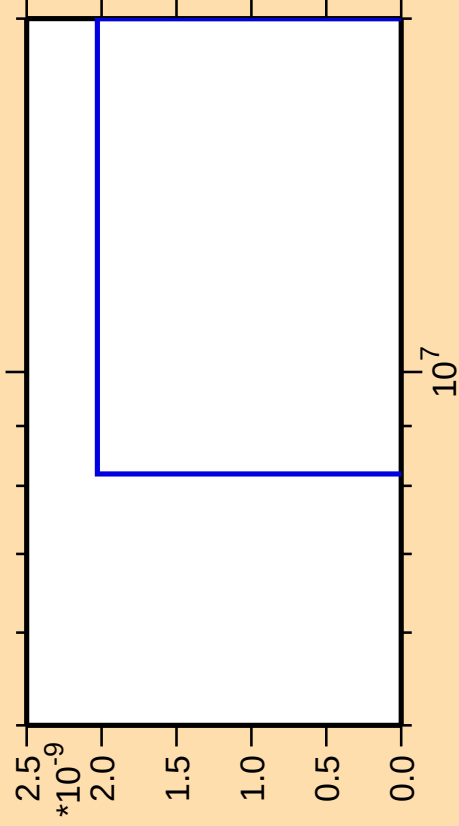
\Delta\sigma/\sigma vs. E for ^{209}\text{Fr}(\text{mt } 42)
