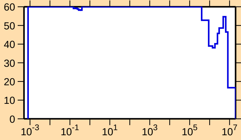
\Delta\sigma/\sigma vs. E for ^{209}\text{Fr}(n,p)
