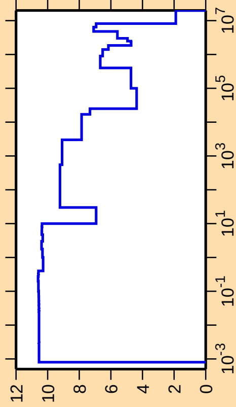
\Delta\sigma/\sigma vs. E for ^{209}\text{Fr}(n,\text{el.})
