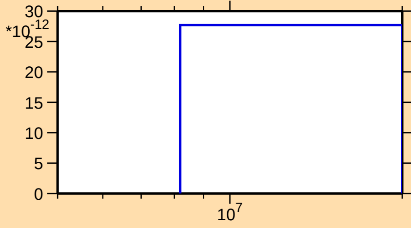
\sigma vs. E for ^{209}\text{Fr}(n,3n\alpha)
