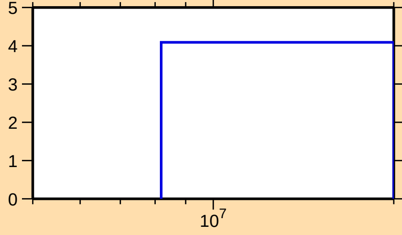
\Delta\sigma/\sigma vs. E for ^{209}\text{Fr}(n,\text{nonel.})
