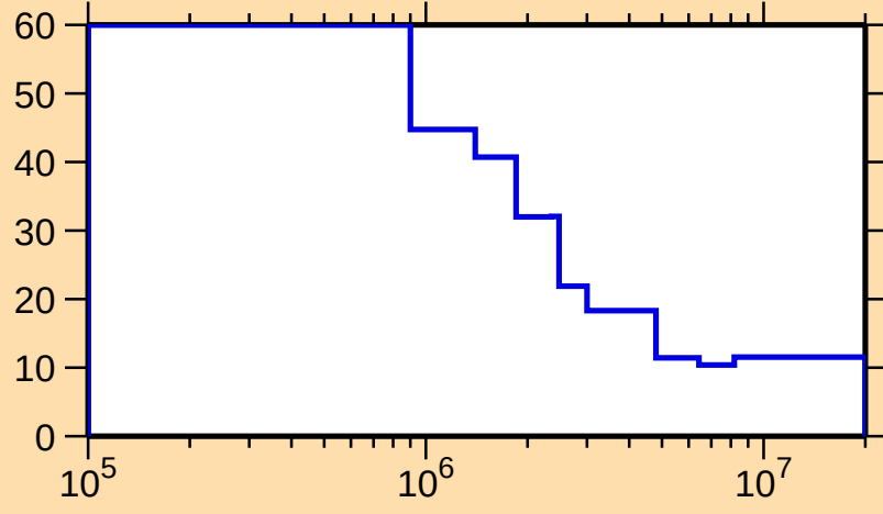
\Delta\sigma/\sigma vs. E for ^{209}\text{Fr}(n,n\text{cont.})
