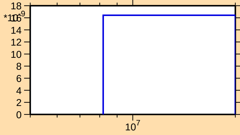
\sigma vs. E for ^{209}\text{Fr}(\text{mt } 45)
