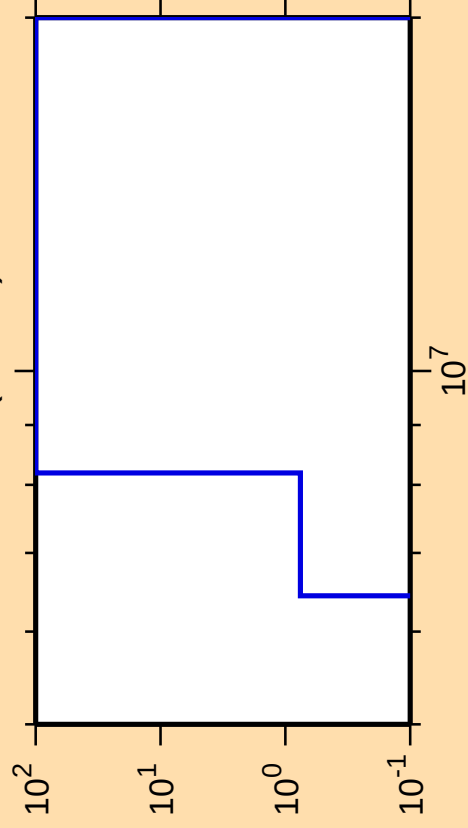
\Delta\sigma/\sigma vs. E for ^{209}\text{Fr}(n,\text{He3})
