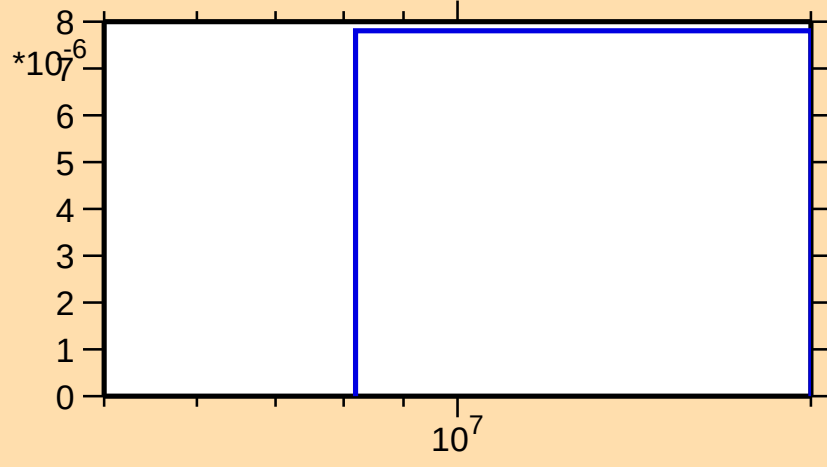
\sigma vs. E for ^{209}\text{Fr}(n,2np)
