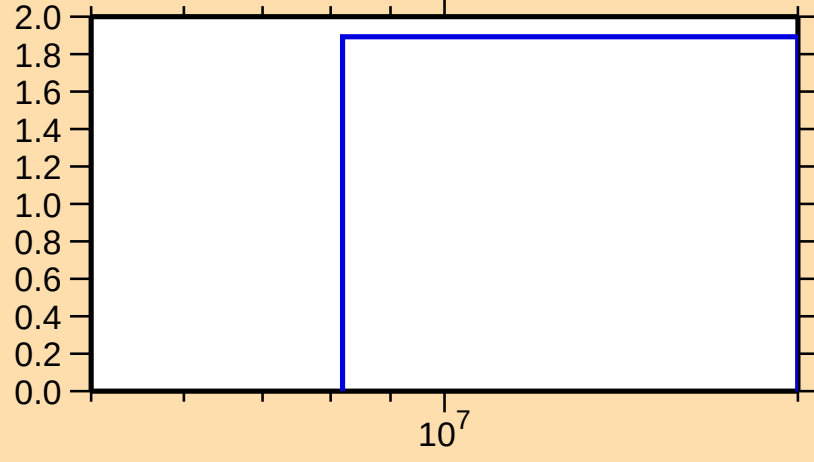
\Delta\sigma/\sigma vs. E for ^{209}\text{Fr}(n,\text{el.})
