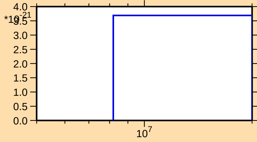
\sigma vs. E for ^{209}\text{Fr}(\text{mt } 42)
