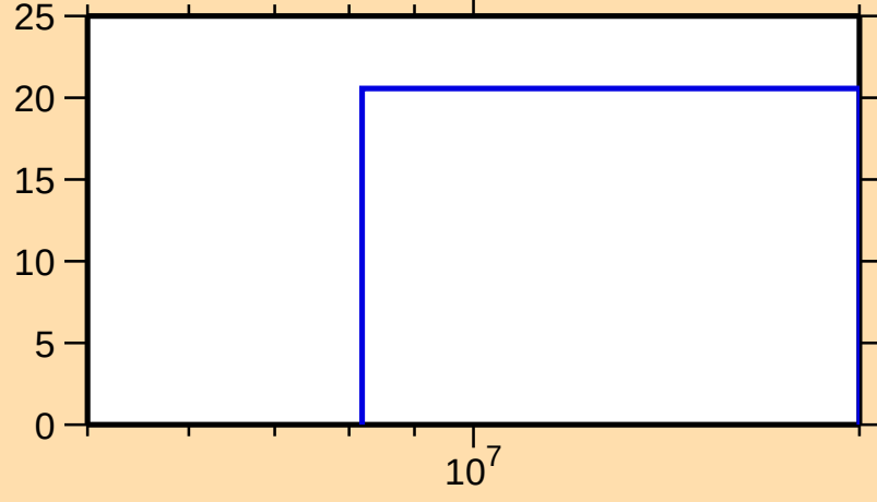
\Delta\sigma/\sigma vs. E for ^{209}\text{Fr}(n,2n)
