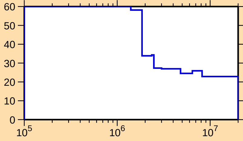
\Delta\sigma/\sigma vs. E for ^{209}\text{Fr}(n,n_1)
