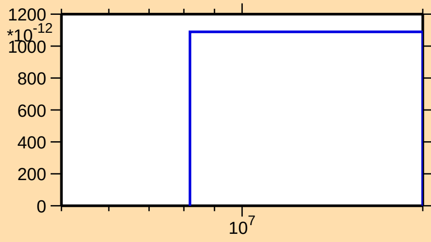
\sigma vs. E for ^{209}\text{Fr}(n,\text{pd})
