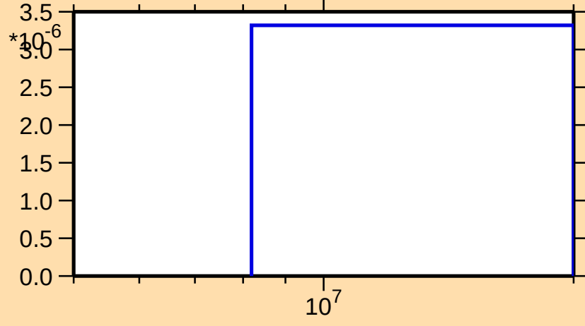
\sigma vs. E for ^{209}\text{Fr}(n,3n)
