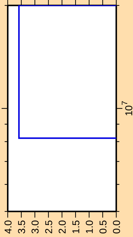
\Delta\sigma/\sigma vs. E for ^{209}\text{Fr}(\text{mt } 34)
