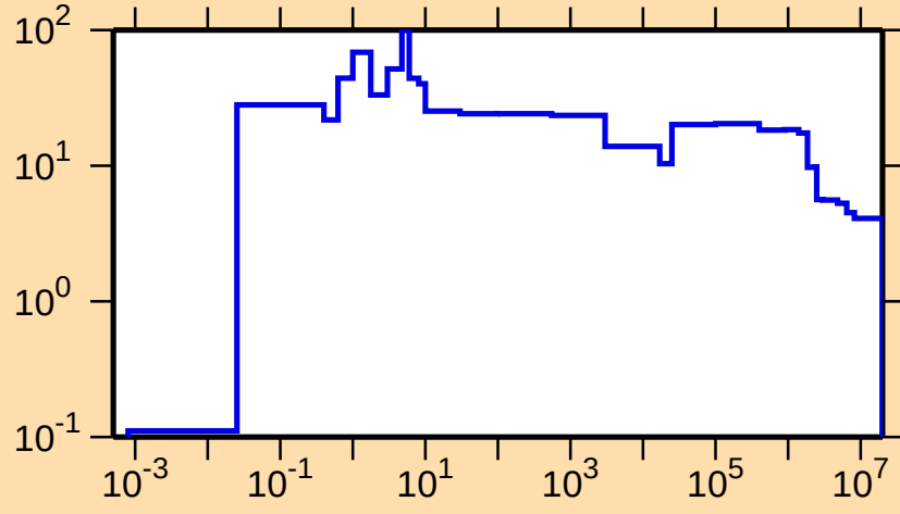
\Delta\sigma/\sigma vs. E for ^{209}\text{Fr}(n,\text{nonel.})
