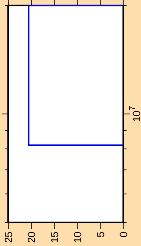
\Delta\sigma/\sigma vs. E for ^{209}\text{Fr}(n,2n)
