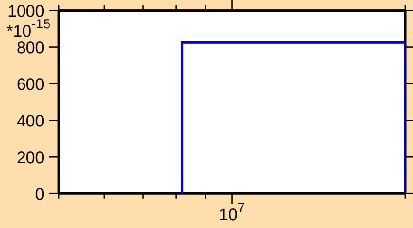
\sigma vs. E for ^{209}\text{Fr}(\text{mt } 34)
