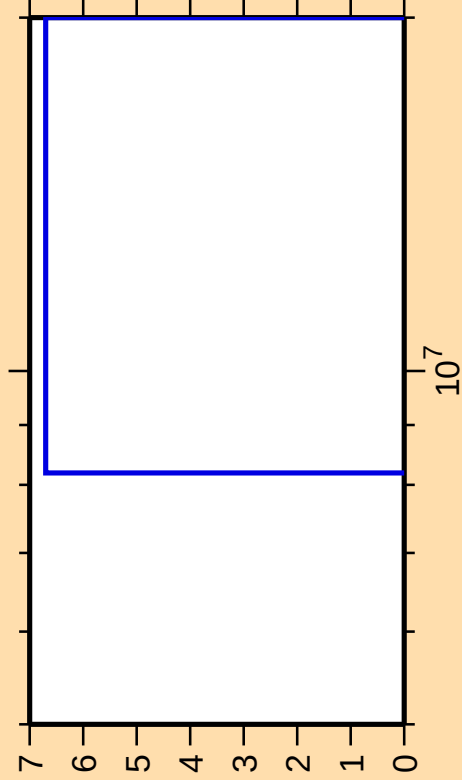
\Delta\sigma/\sigma vs. E for ^{209}\text{Fr}(n,\text{pt})
