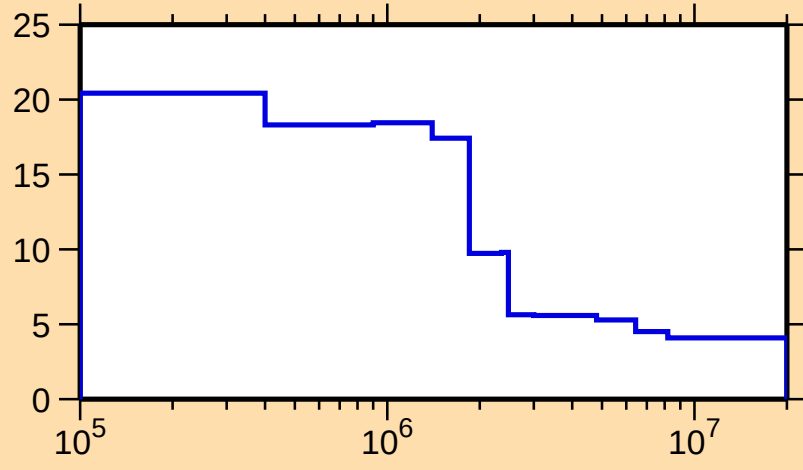
\Delta\sigma/\sigma vs. E for ^{209}\text{Fr}(n,\text{nonel.})
