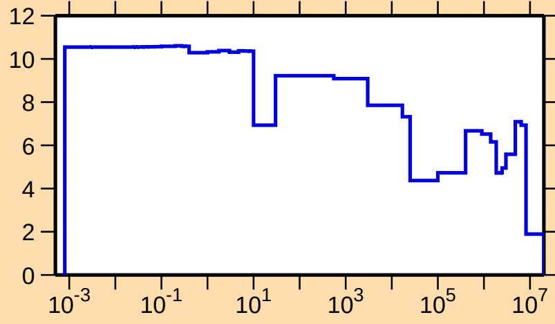
\Delta\sigma/\sigma vs. E for ^{209}\text{Fr}(n,\text{el.})
