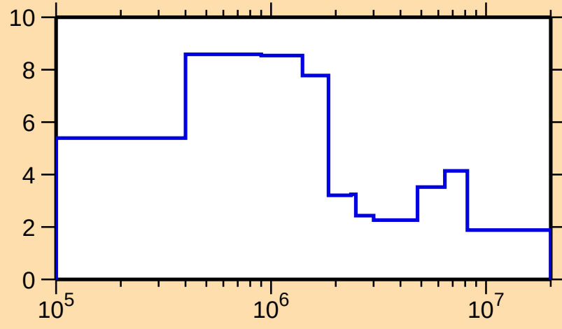
\Delta\sigma/\sigma vs. E for ^{209}\text{Fr}(n,\text{tot.})
