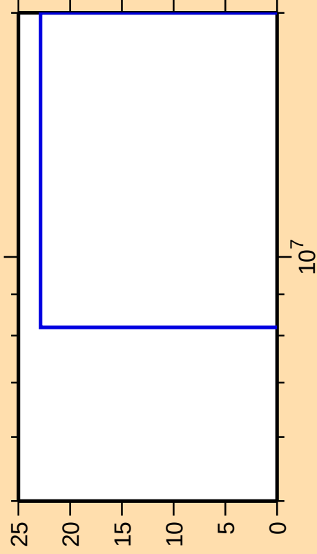
\Delta\sigma/\sigma vs. E for ^{209}\text{Fr}(n,n_1)
