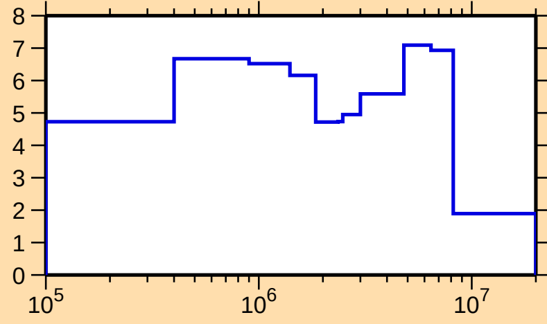
\Delta\sigma/\sigma vs. E for ^{209}\text{Fr}(n,\text{el.})
