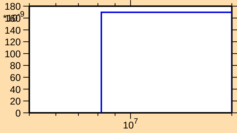
\sigma vs. E for ^{209}\text{Fr}(n,\text{nd})
