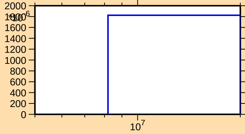
\sigma vs. E for ^{209}\text{Fr}(n,2n\alpha)
