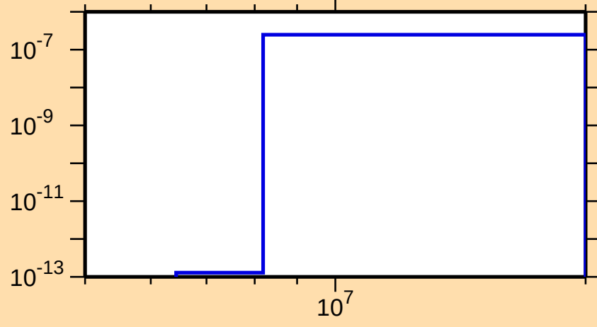
\sigma vs. E for ^{209}\text{Fr}(n,\text{He3})
