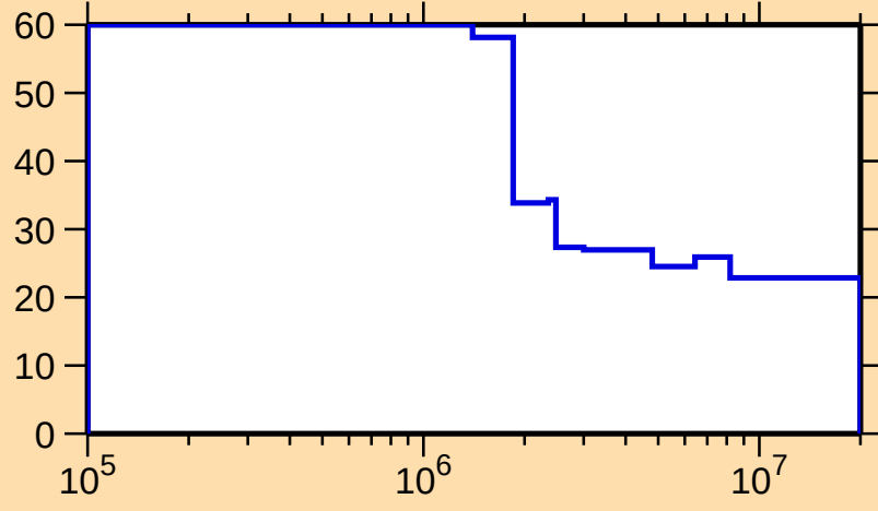
\Delta\sigma/\sigma vs. E for ^{209}\text{Fr}(n,n_1)
