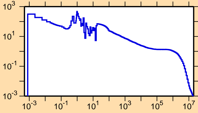
\sigma vs. E for ^{210}\text{Fr}(n,\gamma)
