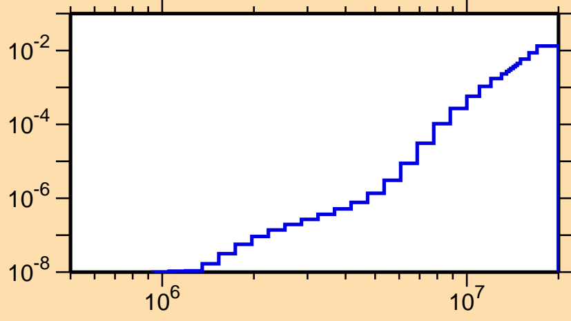
\sigma vs. E for ^{210}\text{Fr}(n,n\alpha)
