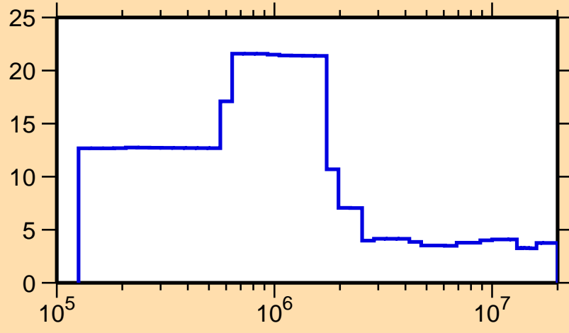
\Delta\sigma/\sigma vs. E for ^{210}\text{Fr}(n,\text{nonel.})
