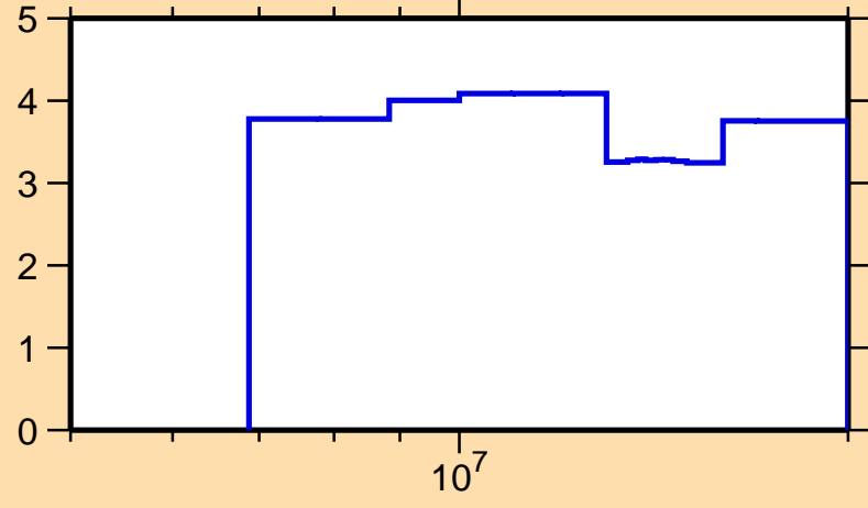
\Delta\sigma/\sigma vs. E for ^{210}\text{Fr}(n,\text{nonel.})
