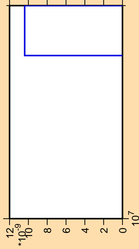
\Delta\sigma/\sigma vs. E for ^{210}\text{Fr}(\text{mt } 42)
