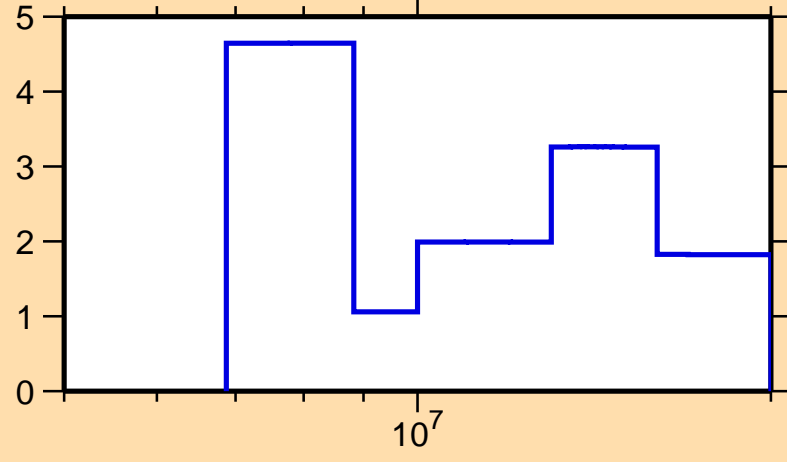
\Delta\sigma/\sigma vs. E for ^{210}\text{Fr}(n,\text{el.})
