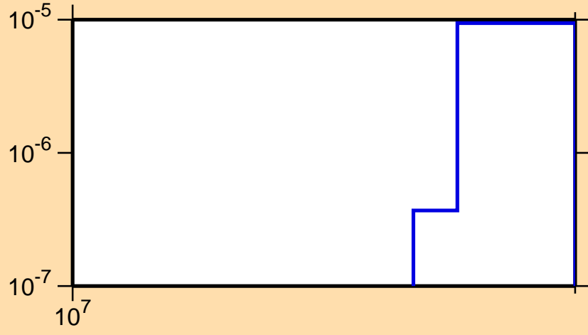
\sigma vs. E for ^{210}\text{Fr}(n,3n\alpha)
