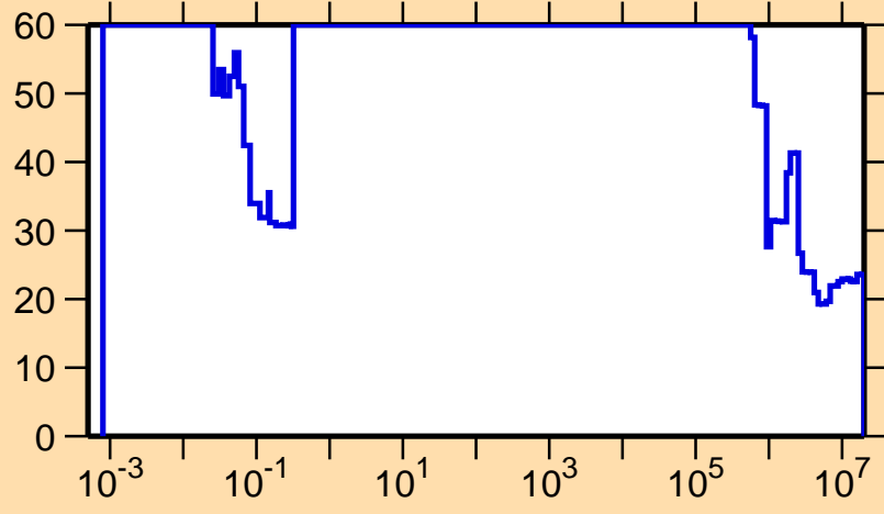
\Delta\sigma/\sigma vs. E for ^{210}\text{Fr}(n,p)
