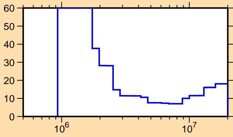
\Delta\sigma/\sigma vs. E for ^{210}\text{Fr}(n,n\text{cont.})
