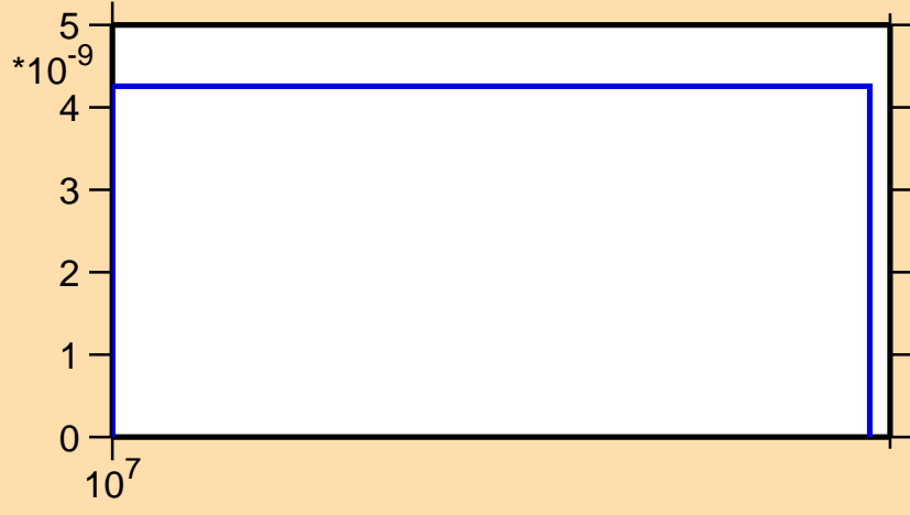
\sigma vs. E for ^{210}\text{Fr}(n,nt)
