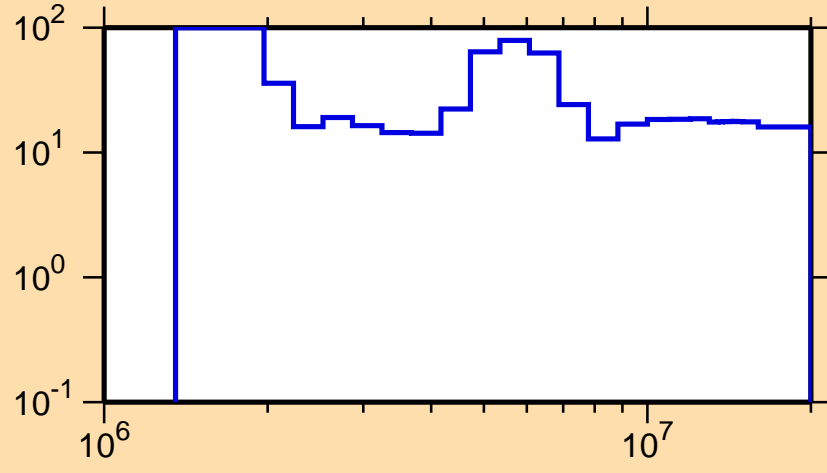
\Delta\sigma/\sigma vs. E for ^{211}\text{Fr}(n,n\text{cont.})
