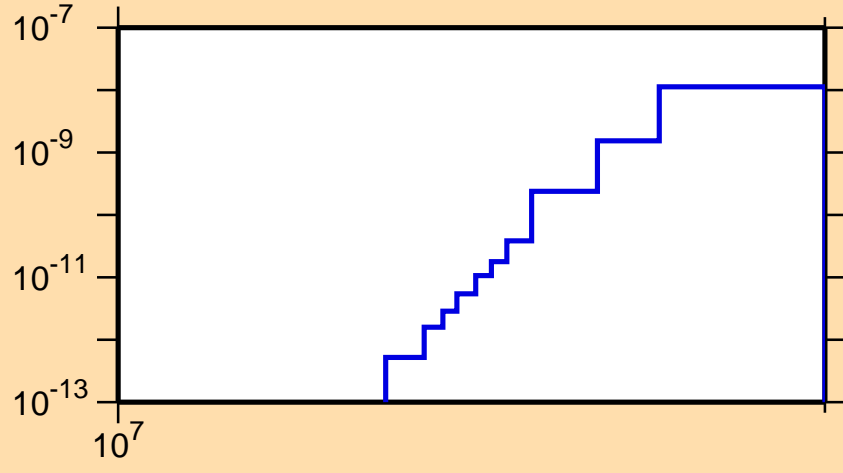
\sigma vs. E for ^{211}\text{Fr}(n,\text{pd})
