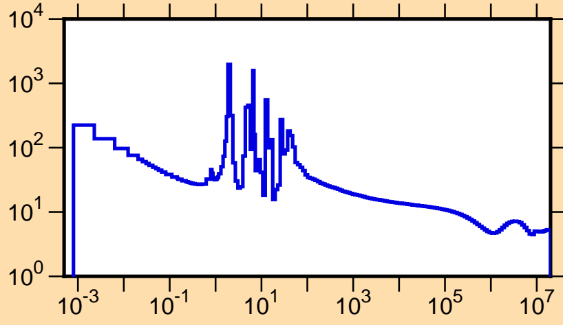
\sigma vs. E for ^{211}\text{Fr}(n,\text{tot.})
