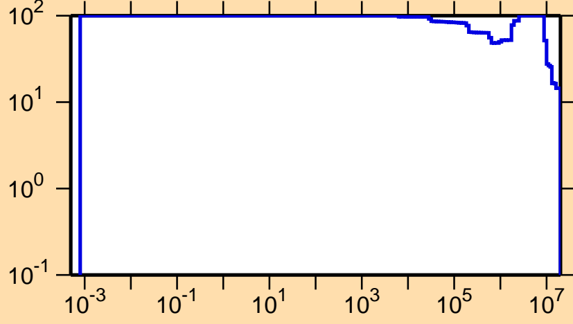
\Delta\sigma/\sigma vs. E for ^{211}\text{Fr}(n,p)
