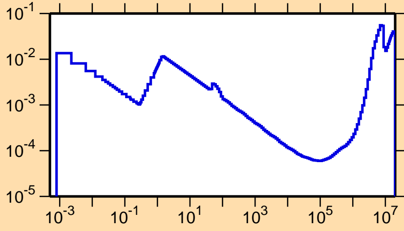
\sigma vs. E for ^{211}\text{Fr}(n,p)
