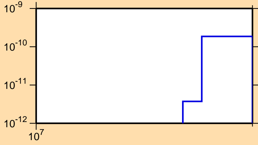
\sigma vs. E for ^{211}\text{Fr}(n,\text{pt})
