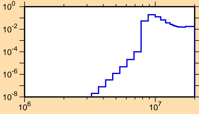
\sigma vs. E for ^{211}\text{Fr}(n,n\alpha)
