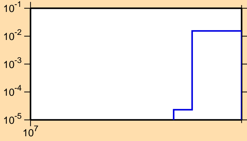
\sigma vs. E for ^{211}\text{Fr}(n,3n)
