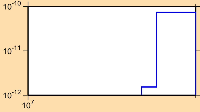
\sigma vs. E for ^{211}\text{Fr}(\text{mt } 34)
