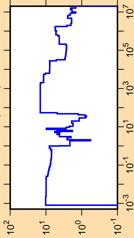
\Delta\sigma/\sigma vs. E for ^{211}\text{Fr}(n,\text{tot.})
