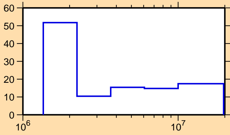
\Delta\sigma/\sigma vs. E for ^{211}\text{Fr}(n,n\text{cont.})
