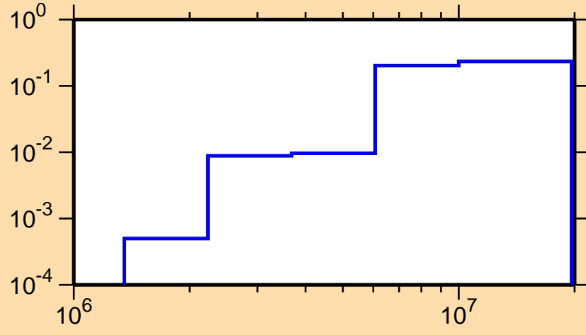
\sigma vs. E for ^{211}\text{Fr}(n,n\text{cont.})
