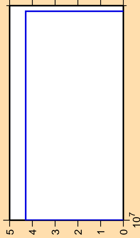
\Delta\sigma/\sigma vs. E for ^{211}\text{Fr}(\text{mt } 34)
