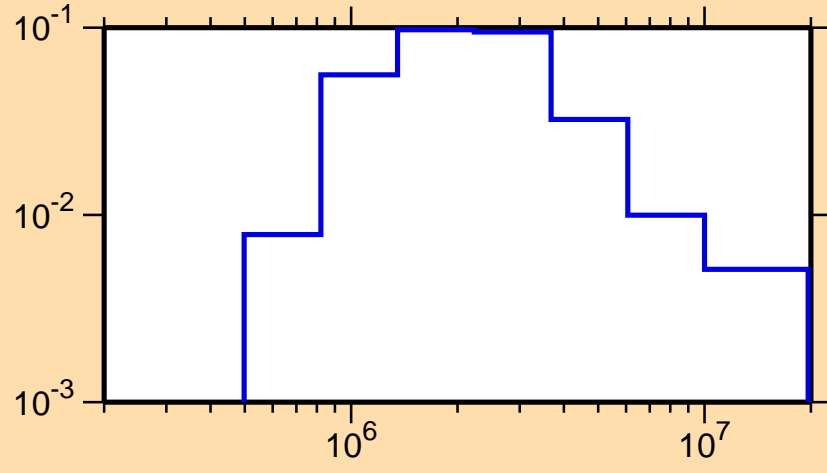
\sigma vs. E for ^{211}\text{Fr}(n,n_4)
