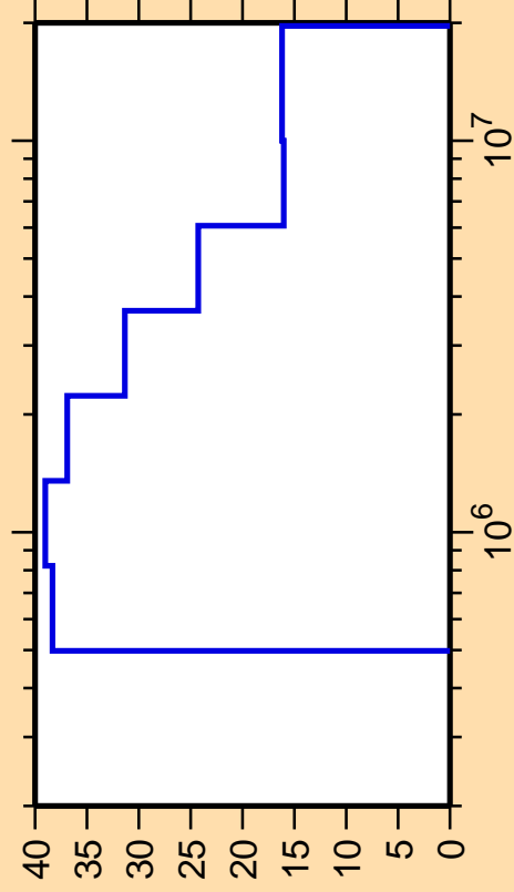
\Delta\sigma/\sigma vs. E for ^{211}\text{Fr}(n,n_4)
