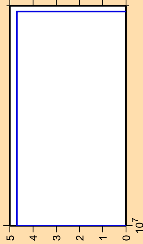
\Delta\sigma/\sigma vs. E for ^{211}\text{Fr}(n,\text{pt})
