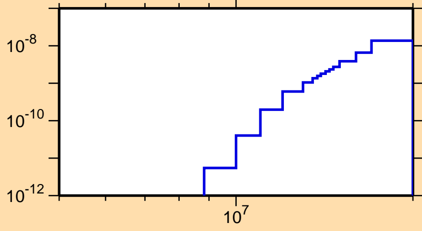
\sigma vs. E for ^{212}\text{Fr}(\text{mt117})
