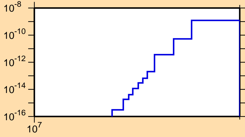
\sigma vs. E for ^{212}\text{Fr}(n,\text{pt})
