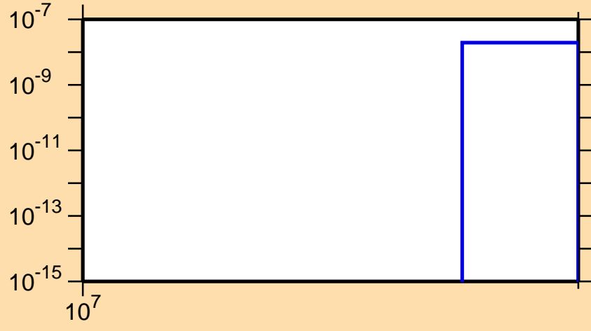
\sigma vs. E for ^{212}\text{Fr}(n,3n\alpha)
