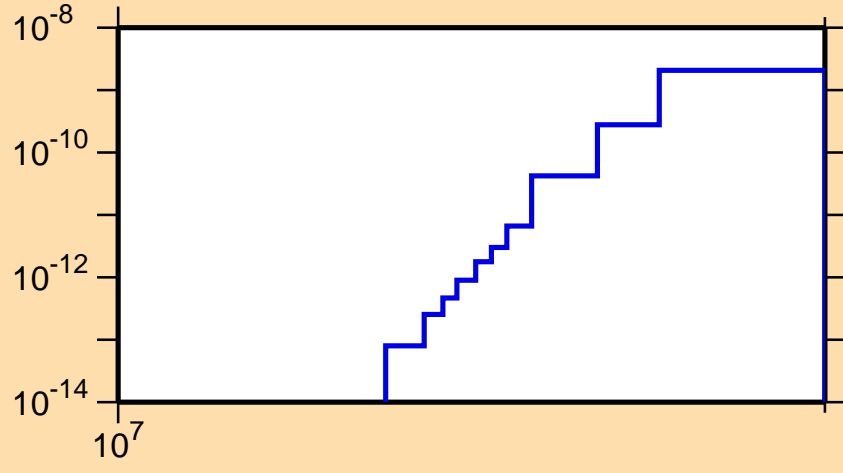
\sigma vs. E for ^{212}\text{Fr}(n,\text{pd})
