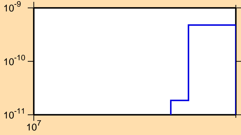
\sigma vs. E for ^{212}\text{Fr}(\text{mt } 34)
