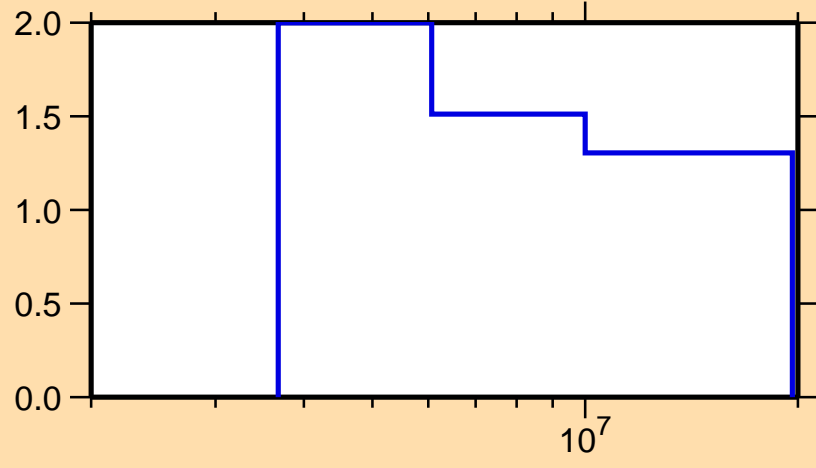
\Delta\sigma/\sigma vs. E for ^{212}\text{Fr}(n,n\text{nonel.})
