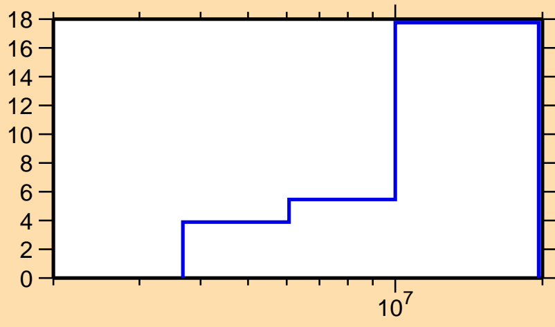
\Delta\sigma/\sigma vs. E for ^{212}\text{Fr}(n,n\text{cont.})
