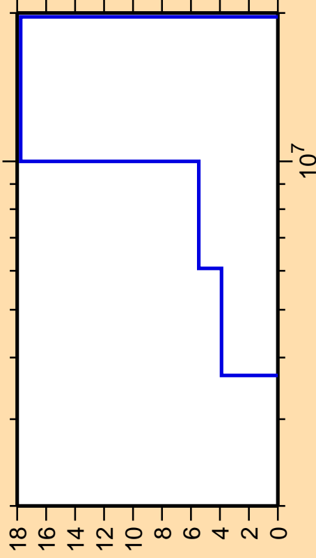
\Delta\sigma/\sigma vs. E for ^{212}\text{Fr}(n,n\text{cont.})
