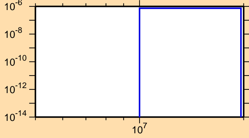
\sigma vs. E for ^{212}\text{Fr}(n,nd)
