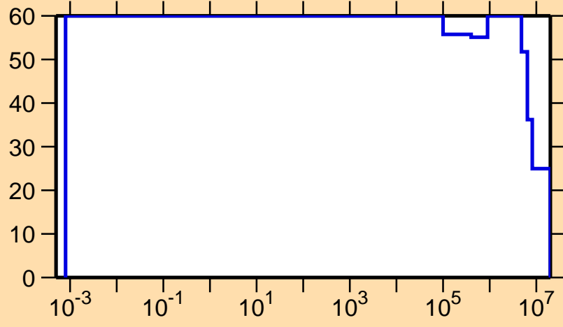
\Delta\sigma/\sigma vs. E for ^{212}\text{Fr}(n,p)
