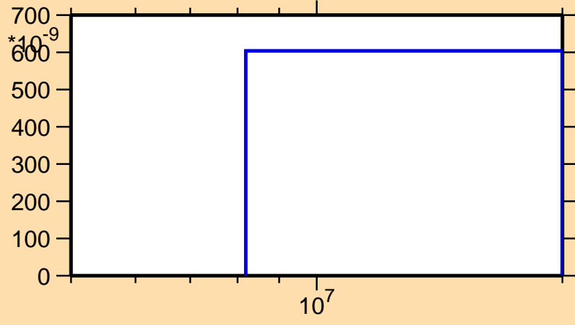
\sigma vs. E for ^{212}\text{Fr}(n,\text{nd})
