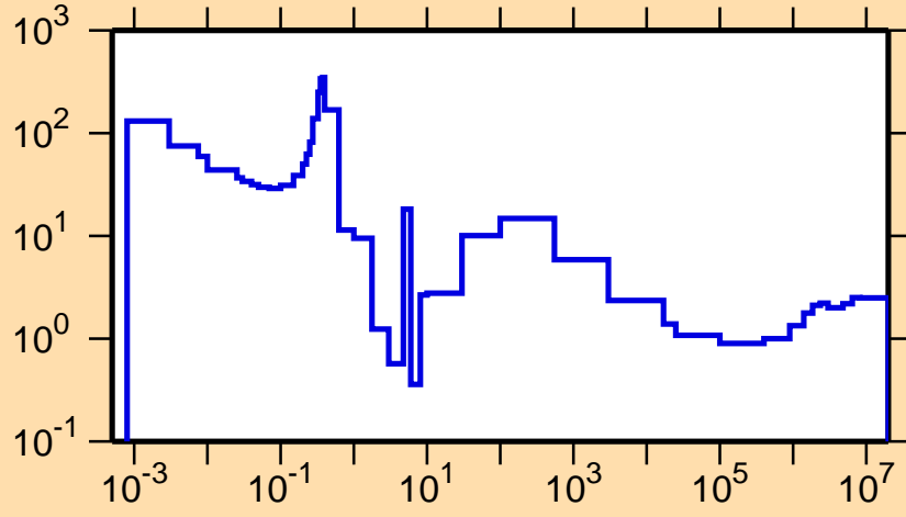
\sigma vs. E for ^{212}\text{Fr}(n,\text{nonel.})
