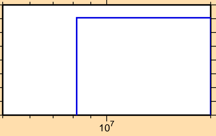
\sigma vs. E for ^{212}\text{Fr}(n,3n)
