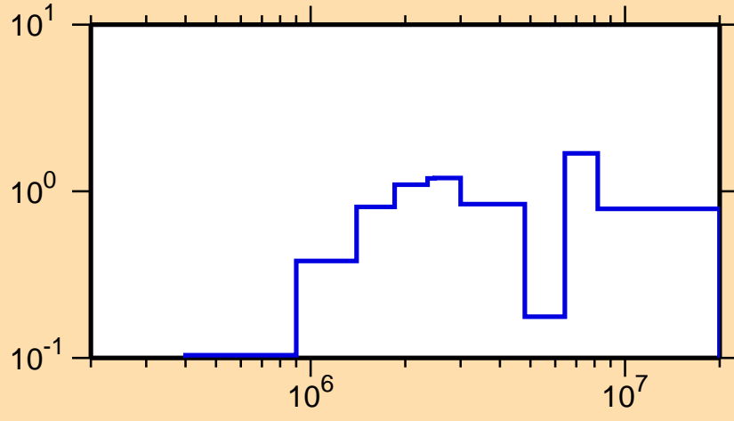
\sigma vs. E for ^{213}\text{Fr}(n,\text{inel.})
