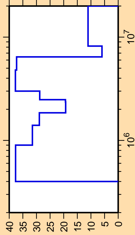
\Delta\sigma/\sigma vs. E for ^{213}\text{Fr}(n,\text{inel.})
