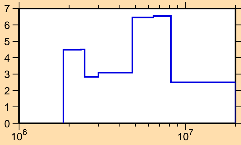
\Delta\sigma/\sigma vs. E for ^{213}\text{Fr}(n, el.)
