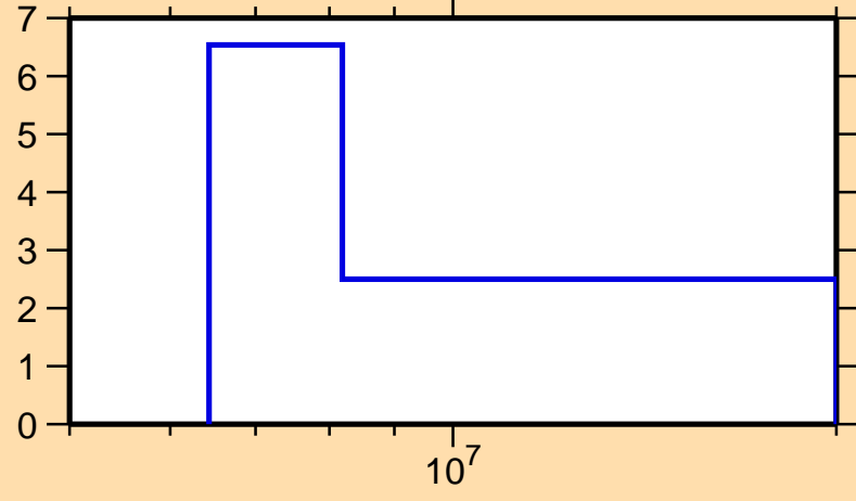
\Delta\sigma/\sigma vs. E for ^{213}\text{Fr}(n,\text{el.})
