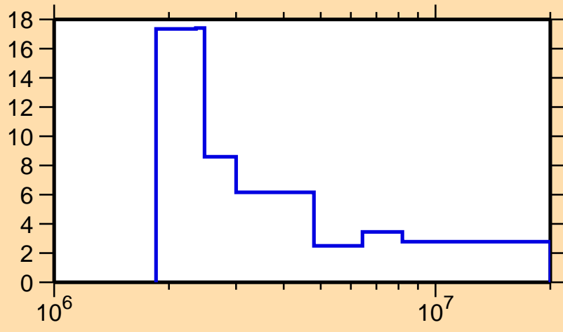
\Delta\sigma/\sigma vs. E for ^{213}\text{Fr}(n,\text{nonel.})
