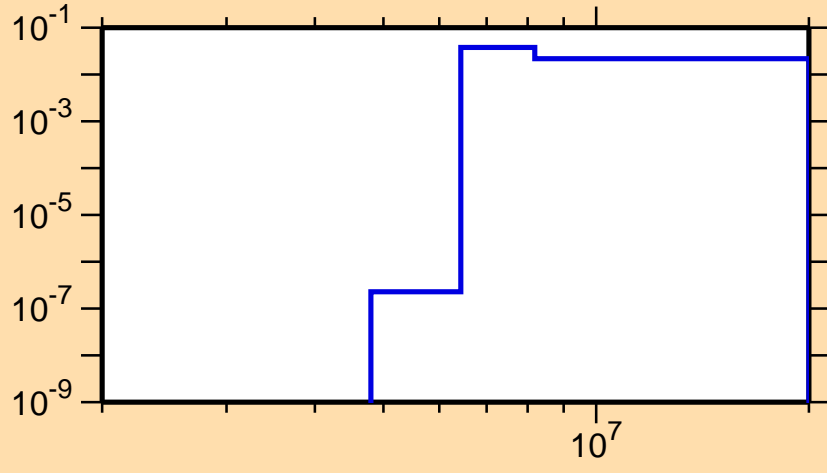
\sigma vs. E for ^{213}\text{Fr}(n,np)
