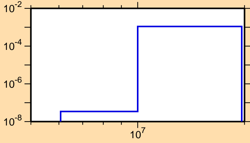
\sigma vs. E for ^{220}\text{Fr}(n,d)
