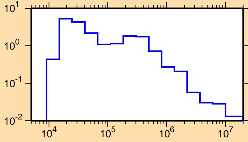
\sigma vs. E for ^{220}\text{Fr}(n,n_2)
