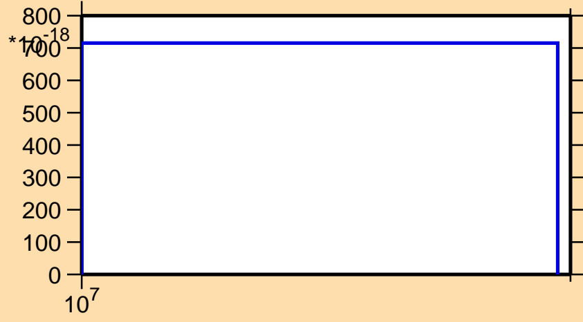
\sigma vs. E for ^{220}\text{Fr}(\text{mt } 42)
