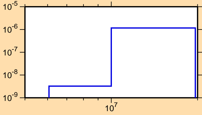
\sigma vs. E for ^{220}\text{Fr}(n,p\alpha)
