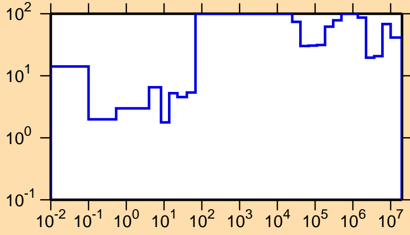
\Delta\sigma/\sigma vs. E for ^{220}\text{Fr}(n,el.)
