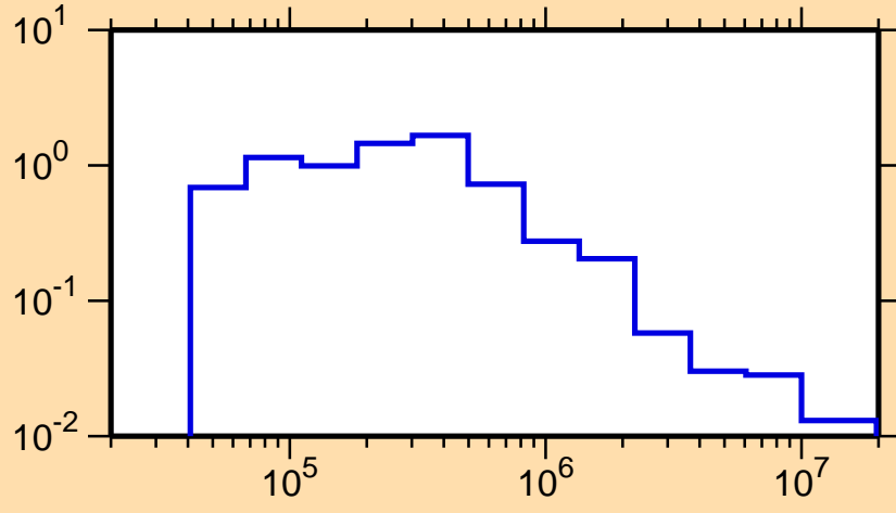
\sigma vs. E for ^{220}\text{Fr}(n,n_4)
