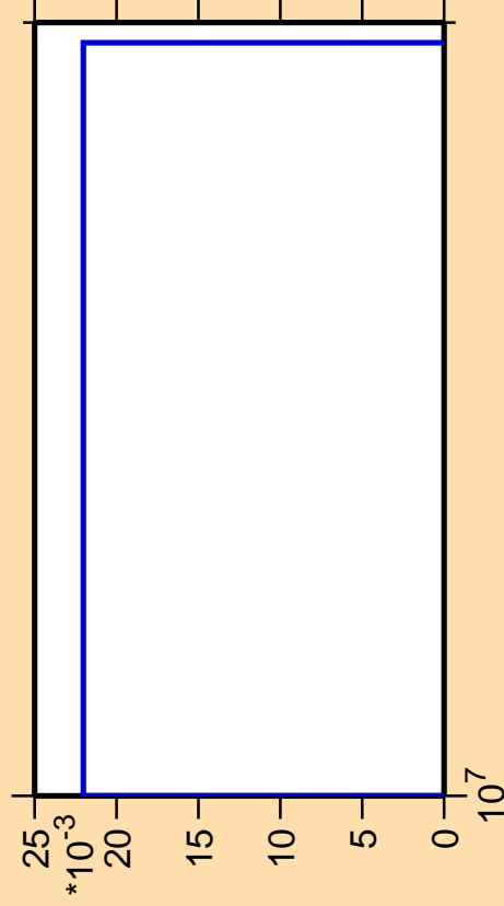
\Delta\sigma/\sigma vs. E for ^{220}\text{Fr} (mt 11)
