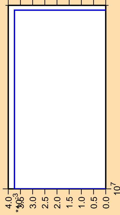
\Delta\sigma/\sigma vs. E for ^{220}\text{Fr}(\text{mt } 42)
