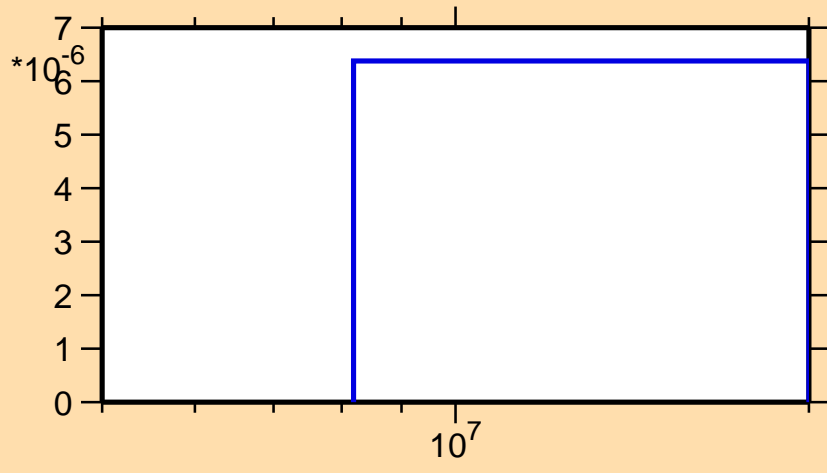
\sigma vs. E for ^{220}\text{Fr}(n,nt)
