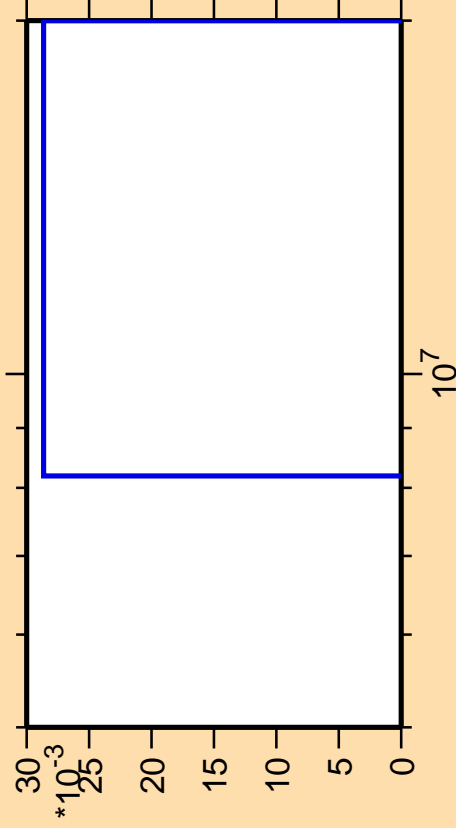
\Delta\sigma/\sigma vs. E for ^{220}\text{Fr}(\text{mt } 11)
