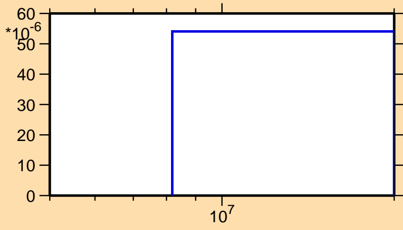
\sigma vs. E for ^{220}\text{Fr}(\text{mt117})
