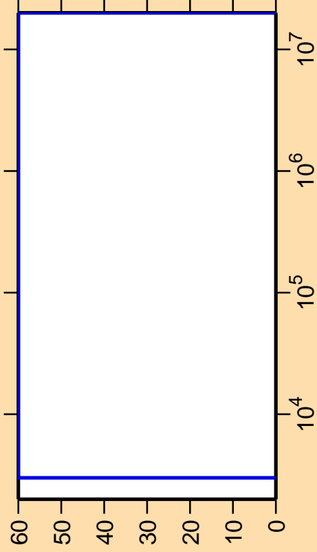
\Delta\sigma/\sigma vs. E for ^{220}\text{Fr}(n,n_2)
