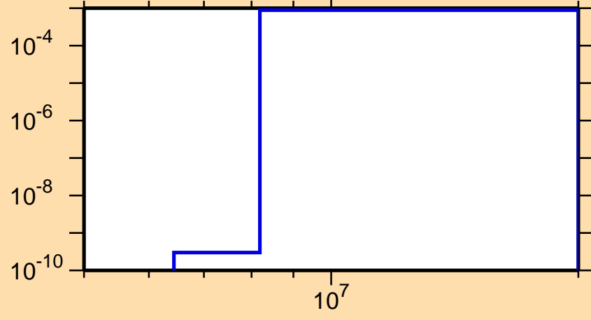
\sigma vs. E for ^{220}\text{Fr}(n,d)
