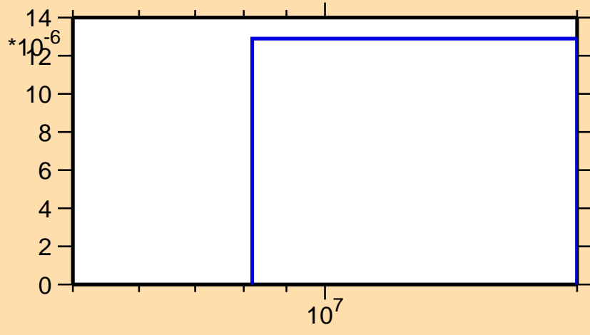
\sigma vs. E for ^{220}\text{Fr}(\text{mt } 45)
