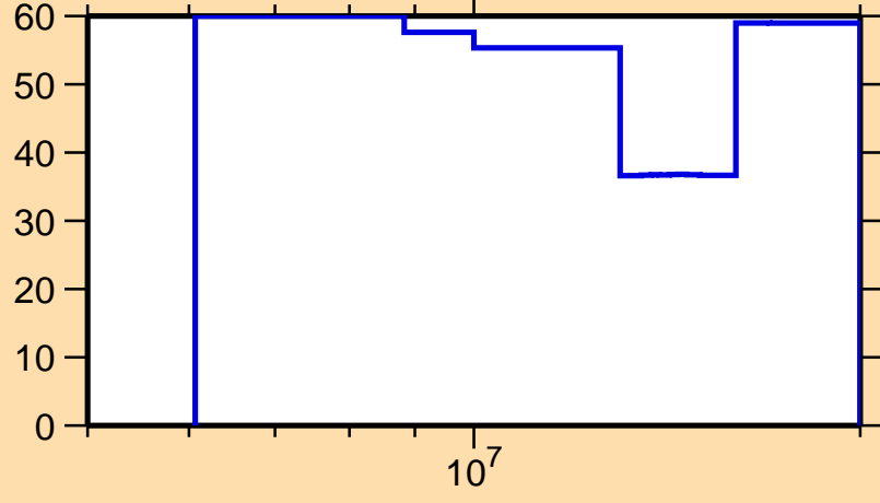
\Delta\sigma/\sigma vs. E for ^{221}\text{Fr}(n,2n)
