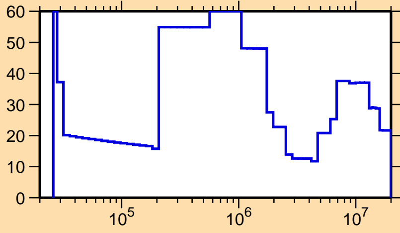
\Delta\sigma/\sigma vs. E for ^{221}\text{Fr}(n,\text{tot.})
