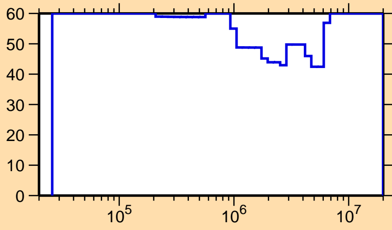
\Delta\sigma/\sigma vs. E for ^{221}\text{Fr}(n,\text{inel.})
