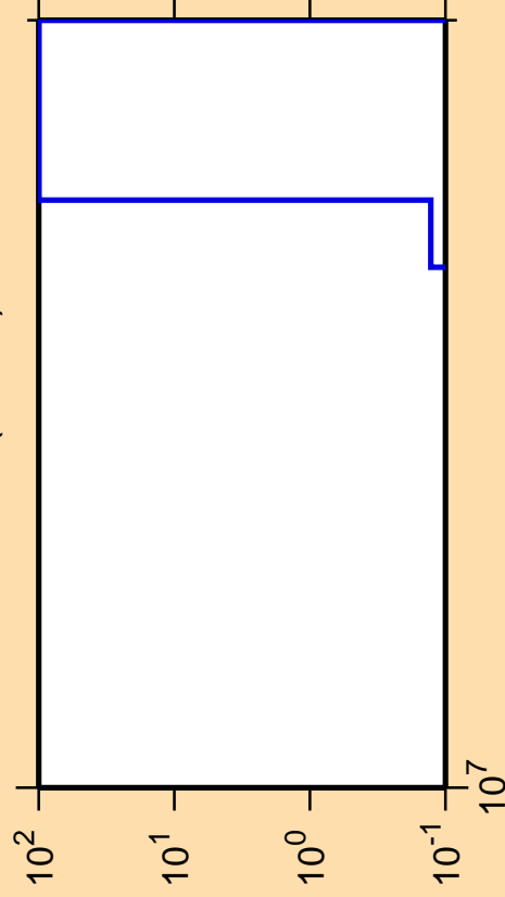
\Delta\sigma/\sigma vs. E for ^{221}\text{Fr}(\text{mt 11})
