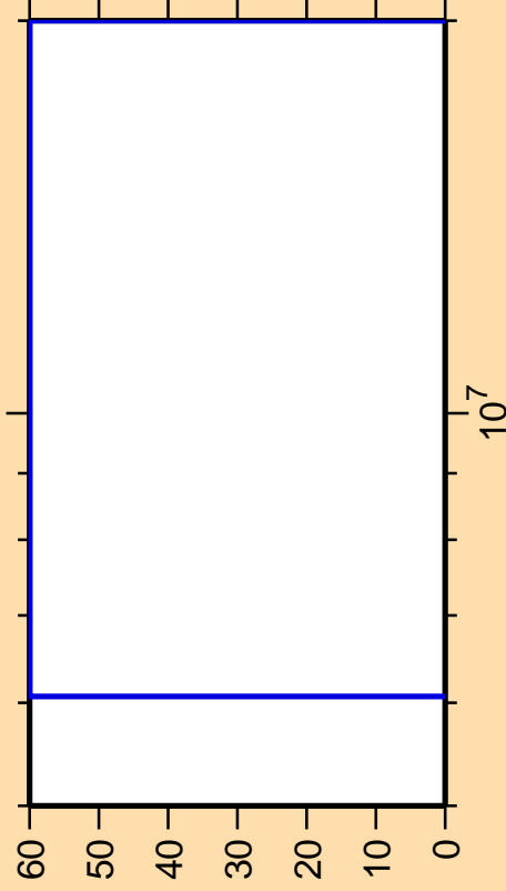
\Delta\sigma/\sigma vs. E for ^{221}\text{Fr}(n,n\text{cont.})
