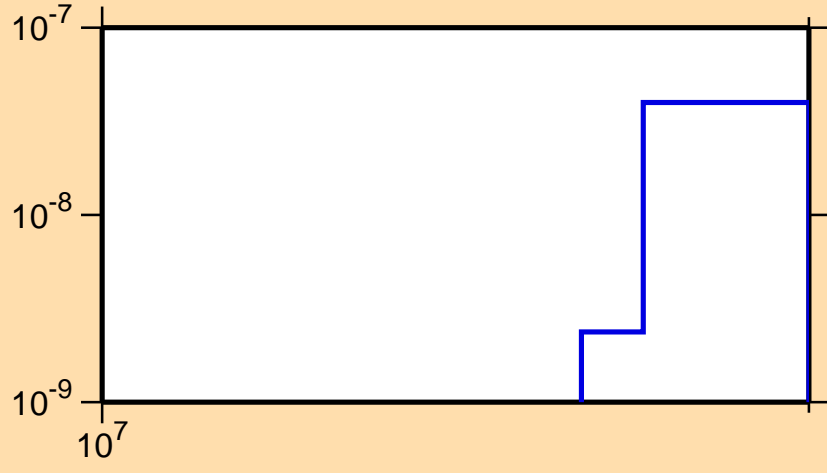
\sigma vs. E for ^{221}\text{Fr}(n,\text{He3})
