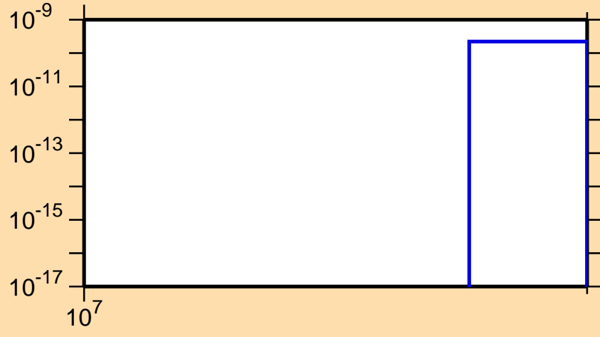
\sigma vs. E for ^{221}\text{Fr}(\text{mt } 42)
