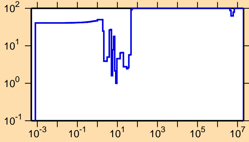
\Delta\sigma/\sigma vs. E for ^{221}\text{Fr}(n,\gamma)
