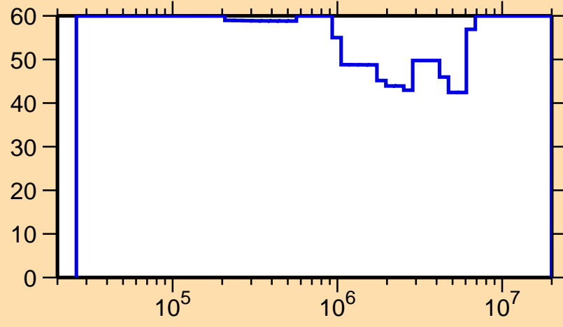
\Delta\sigma/\sigma vs. E for ^{221}\text{Fr}(n,\text{inel.})
