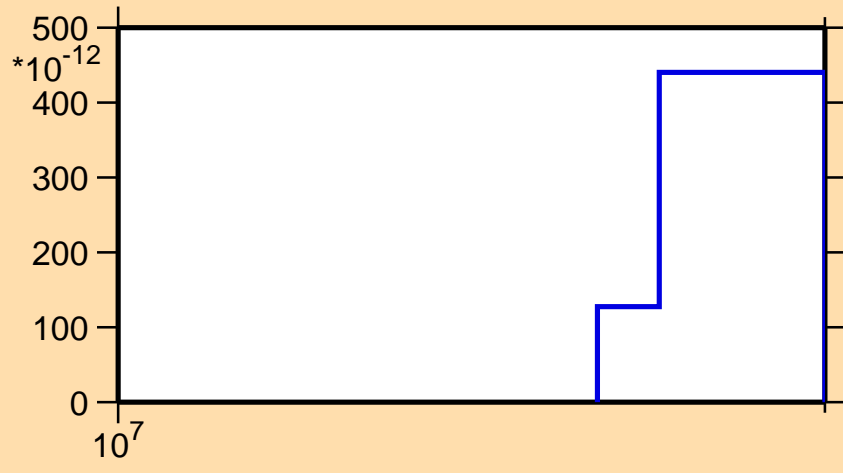
\sigma vs. E for ^{221}\text{Fr}(\text{mt } 45)
