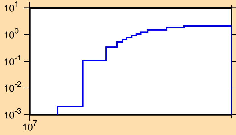
\sigma vs. E for ^{221}\text{Fr}(n,3n)
