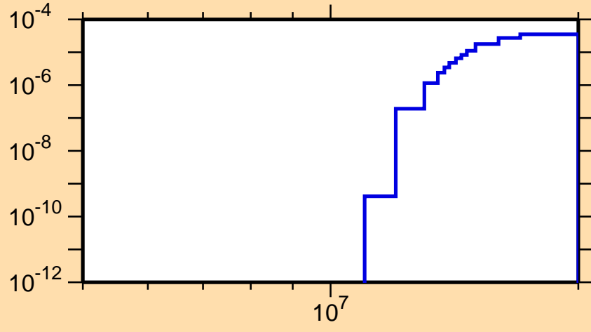
\sigma vs. E for ^{221}\text{Fr}(n,3n\alpha)
