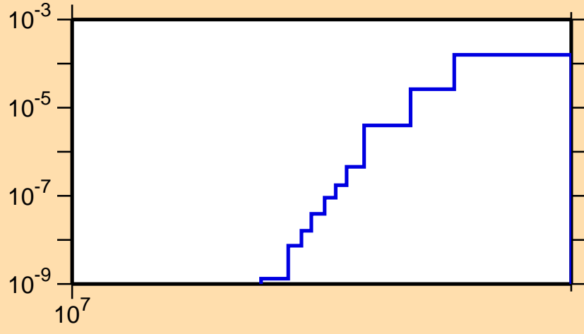
\sigma vs. E for ^{221}\text{Fr}(n,\text{nd})
