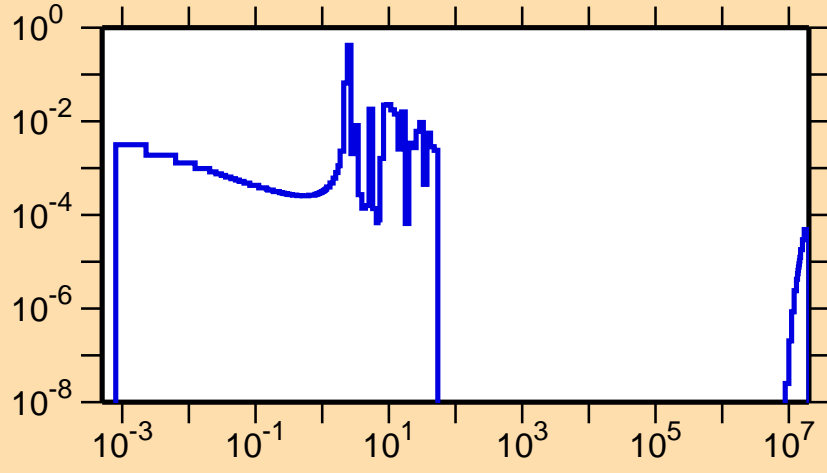
\sigma vs. E for ^{221}\text{Fr}(n,f)
