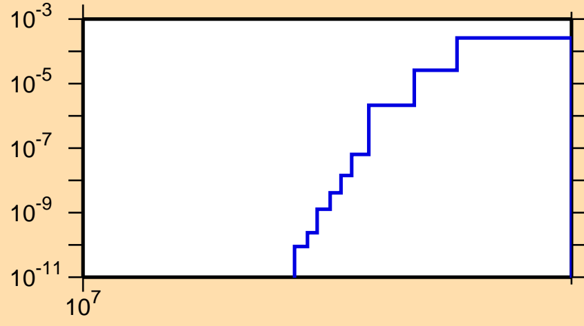
\sigma vs. E for ^{221}\text{Fr}(n,2np)
