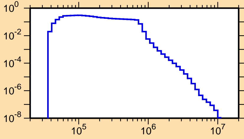
\sigma vs. E for ^{221}\text{Fr}(n,n_2)
