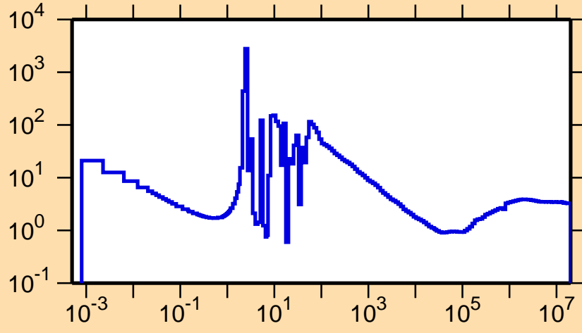
\sigma vs. E for ^{221}\text{Fr}(n,\text{nonel.})
