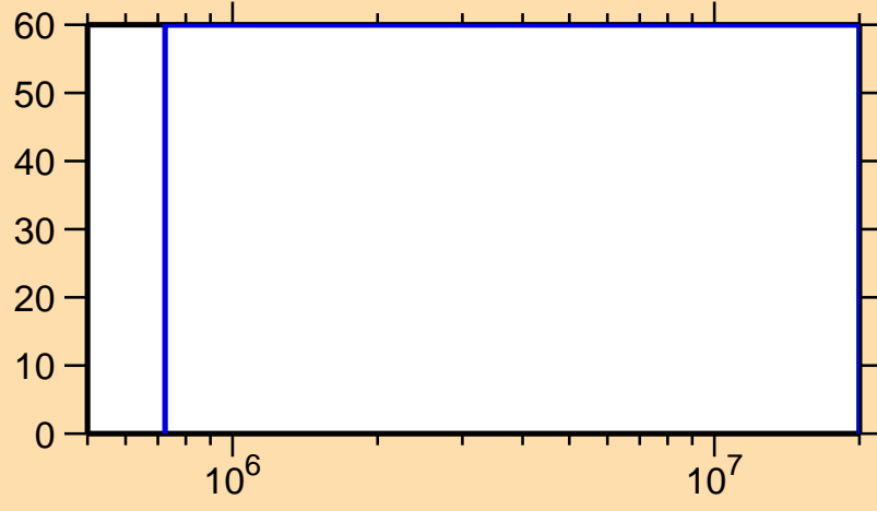
\Delta\sigma/\sigma vs. E for ^{221}\text{Fr}(n,n\text{cont.})
