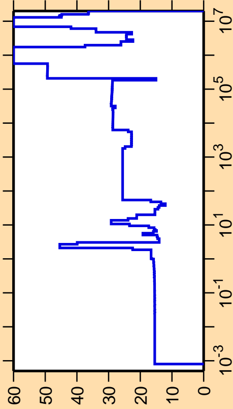
\Delta\sigma/\sigma vs. E for ^{221}\text{Fr}(n,\text{el.})
