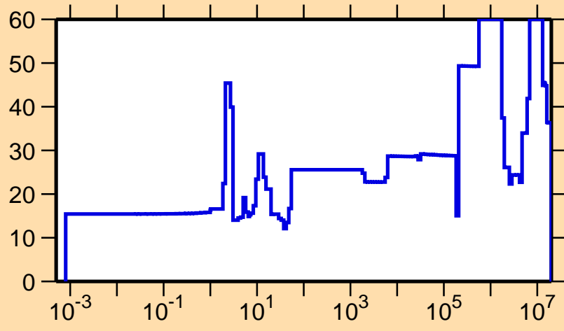
\Delta\sigma/\sigma vs. E for ^{221}\text{Fr}(n,\text{el.})
