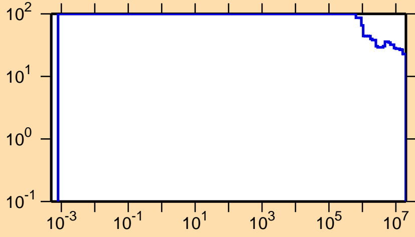
\Delta\sigma/\sigma vs. E for ^{221}\text{Fr}(n,\text{nonel.})
