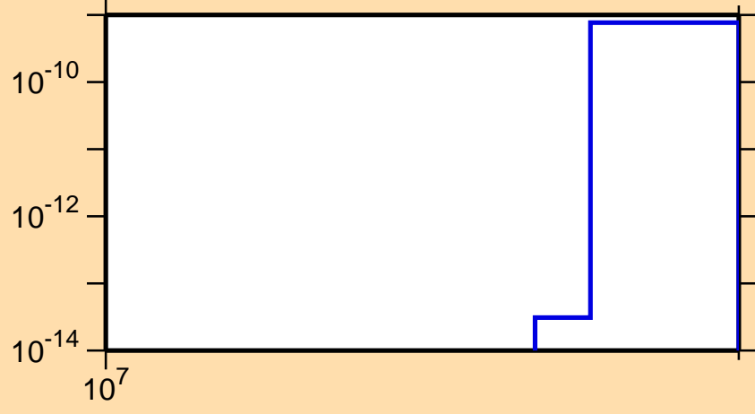
\sigma vs. E for ^{221}\text{Fr}(\text{mt 11})
