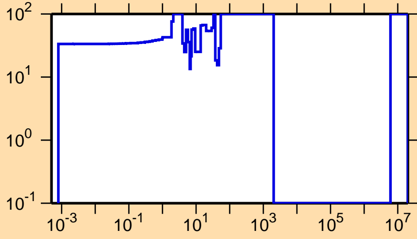
\Delta\sigma/\sigma vs. E for ^{221}\text{Fr}(n,f)
