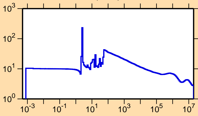
\sigma vs. E for ^{221}\text{Fr}(n,\text{el.})
