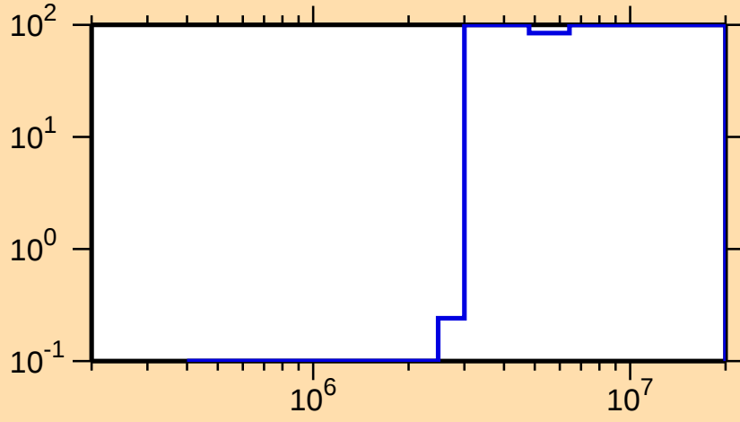
\Delta\sigma/\sigma vs. E for ^{222}\text{Fr}(n,\text{f})
