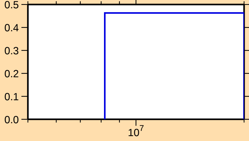
\sigma vs. E for ^{222}\text{Fr}(n,3n)
