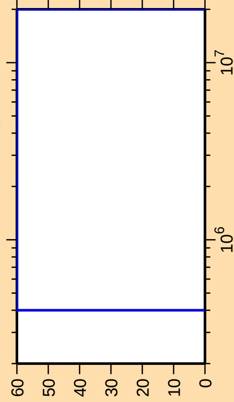
\Delta\sigma/\sigma vs. E for ^{222}\text{Fr}(n,n_{\text{cont.}})
