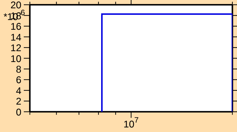
\sigma vs. E for ^{222}\text{Fr}(n,nt)
