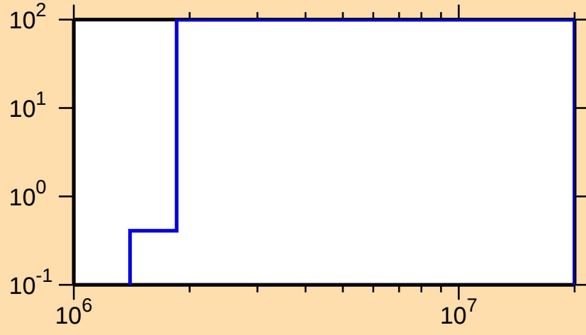
\Delta\sigma/\sigma vs. E for ^{222}\text{Fr}(n,p)
