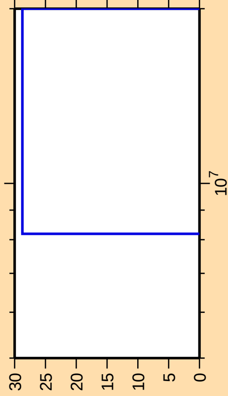
\Delta\sigma/\sigma vs. E for ^{222}\text{Fr}(\text{mt } 11)
