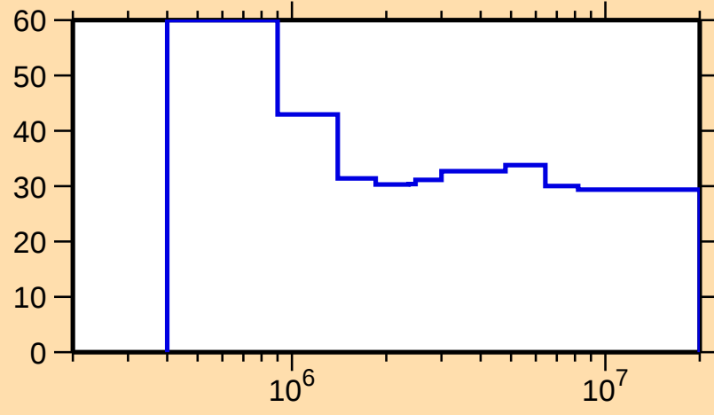
\Delta\sigma/\sigma vs. E for ^{222}\text{Fr}(n,\text{nonel.})
