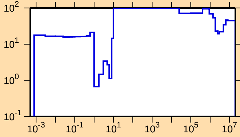
\Delta\sigma/\sigma vs. E for ^{222}\text{Fr}(n,\text{tot.})
