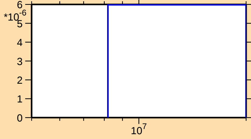
\sigma vs. E for ^{222}\text{Fr}(n,p\alpha)
