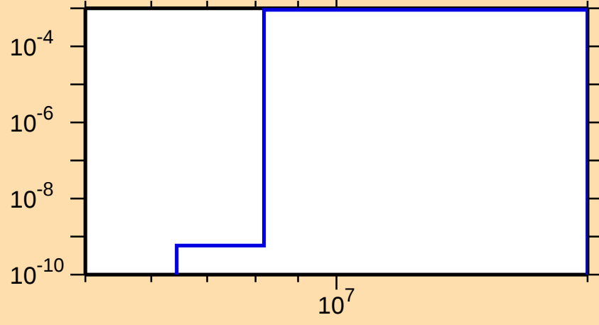
\sigma vs. E for ^{222}\text{Fr}(n,t)
