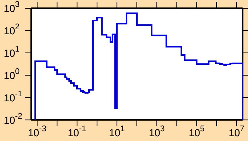
\sigma vs. E for ^{222}\text{Fr}(n,\text{nonel.})
