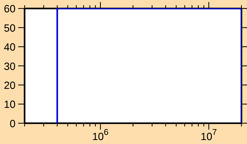
\Delta\sigma/\sigma vs. E for ^{222}\text{Fr}(n,n\text{cont.})
