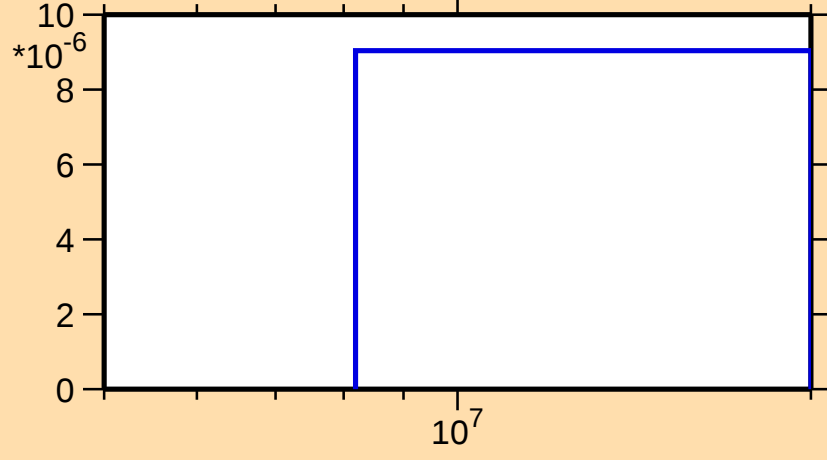
\sigma vs. E for ^{222}\text{Fr}(n,\text{nd})
