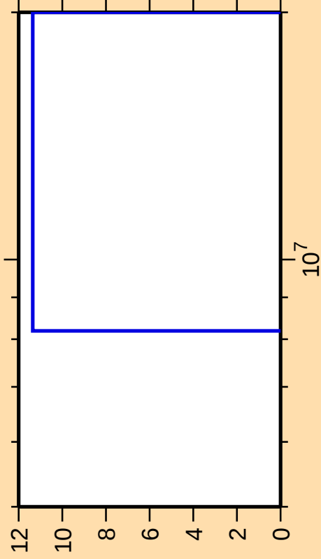
\Delta\sigma/\sigma vs. E for ^{222}\text{Fr}(\text{mt } 42)
