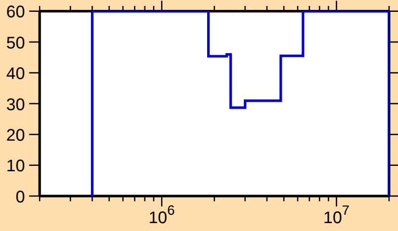
\Delta\sigma/\sigma vs. E for ^{222}\text{Fr}(n,\text{el.})
