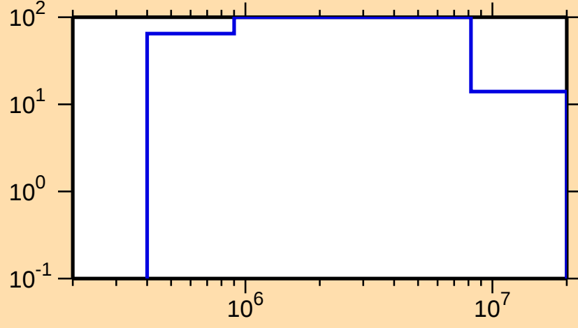
\Delta\sigma/\sigma vs. E for ^{222}\text{Fr}(n,n_1)
