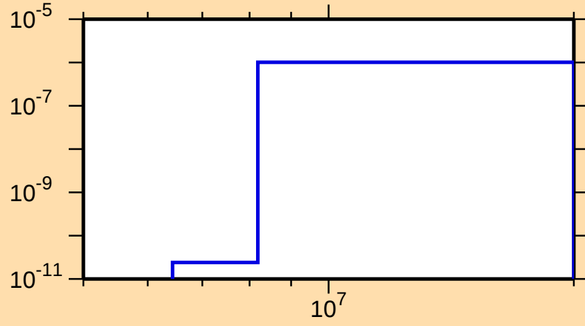
\sigma vs. E for ^{222}\text{Fr}(n,2n\alpha)
