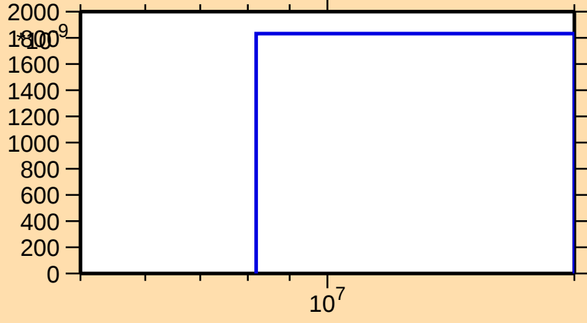
\sigma vs. E for ^{222}\text{Fr}(n,2np)
