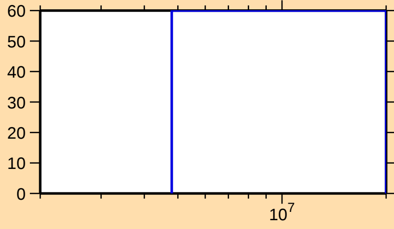
\Delta\sigma/\sigma vs. E for ^{222}\text{Fr}(n,2n)
