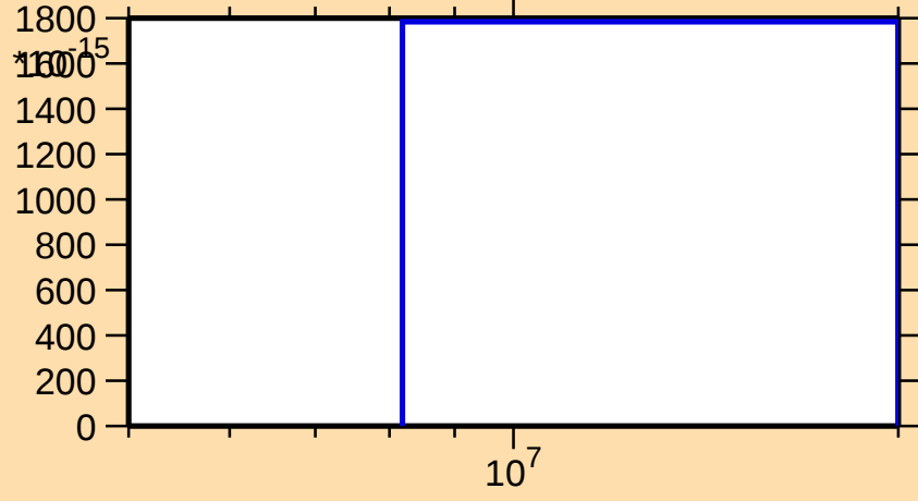
\sigma vs. E for ^{222}\text{Fr}(\text{mt } 42)
