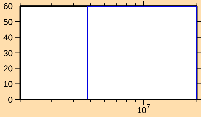
\Delta\sigma/\sigma vs. E for ^{222}\text{Fr}(n,\text{inel.})
