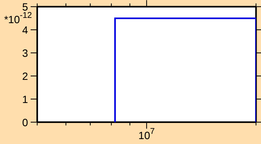
\sigma vs. E for ^{222}\text{Fr}(\text{mt } 11)
