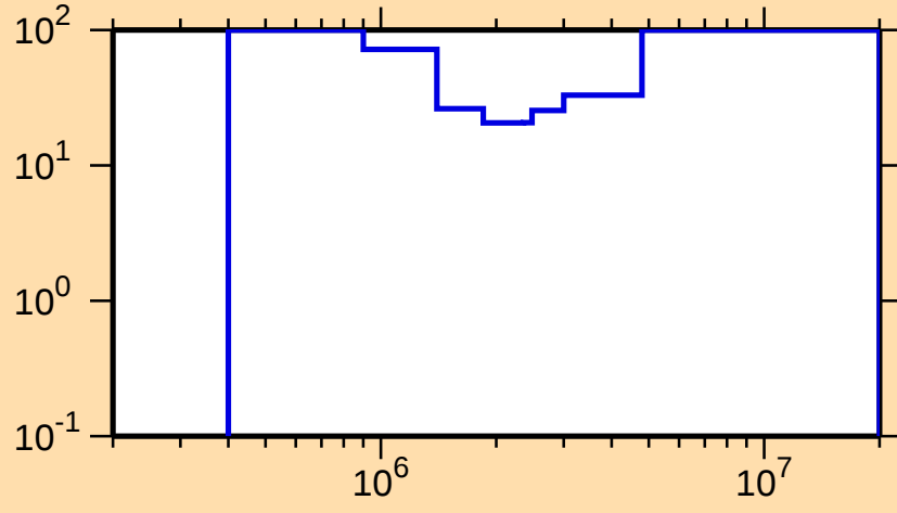
\Delta\sigma/\sigma vs. E for ^{222}\text{Fr}(n,\text{inel.})
