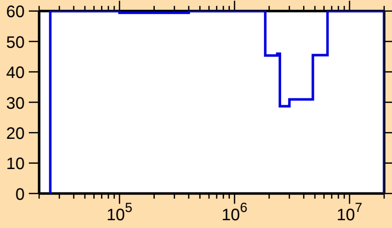
\Delta\sigma/\sigma vs. E for ^{222}\text{Fr}(n,\text{el.})
