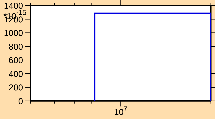
\sigma vs. E for ^{222}\text{Fr}(\text{mt } 45)
