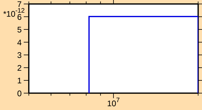
\sigma vs. E for ^{222}\text{Fr}(\text{mt117})
