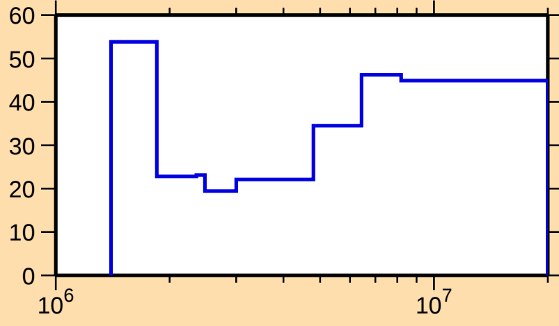
\Delta\sigma/\sigma vs. E for ^{222}\text{Fr}(n,\text{tot.})
