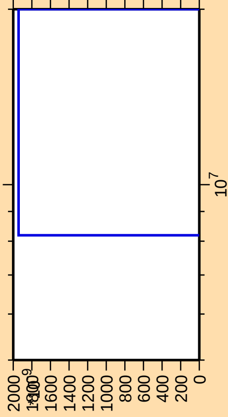
\Delta\sigma/\sigma vs. E for ^{222}\text{Fr}(\text{mt } 34)
