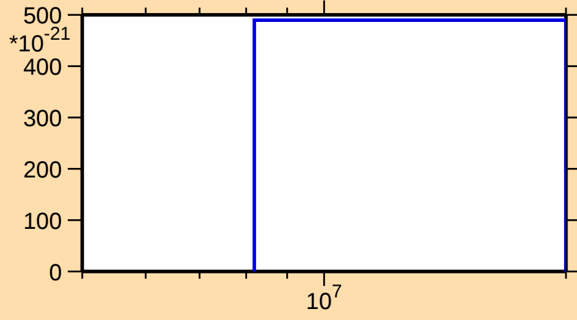
\sigma vs. E for ^{222}\text{Fr}(\text{mt } 34)
