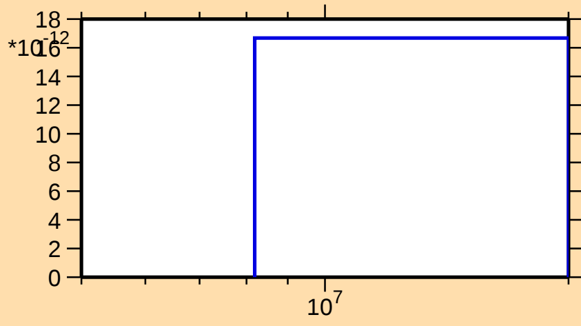
\sigma vs. E for ^{222}\text{Fr}(n,\text{He3})
