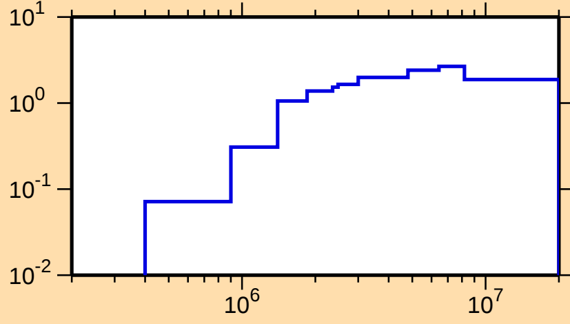
\sigma vs. E for ^{222}\text{Fr}(n,n\text{cont.})
