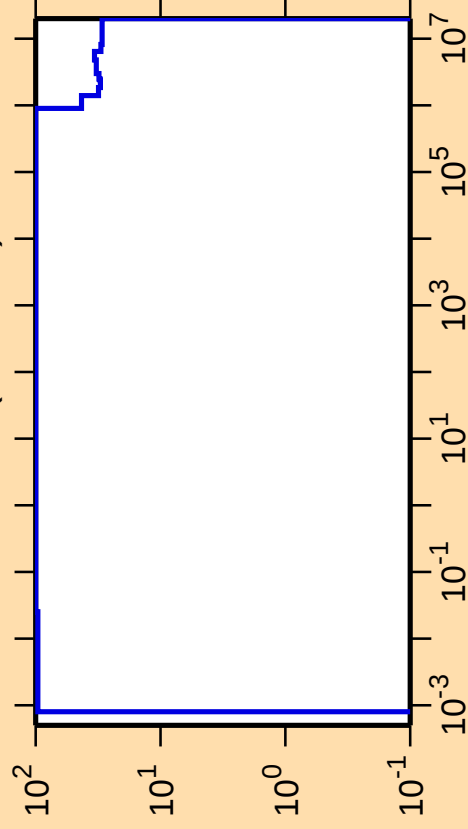
\Delta\sigma/\sigma vs. E for ^{222}\text{Fr}(n,\text{nonel.})
