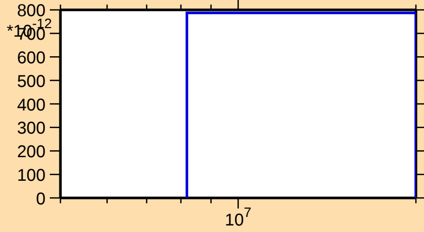
\sigma vs. E for ^{222}\text{Fr}(n,3n\alpha)
