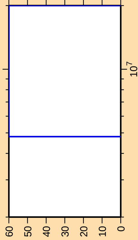
\Delta\sigma/\sigma vs. E for ^{222}\text{Fr}(n,\gamma)
