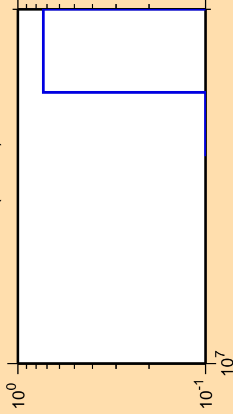
\Delta\sigma/\sigma vs. E for ^{223}\text{Fr} (mt 42)
