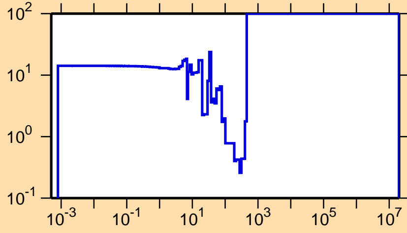
\Delta\sigma/\sigma vs. E for ^{223}\text{Fr}(n,\gamma)
