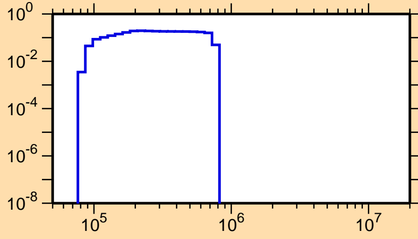
\sigma vs. E for ^{223}\text{Fr}(n,n_3)
