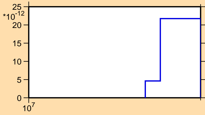
\sigma vs. E for ^{223}\text{Fr}(\text{mt117})
