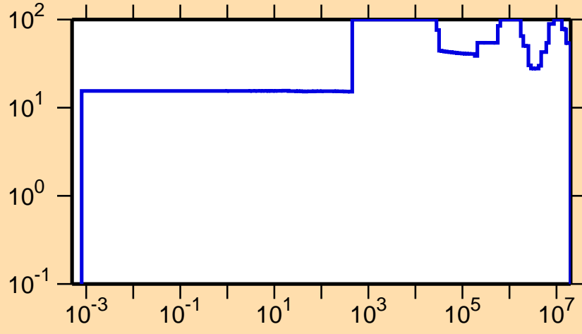
\Delta\sigma/\sigma vs. E for ^{223}\text{Fr}(n,el.)
