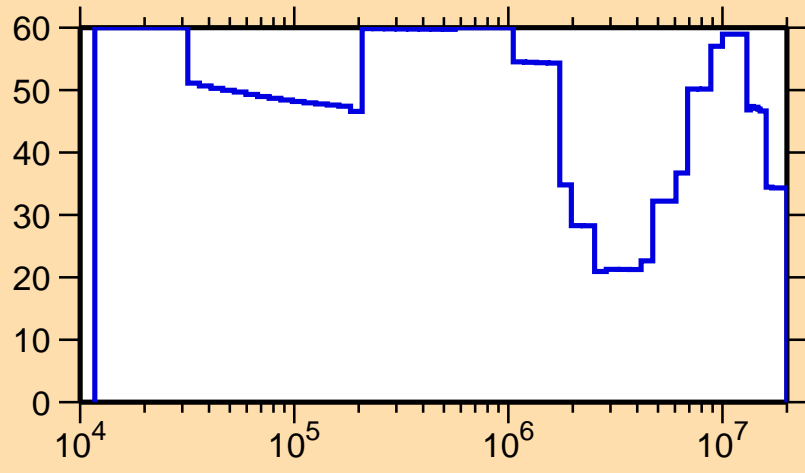
\Delta\sigma/\sigma vs. E for ^{223}\text{Fr}(n,\text{tot.})
