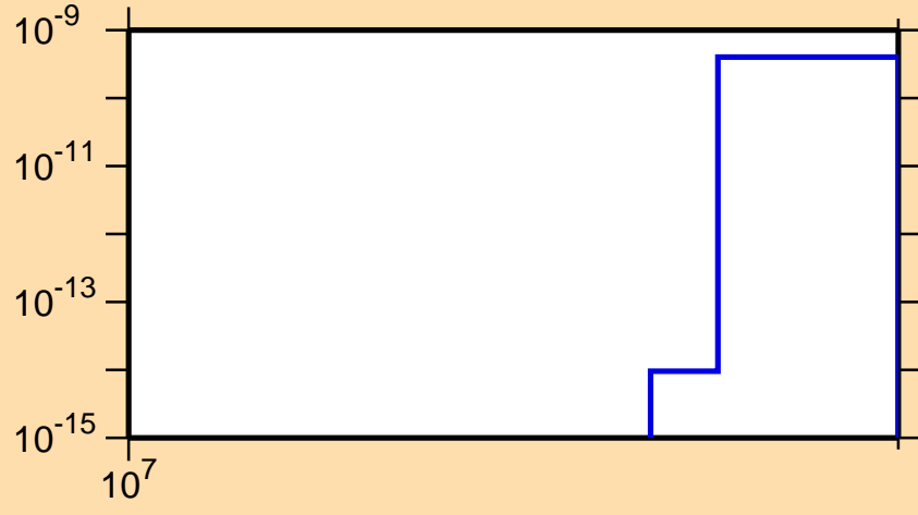
\sigma vs. E for ^{223}\text{Fr}(\text{mt } 11)
