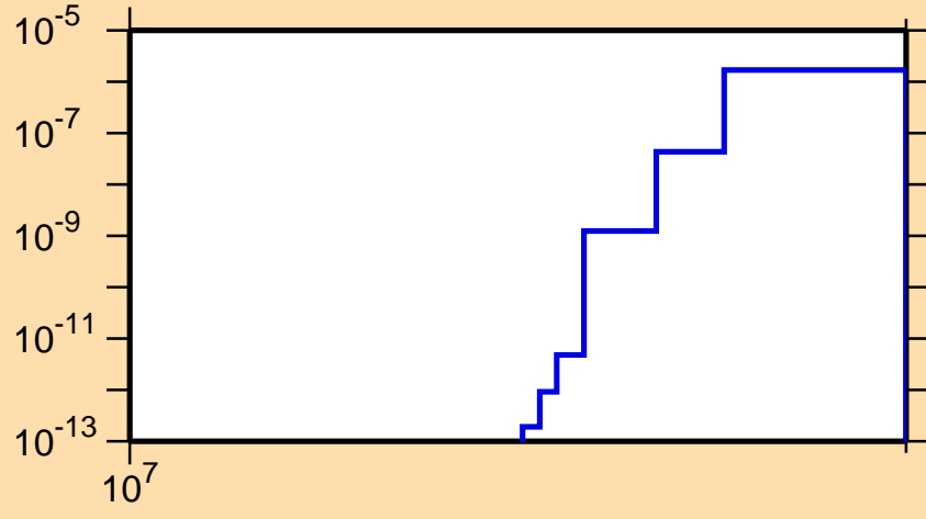
\sigma vs. E for ^{223}\text{Fr}(n,2np)
