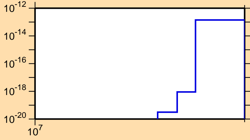
\sigma vs. E for ^{223}\text{Fr} (mt 42)
