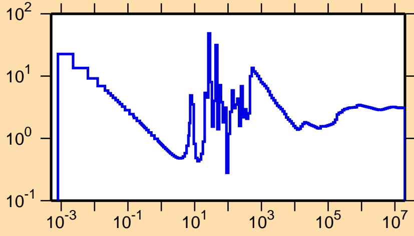
\sigma vs. E for ^{223}\text{Fr}(n,\text{nonel.})
