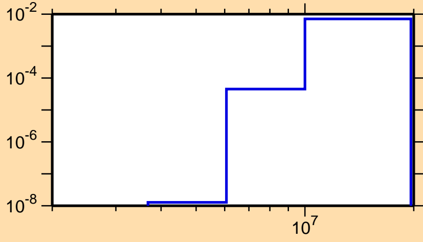
\sigma vs. E for ^{223}\text{Fr}(n,p)
