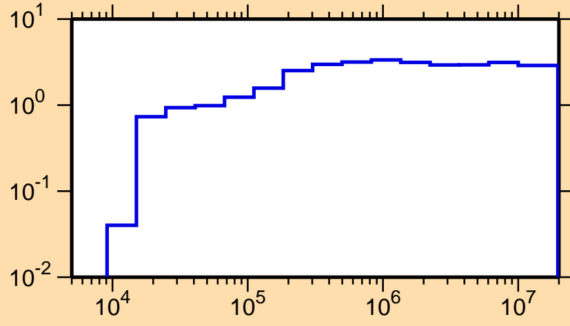
\sigma vs. E for ^{223}\text{Fr}(n,\text{inel.})
