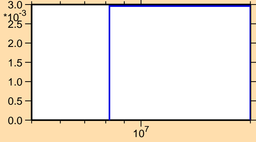
\sigma vs. E for ^{223}\text{Fr}(n,3n)
