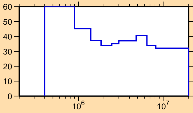
\Delta\sigma/\sigma vs. E for ^{223}\text{Fr}(n,\text{nonel.})
