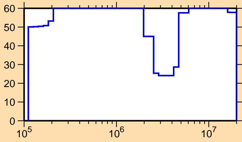
\Delta\sigma/\sigma vs. E for ^{224}\text{Fr}(n, el.)
