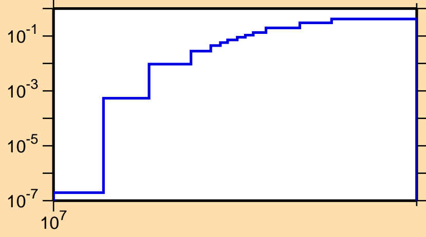
\sigma vs. E for ^{224}\text{Fr}(n,3n)
