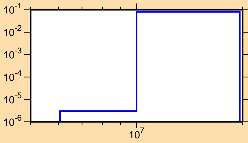
\sigma vs. E for ^{224}\text{Fr}(n,np)
