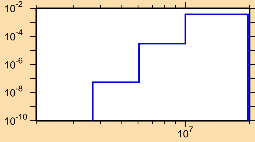
\sigma vs. E for ^{224}\text{Fr}(n,n\alpha)
