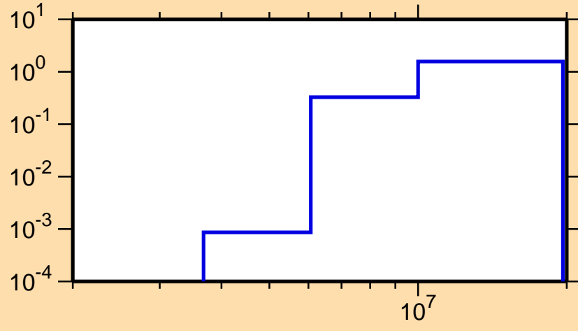
\sigma vs. E for ^{224}\text{Fr}(n,2n)
