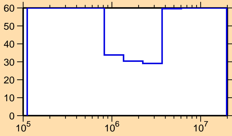
\Delta\sigma/\sigma vs. E for ^{224}\text{Fr}(n,\text{inel.})
