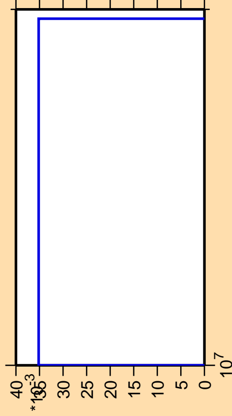
\Delta\sigma/\sigma vs. E for ^{224}\text{Fr}(n,p\alpha)
