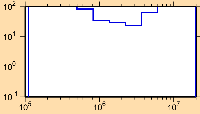
\Delta\sigma/\sigma vs. E for ^{224}\text{Fr}(n,ncont.)
