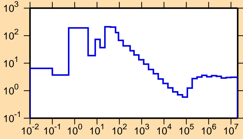
\sigma vs. E for ^{224}\text{Fr}(n,\text{nonel.})
