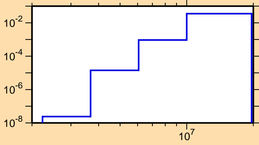
\sigma vs. E for ^{224}\text{Fr}(n,p)
