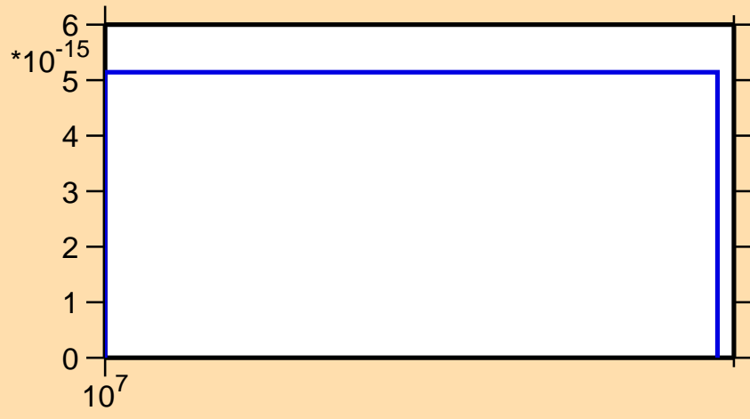
\sigma vs. E for ^{224}\text{Fr}(n,p\alpha)
