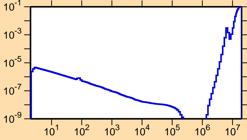
\sigma vs. E for ^{225}\text{Fr}(n,\alpha)
