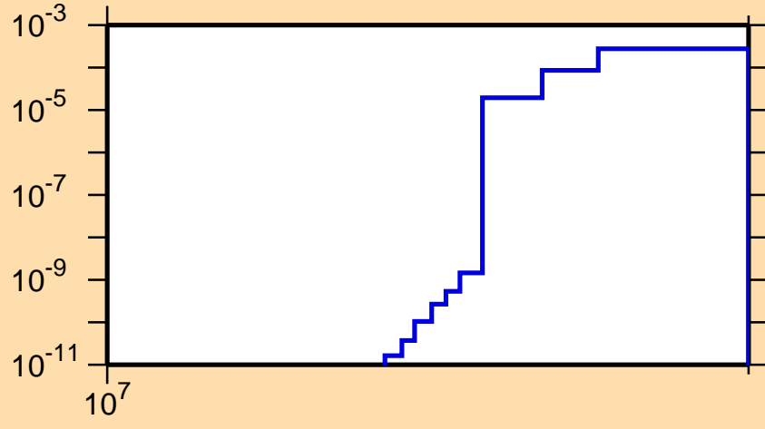
\sigma vs. E for ^{225}\text{Fr}(n,3n\alpha)
