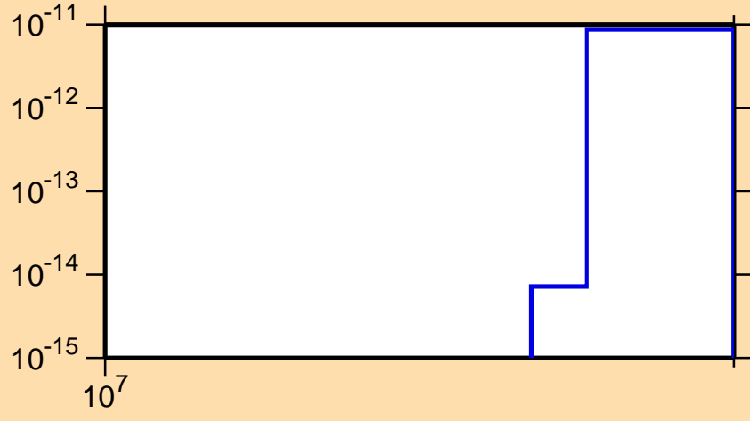
\sigma vs. E for ^{225}\text{Fr} (mt 11)
