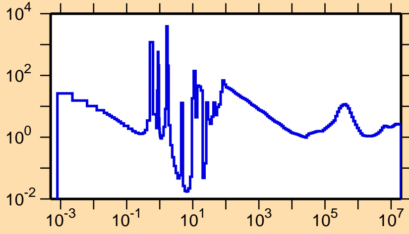
\sigma vs. E for ^{225}\text{Fr}(n,\text{nonel.})
