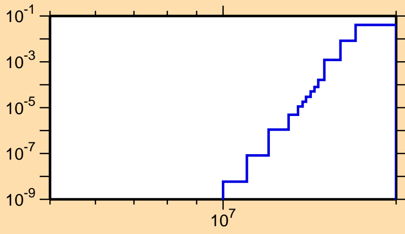
\sigma vs. E for ^{225}\text{Fr}(n,2n\alpha)
