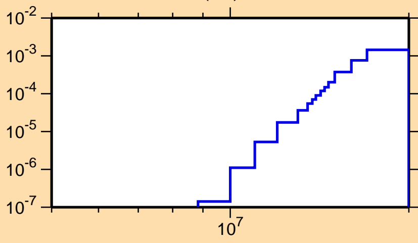
\sigma vs. E for ^{225}\text{Fr}(n,t)
