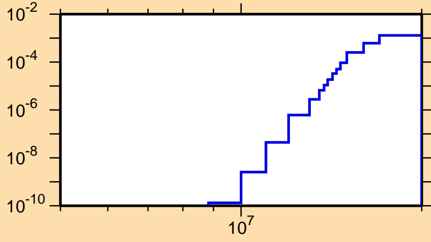
\sigma vs. E for ^{225}\text{Fr}(n,np)
