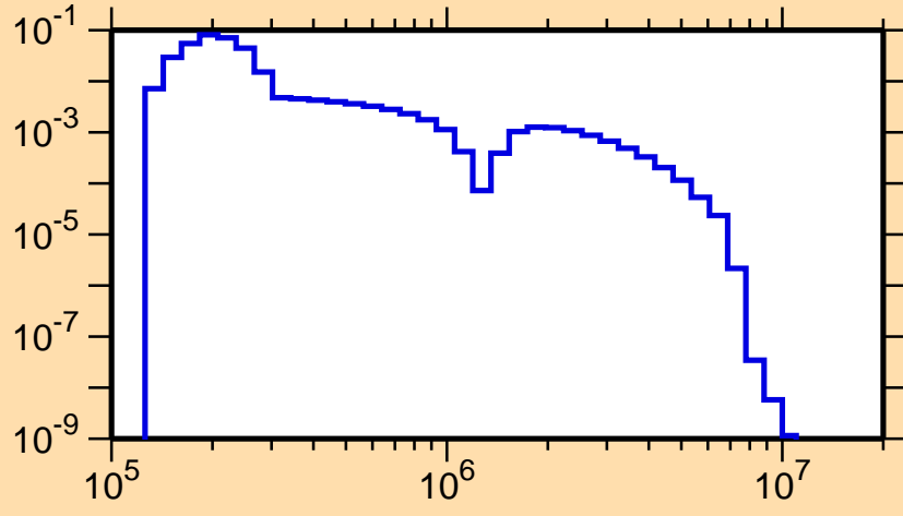
\sigma vs. E for ^{225}\text{Fr}(n,n_3)
