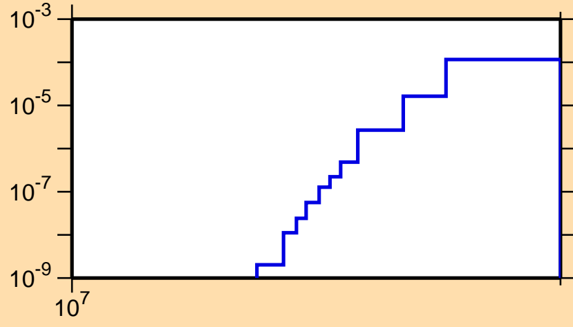
\sigma vs. E for ^{225}\text{Fr}(n,\text{nd})
