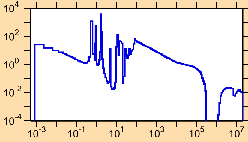
\sigma vs. E for ^{225}\text{Fr}(n,\gamma)
