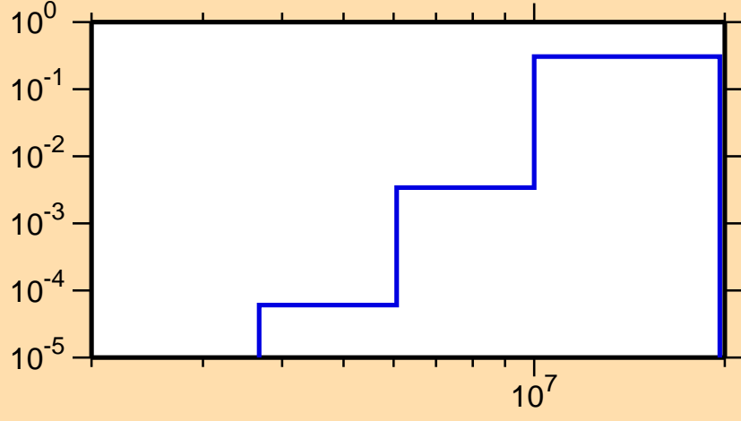
\sigma vs. E for ^{225}\text{Fr}(n,p)
