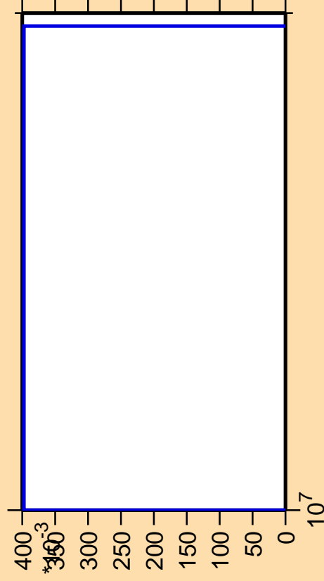
\Delta\sigma/\sigma vs. E for ^{225}\text{Fr} (mt 11)
