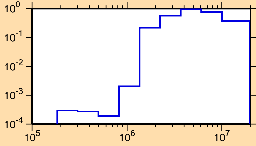
\sigma vs. E for ^{225}\text{Fr}(n,n\text{cont.})
